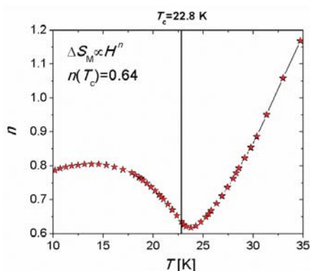
Figure 12. Temperature dependence of exponent n for 2 .
