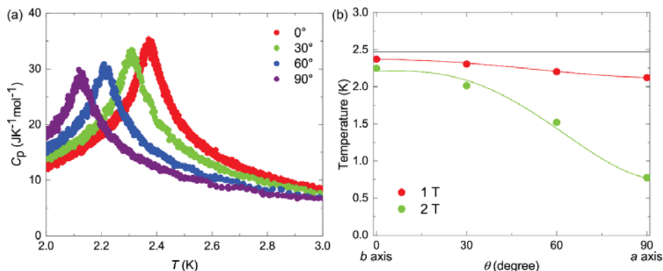
Figure 4. (a) Temperature dependences of the heat capacity of \kappa -(BETS) 2 FeBr 4 . The magnetic field of 1 T is applied in several directions from the b axis (0°) to the a axis (90°). (b) Field-direction dependence of the antiferromagnetic transition temperature at 1 T (red) and 2 T (green). The black line represents the antiferromagnetic transition temperature of 2.47 K at 0 T.
