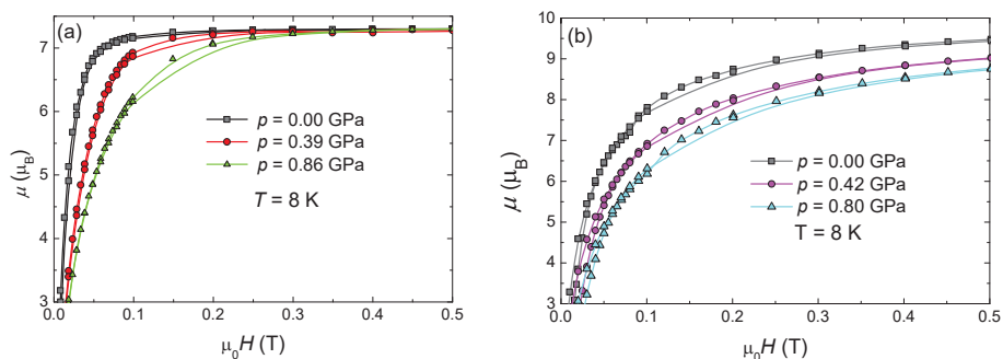
Figure 8. Effect of pressure on magnetic isotherms for (a) Mn 3 [Cr(CN) 6 ] 2 ·15H 2 O and (b) for Ni 3 [Cr(CN) 6 ] 2 ·15H 2 O.
