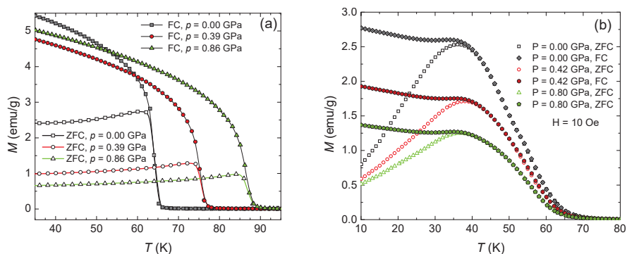
Figure 9. Effect of pressure on magnetization for (a) Mn 2+ -Cr III -PBs and (b) Ni 2+ -Cr III -PBs.
