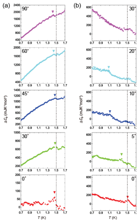
Figure 9. Field-direction dependences of the \Delta C_p vs. T curves of \kappa -(BETS) _2 FeBr _4 under the in-plane magnetic field at (a) 1 T and (b) 2 T. 0° and 90° correspond to the c axis and the a axis, respectively. Dashed lines represent the superconducting transition temperature of 1.5 K at 0 T. Reproduced with permission from [60].
