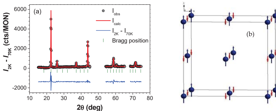
Figure 5. (a) Results of Rietveld refinement of data taken on Mn_3[Cr(CN)_6] \cdot zD_2O . (b) Simple model of ferrimagnetic structure of Mn_3[Cr(CN)_6] \cdot zD_2O , Mn (4a) (0,0,0): blue; Cr (4b) ( \frac{1}{2}, \frac{1}{2}, \frac{1}{2} ): red; \mu_{Mn} = 3.790 \mu_B a \mu_{Cr} = -1.375 \mu_B .
