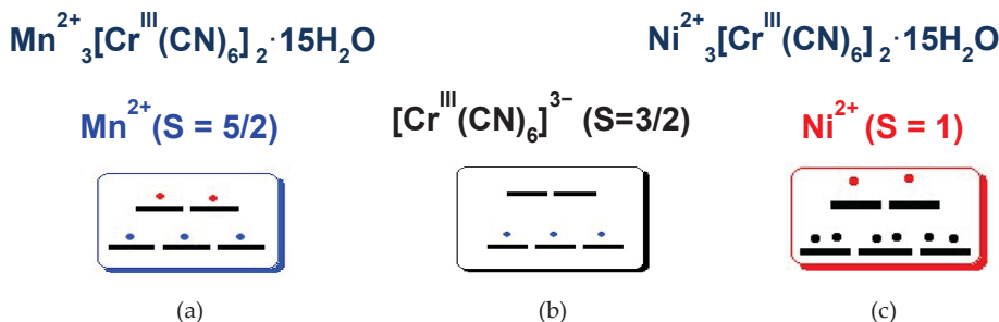
Figure 6. (a) There are six F and nine AF pathways with (t_{2g})^3(e_g)^2 orbitals of Mn^{2+} leading to overall J_{AF} in interaction; (b) Cr^{III} in anion [Cr^{III}(CN)_6]^{3-} is low spin and has only (t_{2g})^3 orbitals; (c) there are six F pathways with (e_g)^2 orbitals of Ni^{2+} leading to overall J_F interaction.
