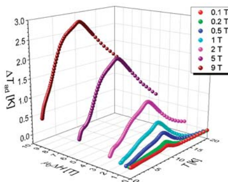
Figure 18. Temperature dependence of \Delta T_{\text{ad}} for 3 .
