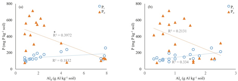
Figure 2. Correlations of contents of \text{P}_i and \text{P}_o with \text{Al}_d (a) and \text{Al}_o (b) in the pedon samples collected from the three sampling sites. * Statistically significant at p < 0.05 .
