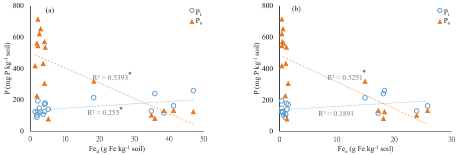
Figure 1. Correlations of contents of \text{P}_i and \text{P}_o with \text{Fe}_d (a) and \text{Fe}_o (b) in the pedon samples collected from the three sampling sites. * Statistically significant at p < 0.05 .
