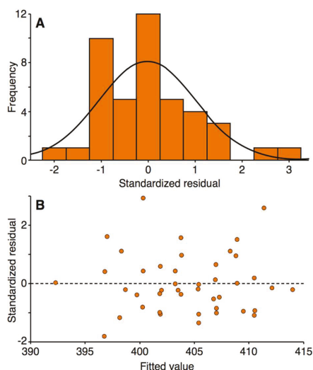
Figure 2. Frequency distribution graph of the standardized residuals (A) and a scatter plot of the standardized residuals versus the fitted values (B).
