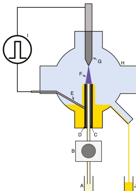
Figure 1. The scheme of the pulse-modulated radio-frequency atmospheric-pressure glow discharge (pm-rf-APGD)-based plasma-reaction system for the continuous production of silver nanoparticles (AgNPs). (A) Solution containing the AgNP precursor with or without pectin; (B) peristaltic pump; (C) quartz capillary; (D) graphite tube; (E) platinum wire; (F) pm-rf-APGD; (G) pin-type electrode; (H) quartz chamber; (I) radio-frequency (rf) voltage; (J) solution after pm-rf-APGD treatment containing AgNPs.
