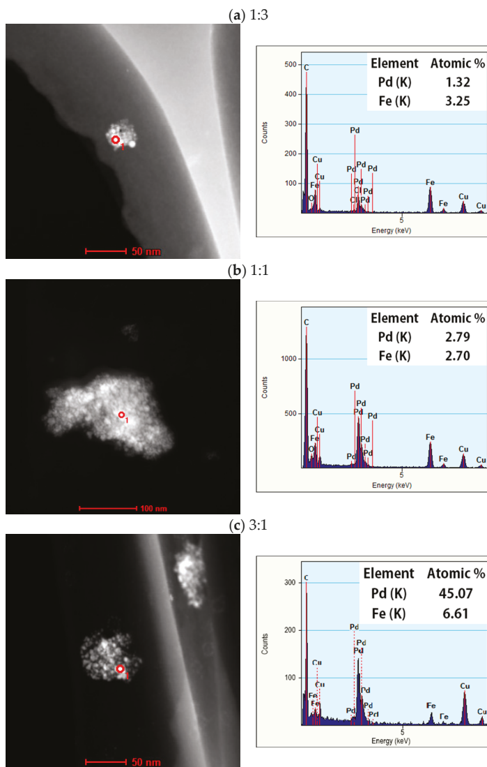
Figure 7. HAADF-STEM image and EDX analysis of upper 1:3 (a); 1:1 (b); and 3:1 (c) Pd-Fe alloy nanoparticles.
