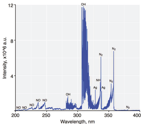
Figure 6. The optical emission spectrometry (OES) spectrum of pulse-modulated radio-frequency atmospheric-pressure glow discharge (pm-rf-APGD) generated under optimal operating conditions in the spectral range from 200 to 400 nm.
