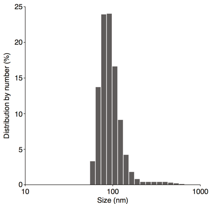
Figure 5. A histogram displaying size by number distribution of PVP-PtNPs as determined by DLS.
