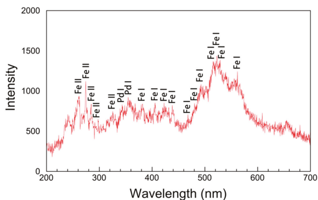
Figure 11. Optical emission spectrum from pulsed plasma in ethanol solution with Pd-Fe electrodes.
