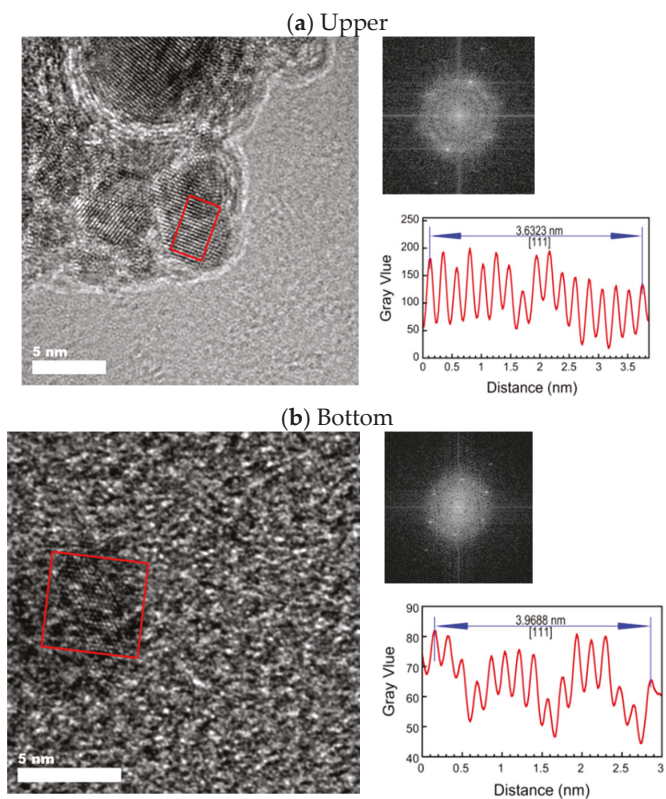
Figure 6. HR-TEM images of upper (a) and bottom (b) 1:1 Pd-Fe alloy nanoparticles with FFT pattern and surface spacing in the region enclosed in red.
