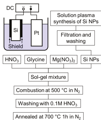
Figure 1. (Color online) Experimental setup for producing Si particles and schematic diagram for the solution combustion synthesis of Si-C the composite.
