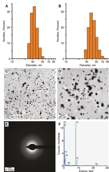
Figure 7. The morphology of silver nanoparticles (AgNPs) produced under optimal conditions. The histograms of size distribution by number of (A) purified AgNPs, and (B) non-purified AgNPs. (C,D) Representative transmission electron microscopy (TEM) micrographs of non-purified AgNPs, (E) the selected-area electron diffraction (SAED) pattern, and (F) the energy-dispersive X-ray spectroscopy (EDS) spectrum with prominent peaks labeled.
