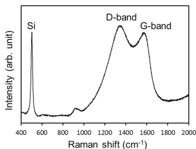
Figure 6. Raman spectrum of the Si-C composite prepared from Si-NPs generated in LiCl + H 3 BO 3 solution.
