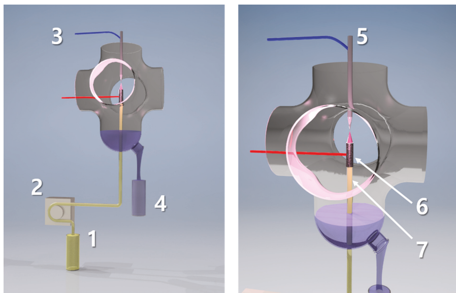
Figure 1. A continuous-flow reaction-discharge system for synthesis of poly(vinylpyrrolidone)-stabilized Pt nanoparticles (PVP-PtNPs); (1) the mixed working solution containing the PtNPs precursor and the PVP capping agent (FLA), (2) a four-channel peristaltic pump, (3) high-voltage wires, (4) a collector for the direct current atmospheric pressure glow discharge (dc-APGD)-treated solution, (5) a tungsten cathode, (6) graphite, and (7) quartz tubes.
