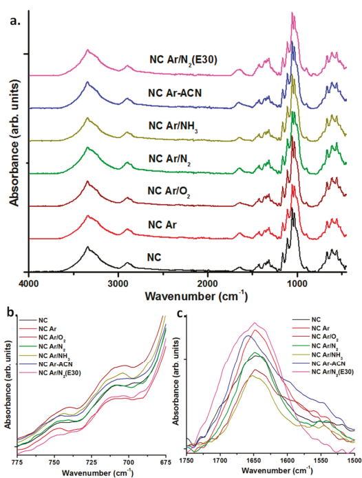
Figure 7. Fourier transform infrared spectroscopy (FTIR) spectra of untreated and plasma treated NC (a); zoomed-in regions (775–675 \text{cm}^{-1} ) (b) and (1750–1500 \text{cm}^{-1} ) (c) of the same spectra.
