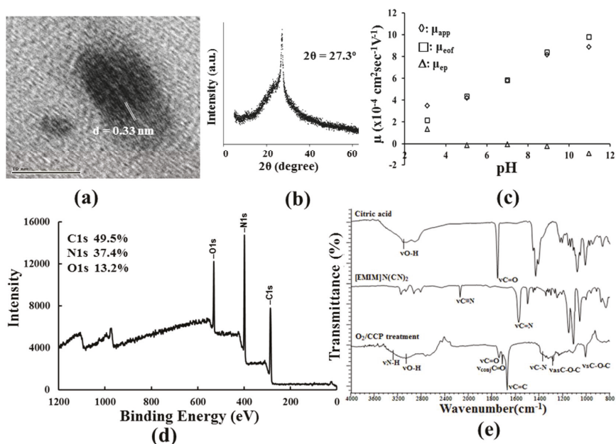
Figure 2. Characterization of the C-dots prepared in the conditions of Figure 1a. (a) HRTEM image; (b) XRD spectrum; (c) the plot of mobility with the pH of the running buffers; (d) XPS spectrum, and (e) FTIR spectrum.
