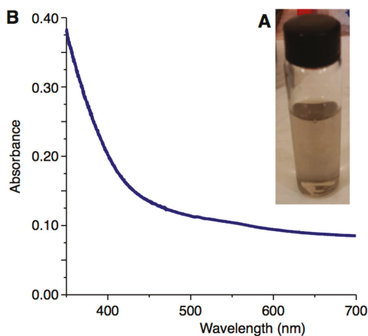
Figure 3. dc-APGD-mediated synthesis of PVP-PtNPs. (A) Color exhibited by the mixed working solution after dc-APGD treatment and related to production of PVP-PtNPs; (B) the UV/Vis spectrum of PVP-PtNPs.
