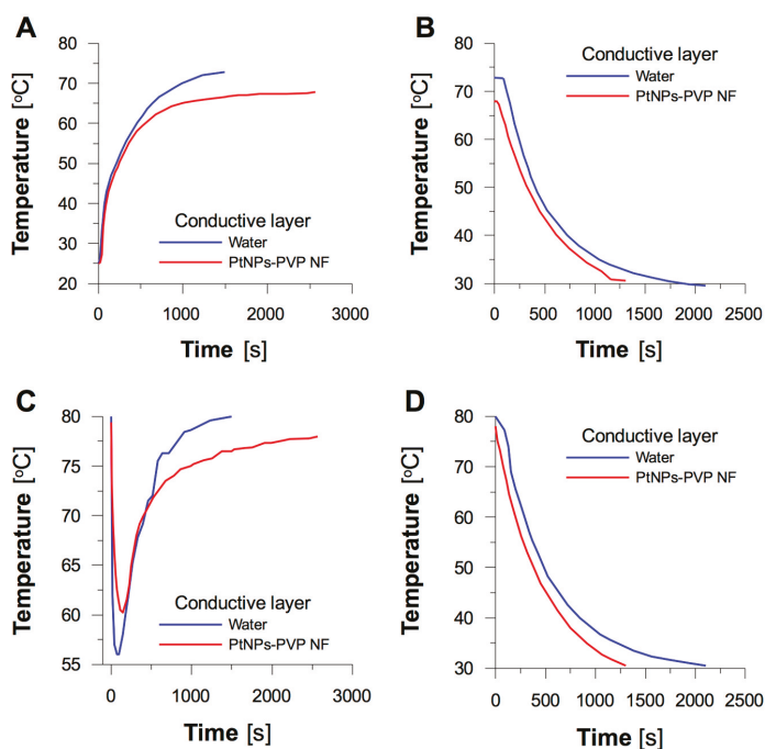
Figure 7. Time-dependent changes of temperature obtained for (A) heating, and (B) cooling of the conductive layer; (C) heating, and (D) cooling of the circulating liquid.
