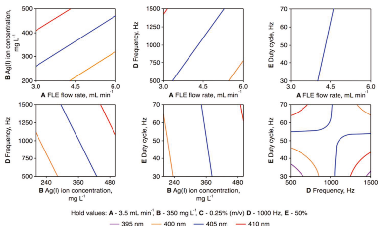
Figure 4. Counter plots of the wavelength at maximum ( \lambda_{\max} ) of the localized surface plasmon resonance (LSPR) band of silver nanoparticles (AgNPs) synthesized using the pulse-modulated radio-frequency atmospheric-pressure glow discharge (pm-rf-APGD) system for pairs of statistically significant parameters in the developed response surface regression model (A–B, A–D, A–E, B–D, B–E, and D–E) at defined hold values. A: the flow rate of the flowing liquid electrode (FLE) solution (mL·min -1 ); B: the precursor concentration in the FLE solution (mg·L -1 ); D: the frequency of pulse modulation of rf current (Hz); E: the duty cycle (%).
