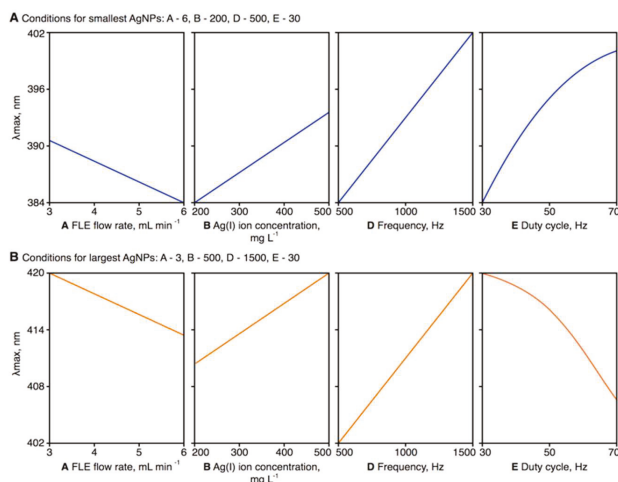
Figure 3. Graphical representation of the effects of the statistically significant parameters included in the response surface regression model on the wavelength at maximum ( \lambda_{\max} ) of the localized surface plasmon resonance (LSPR) absorption band of the synthesized silver nanoparticles (AgNPs). Graphs demonstrate the effects of modifying variables when the operating conditions were otherwise optimal for the production of spherical AgNPs with the lowest (A) and highest (B) \lambda_{\max} . A: the flow rate of the flowing liquid electrode (FLE) solution ( \text{mL}\cdot\text{min}^{-1} ); B: the precursor concentration in the FLE solution ( \text{mg}\cdot\text{L}^{-1} ); D: the frequency of pulse modulation of radio-frequency (rf) current (Hz); E: the duty cycle (%).
