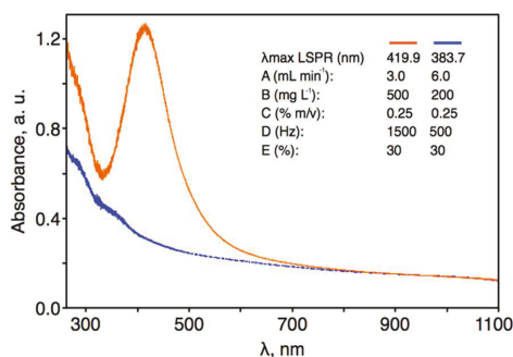
Figure 5. UV/Vis absorption spectra of silver nanoparticles (AgNPs) synthesized with the aid of the pulse-modulated radio-frequency atmospheric-pressure glow discharge (pm-rf-APGD) plasma-reaction under experimental conditions providing the smallest (condition 1) and the largest (condition 2) AgNPs according to the developed response surface regression model.
