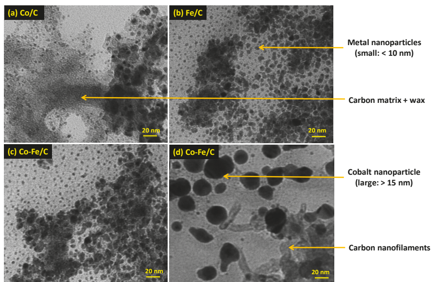
Figure 12. The TEM images of the used (a) Co/C (b) Fe/C and (c) Co-Fe/C catalysts with some sections having nanoparticles predominantly below ~5 nm, or ~10 nm, and (d) sections of the Co-Fe/C catalyst with larger nanoparticles ~20 nm and CNFs.
