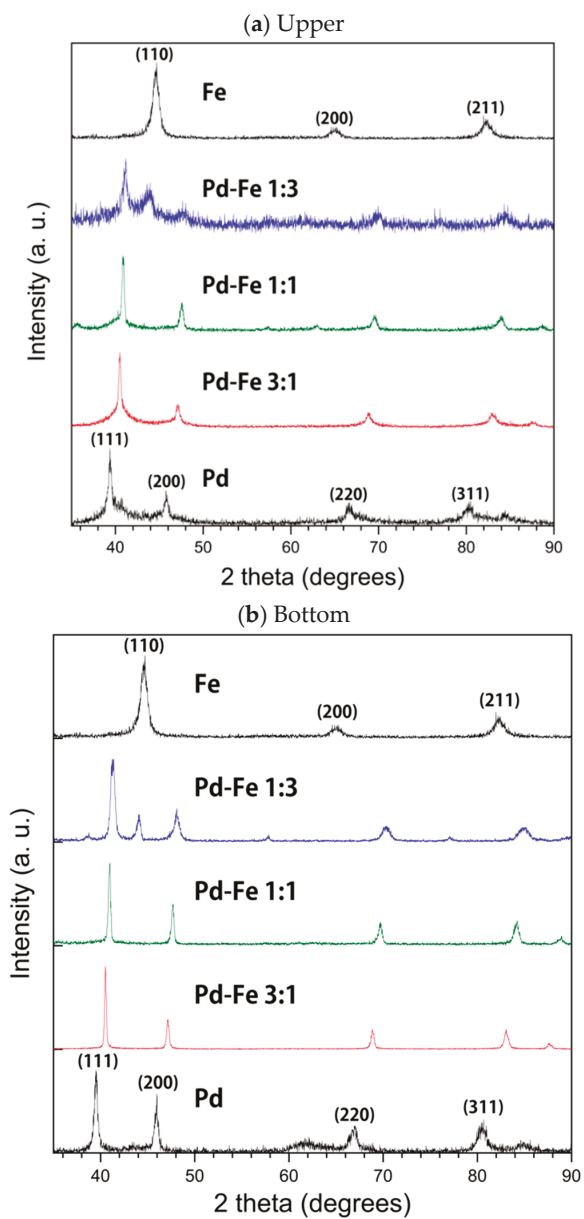
Figure 3. XRD patterns of Pd-Fe alloy nanoparticles and of elemental Pd and Fe nanoparticles in upper (a) and bottom (b) samples.
