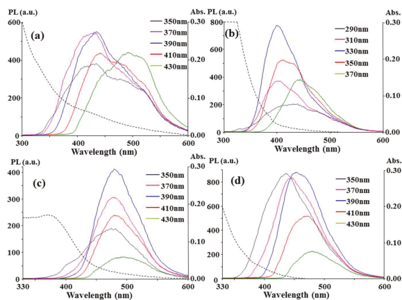
Figure 4. Fluorescence and UV-Vis absorption spectra for the CA + [EMIM]N(CN) 2 (a,c) and [EMIM]N(CN) 2 alone (b,d) samples heated in a 90 W microwave oven for 4.5 min (a,b) and in an autoclave at 200 °C for 30 min (c) and 5.0 h (d). After the addition of 1.0 mL of H 2 O to the heated products, the product solutions of 0.2 μL for (a); 0.3 μL for (b); 2.0 μL for (c); and 15 μL for (d) were diluted with 3.0 mL of H 2 O to measure the spectra.
