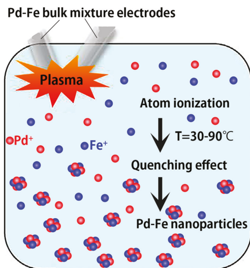
Figure 12. Illustration of Pd-Fe alloy nanoparticle formation via pulsed plasma in water.
