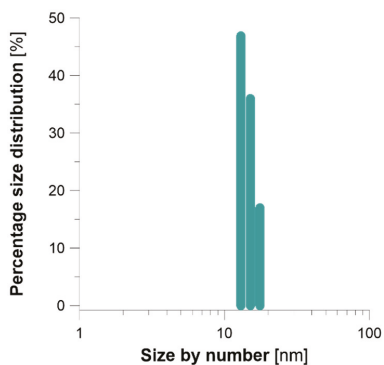
Figure 5. Percentage size distribution by the number of FRU-AgNPs estimated by dynamic light scattering (DLS).
