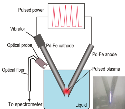
Figure 1. Schematic of pulsed-plasma-in-liquid method.
