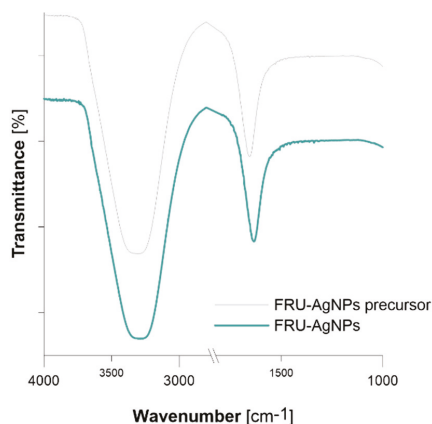
Figure 6. ATR FT-IR spectra of the working solution before (FRU-AgNPs precursor) and after (FRU-AgNPs) dc-APGD treatment.
