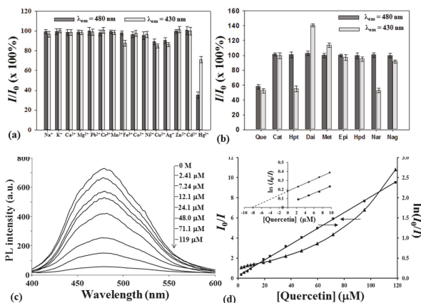
Figure 5. Effect of different metal ions (33.3 \mu\text{M} ) (a) and flavonoids (8.33 \mu\text{g/mL} ) (b) on the relative PL intensity ( I/I_0 ) of the C-dots prepared in the conditions of Figure 1a; (c): Emission spectra of the prepared C-dots before and after the addition of various concentrations of quercetin; (d): The respective emission intensities are plotted versus the quercetin concentrations according to the Stern–Volmer ( \blacktriangle ) and Perrin ( \blacksquare ) models. The curve of the standard addition calibration ( \blacklozenge ) for the determination of quercetin in the ethanol extract of Guang-Chen-Pi is inserted in (d). I and I_0 are the PL intensities observed in the presence ( I ) and absence ( I_0 ), respectively, of the samples in a 50 mM phosphate buffer at pH 7.0.
