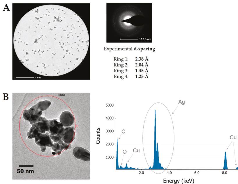
Figure 4. Granulometric properties of Ag nanostructures (A) The SAED pattern for the micrograph of FRU-AgNPs and (B) the EDX spectrum for the presented FRU-AgNPs.
