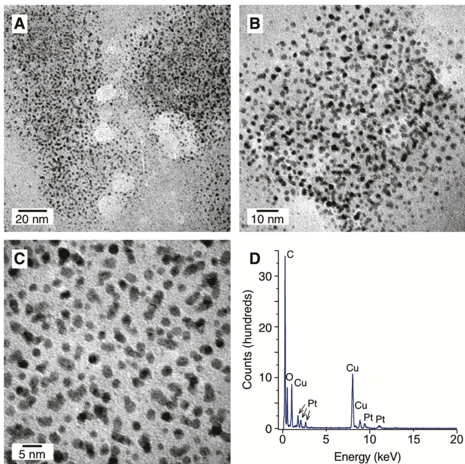
Figure 4. Granulometric properties of PVP-PtNPs synthesized with the aid of dc-APGD. (A–C) Representative TEM photomicrographs; (D) the EDX spectrum.
