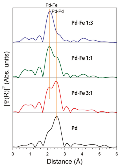
Figure 10. Fourier transforms of the Pd K-edge EXAFS oscillation function k^3\chi(k) . No phase shift corrections are made. The first sets of nearest peaks represent the Pd-Fe and Pd-Pd distances.
