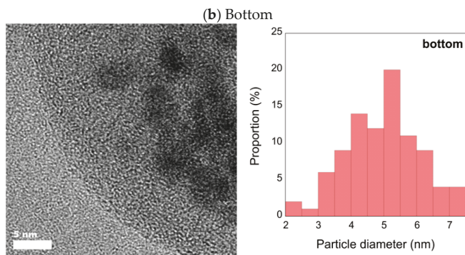
Figure 5. HR-TEM images of upper (a) and bottom (b) 1:1 Pd-Fe sample with particle diameter distribution.
