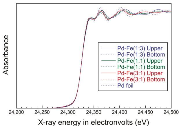
Figure 8. Normalized XANES of Pd parts of nanoparticles.
