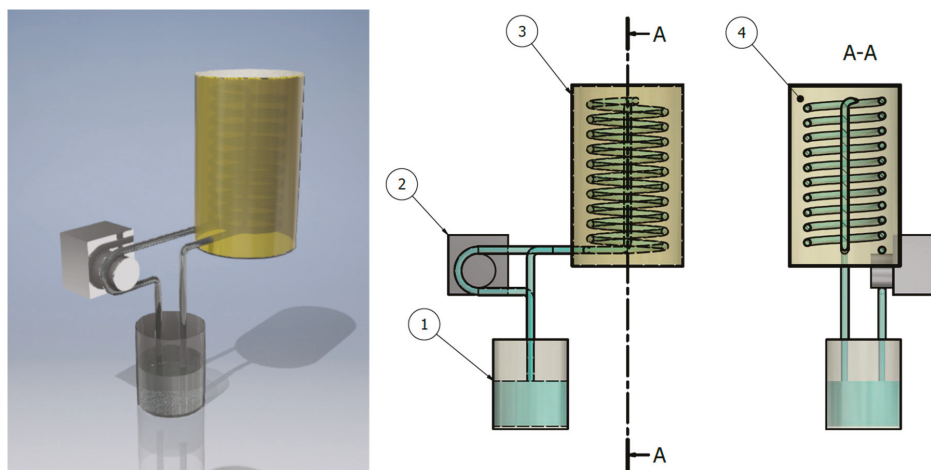
Figure 2. A 3D model of the heat management system (HMS) composed of (1) a cooling liquid reservoir, (2) a peristaltic pump, (3) a spiral radiator filled with (4) a conductive layer (the NF containing PVP-PtNPs or water).
