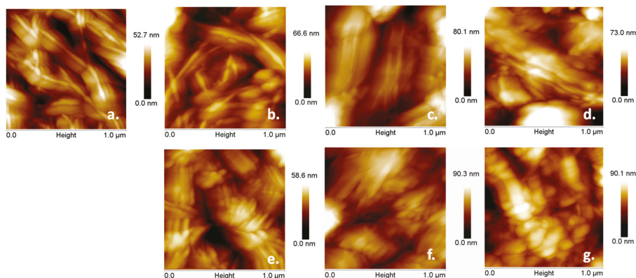
Figure 5. AFM topographic images of untreated (a) and plasma treated NC: Ar (b); Ar/O 2 (c); Ar/N 2 (d); Ar/N 2 (E30) (e); Ar/NH 3 (f); Ar-ACN (g).
