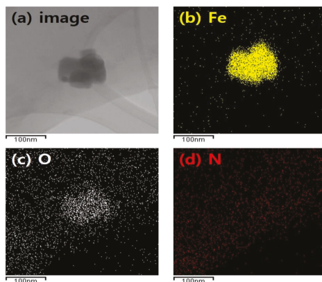
Figure 5. FE-TEM image and elemental mapped results of iron oxide nanoparticle on the IONCC-10; (a) TEM image; (b) iron; (c) oxygen; and (d) nitrogen element.
