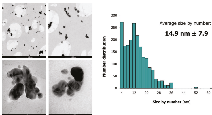
Figure 3. TEM micrographs illustrating shapes and size distribution of FRU-AgNPs.
