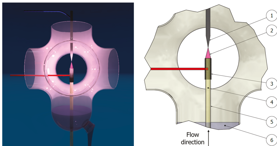
Figure 1. A schematic representation of the dc-APGD-based reaction-discharge system working in a continuous-flow mode. (1) A pin-type W cathode, (2) dc-APGD, (3) a graphite tube, (4) a working solution (with the AgNPs precursor and D-fructose) acting as a flowing liquid anode (FLA), (5) a quartz capillary, and (6) a compartment for the collection of the dc-APGD treated working solution containing the synthesized FRU-AgNPs.
