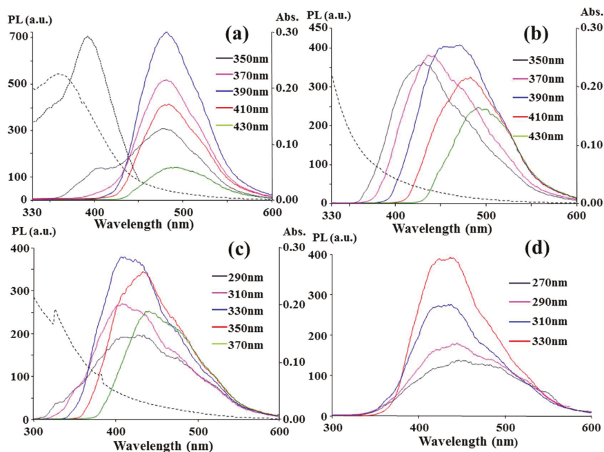
Figure 1. Fluorescence spectra of (a,d) CA + [EMIM]N(CN) 2 ; (b) [EMIM]N(CN) 2 ; and (c) CA + glycerol treated by O 2 /CCP (a,b,d) and N 2 /CCP (c). The mixtures of CA (100 mg) and solvents (500 \mu L) were treated by CCP (10 sccm of gas flow, RF power 90 W, 30 min). After the addition of 1.0 mL of H 2 O to the treated products, different volumes of the product solutions (0.2 \mu L for (a,d) and 20 \mu L for (b,c)) were separately transferred to cuvettes filled with 3.0 mL of H 2 O for spectrometric measurements. (—) and (---) curves denote UV-Vis absorption and PL (emission at 480 nm) spectra, respectively.
