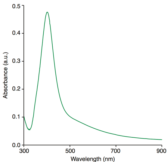
Figure 2. The UV/Vis absorption spectrum of five times diluted colloidal suspension of FRU-AgNPs.
