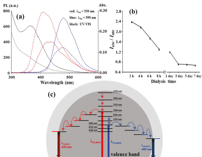
Figure 3. (a) Fluorescence and UV-Vis absorption spectra of the C-dots prepared in the conditions of Figure 1a before (solid lines) and after (dashed lines) dialysis in H 2 O by a 500–1000 Da cut-off membrane for two hours; (b) The plot of the PL intensity ratios of 430 nm PL intensity to 480 nm PL intensity with the dialysis duration; (c) The proposed PL mechanism.
