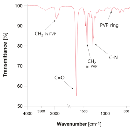
Figure 6. The ATR FT-IR spectrum of PVP-PtNPs.
