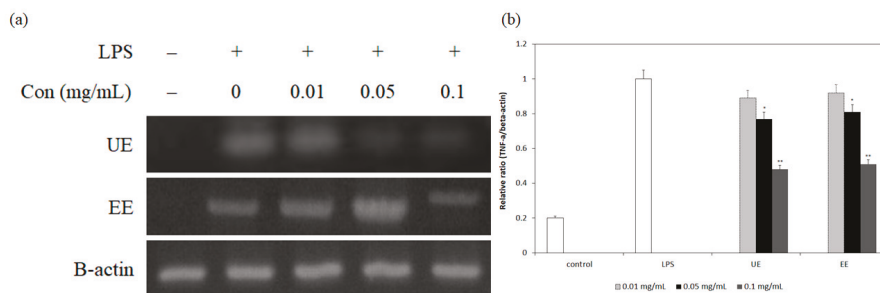
Figure 4. Down-regulation of mRNA expression of TNF-α from LPS-induced BV-2 cells (a) and the relative ratio of the gene expression by normalizing with beta-actin as a house-keeping gene (b) by the treatment of various concentrations of the Spirulina extracts along with the untreated control. EE, 70% ethanol extraction at 80 °C for 12 h, UE, ultrasonic pretreatment with 70% ethanol at 40 kHz and room temperature for 8 h, and further extraction at 65 °C for 4 h. Values are presented as means ±SD; * p < 0.05 and ** p < 0.01 compared with the LPS group.
