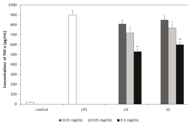
Figure 5. The secretion of TNF-α from LPS-induced BV-2 cells by the treatment of various concentrations of the Spirulina extracts. EE, 70% ethanol extraction at 80 °C for 12 h, UE, ultrasonic pretreatment with 70% ethanol at 40 kHz and room temperature for 8 h, and further extraction at 65 °C for 4 h. Values are presented as means ±SD; * p < 0.05 and ** p < 0.01 compared with the LPS group.
