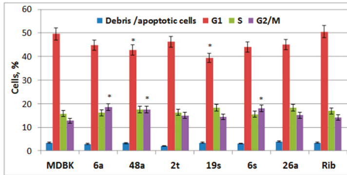
Figure 2. Influence of the EPSs on the cell cycle of the MDBK cells. (A) Cell cycle profiles of the control cells and EPS-treated cells (concentration of exopolysaccharides and ribavirin are 1500 and 125 µg/mL, respectively). (B) Cell cycle features after treatment with the EPSs were measured by flow cytometry following cell fixation and propidium iodide staining. Cell cycle profiles were analyzed with the Flowing Software, version 2.5. Results corresponding to the percentage of cells in G1, S, and G2/M phases of three independent experiments are presented as mean ± S.D. * Significant difference between test sample and control cells ( p < 0.05 ).
