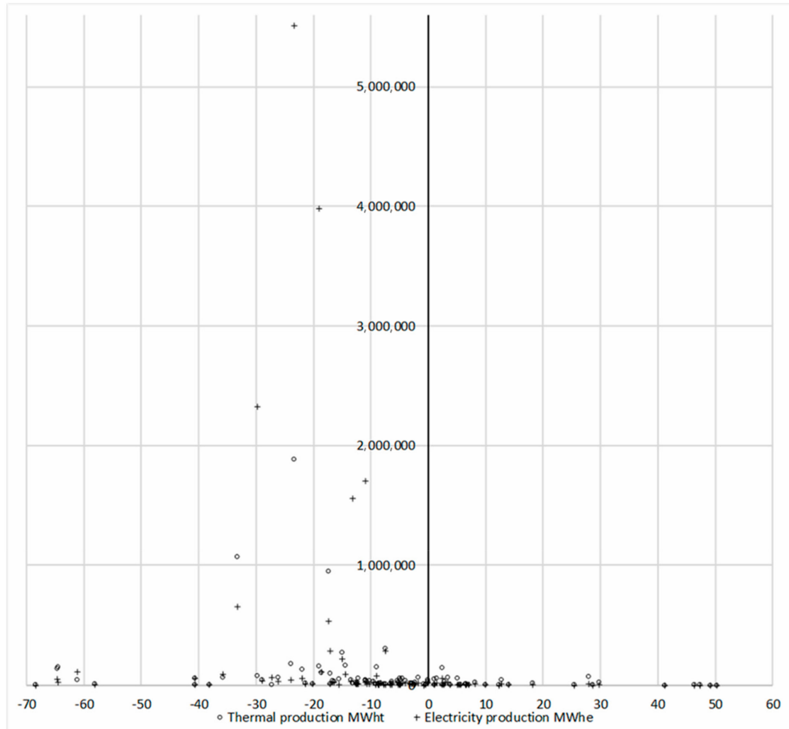
Figure A1. Avoided consumption of fossil fuels in district-heating systems using fossil sources, by the quantity of energy produced (MWht, MWh) [19].
