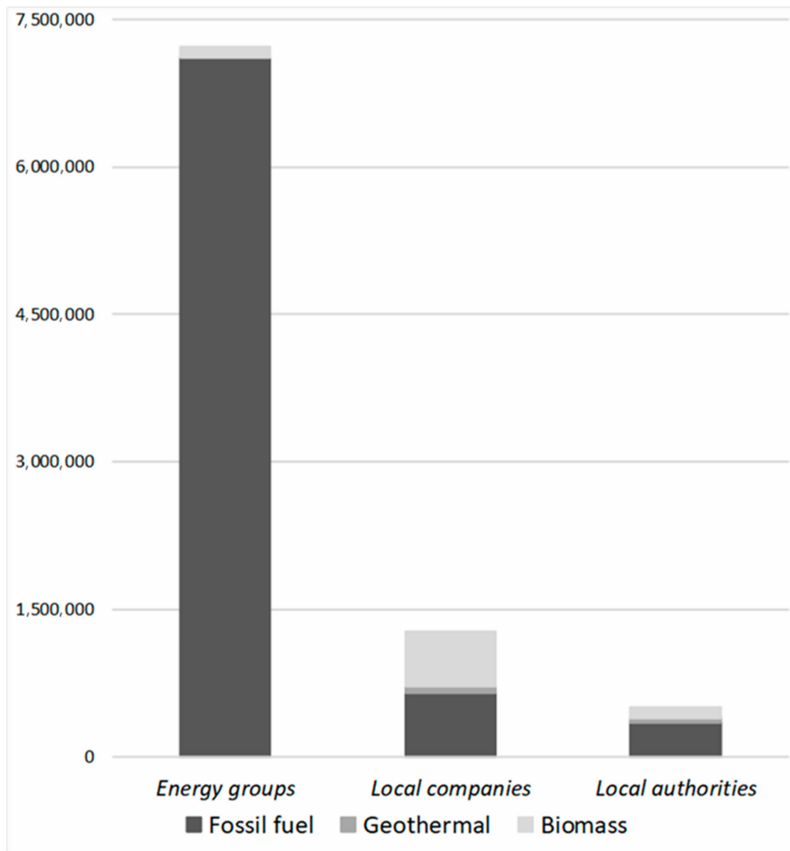
Figure A8. Thermal energy supplied (MWh/year) per ownership and energy source [19].
