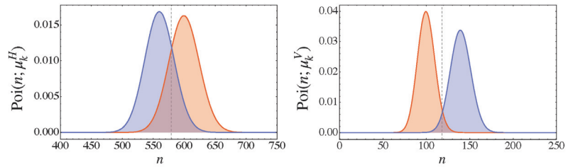
Figure 3. Probability density function of the Poissonian distribution in Equation (17) for the H detector (left plot) and the V detector (right plot) for \langle N_c \rangle = 500 , N_{dc} = 100 and m = 11 . The probability of error in Equations (25) and (29) are, respectively, p_e^V = 0.034 ( V detector) and p_e^H = 0.205 ( H detector). The gray dashed line is the threshold values in Equation (19). The values of the involved parameters have been chosen to better highlight the investigated effect.
