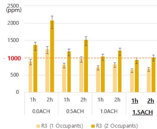
Figure 6. Calculated CO 2 concentration rates of (a) R1, (b) R2, and (c) R3, based on the experimental conditions with error ranges. * The bold text cases are analyzed by numerical calculations and error ranges without experiments in Table 2.
