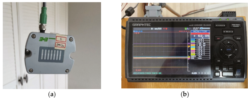
Figure 3. Equipment for experiments: (a) CO 2 Sensor; (b) data logger.
