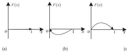
Figure 3. The evolutionary phase diagram of the central government’s strategy choices: (a) 0 < y = z_1 < 1, 0 < z = z_1 < 1, 0 < \theta = \theta_1 < 1 ; (b) 0 < y_1 < y < 1, 0 < z_1 < z < 1, 0 < \theta_1 < \theta < 1 ; (c) 0 < y < y_1 < 1, 0 < z < z_1 < 1, 0 < \theta < \theta_1 < 1 .
