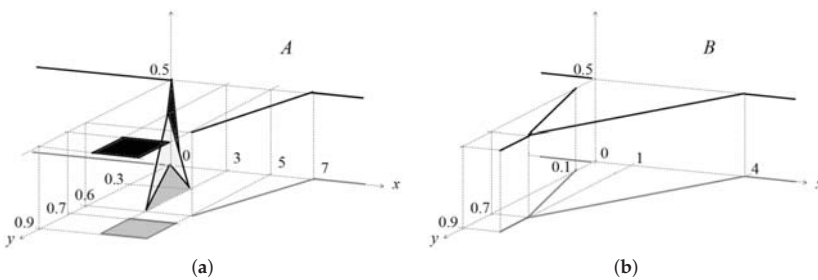
Figure 8. Membership functions of T2GFNs (a,b) given in Example 3.
