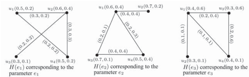
Figure 1. Intuitionistic fuzzy soft graph G = \{H(e_1), H(e_2), H(e_3)\} .
