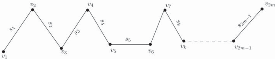
Figure 3. A path on 2n vertices.
