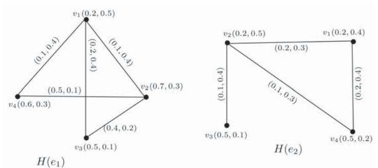
Figure 2. Intuitionistic fuzzy soft graph G = \{H(e_1), H(e_2)\} .
