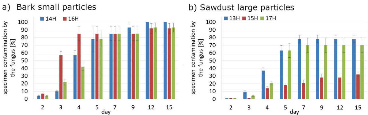
Figure 9. The rate of surface fouling by fungi Aspergillus niger Tiegh of HDPE composites with MAHPE addition; (a) bark small particles; (b) sawdust large particles.
