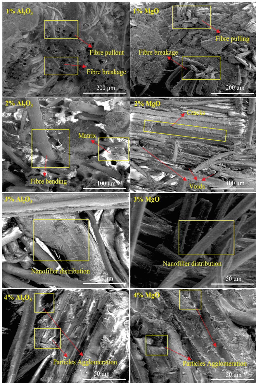
Figure 7. SEM images of alkali-treated biotex flax/PLA reinforced epoxy composite at different percentage of nano-Al 2 O 3 and nano-MgO.
