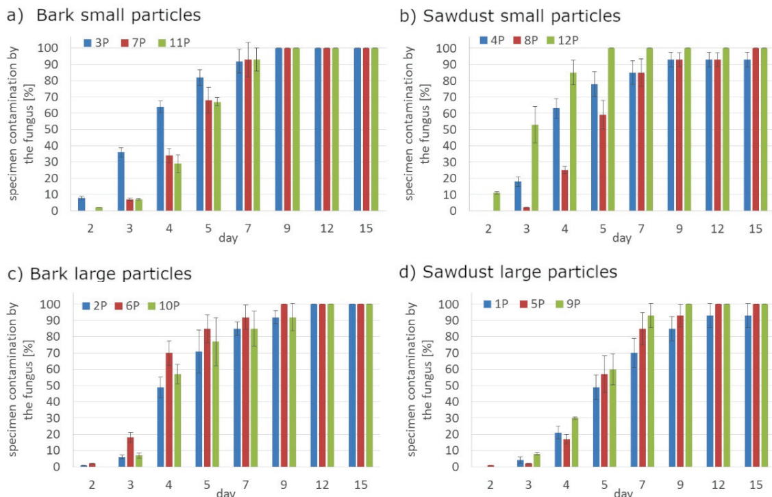
Figure 1. The rate of surface fouling by Aspergillus niger Tiegh fungi on PLA composites for: (a) bark small particles; (b) sawdust particles; (c) bark large particles; (d) sawdust large particles.
