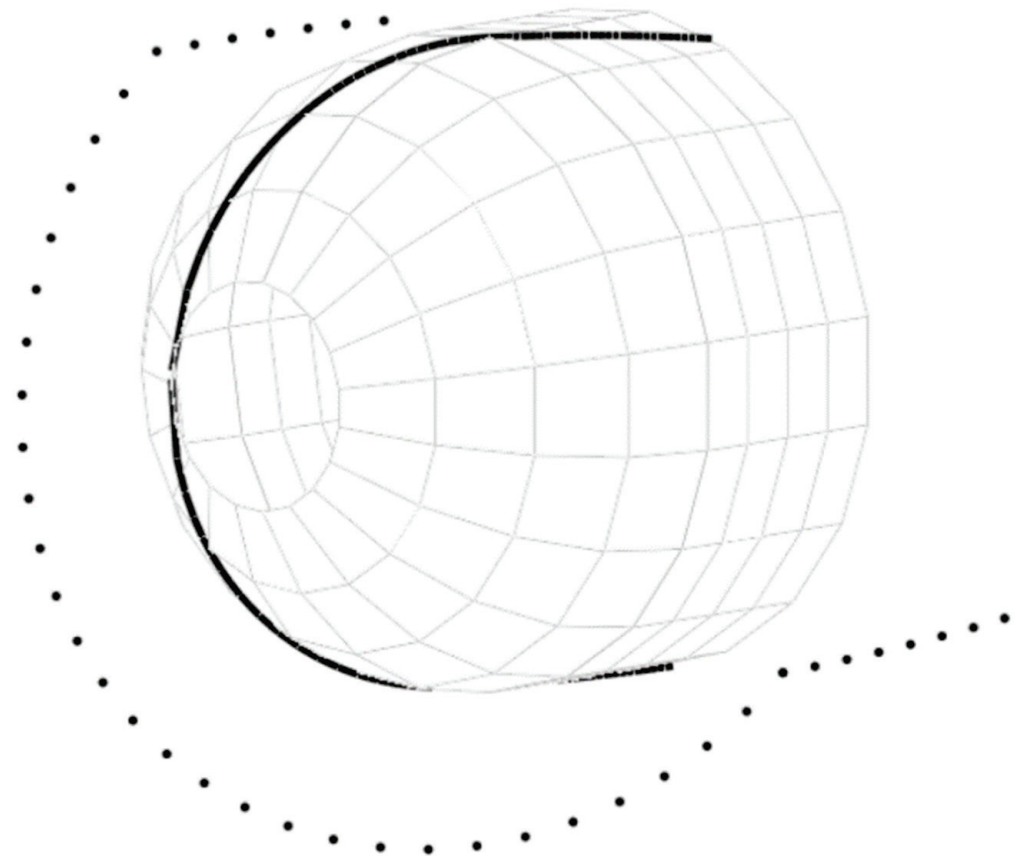
Figure 13. Calculated trajectories of the delivery eye and the tow depicted for half of the mandrel ( \lambda = \text{constant} ).
