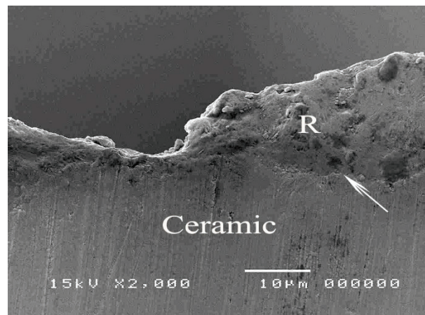
Figure 10. An SEM micrograph of the resin-ceramic interface using Super-Bond demonstrating the shallow irregularity on the ceramic surface of the fractured specimen (original 2000 ×, R = luting resin).
