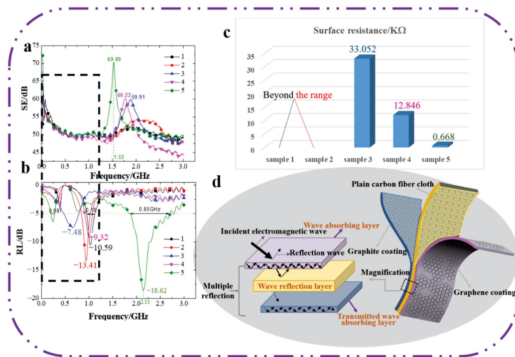
Figure 2. (a) The shielding properties of the composites. (b) The absorbing properties of the composites. (c) The conductive properties of the composites, (d) The structure model.
