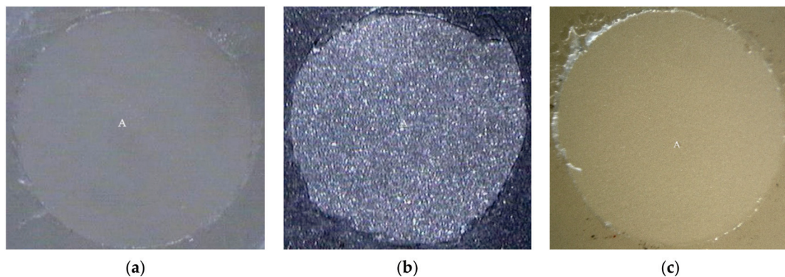
Figure 4. Adhesive failure on the prosthesis side interface (A) on fractured specimens of (a) ceramic, (b) metal alloy, and (c) resin composite using All-Bond2 + DuoLink (original 20×).
