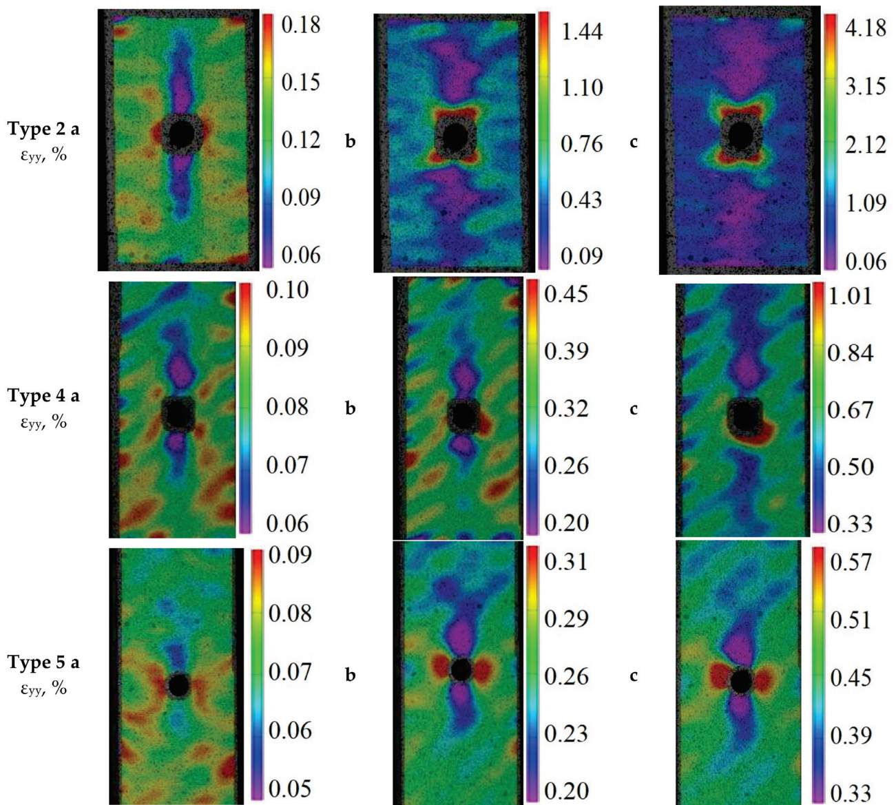
Figure 6. Fields of longitudinal strains \epsilon_{yy} of the surface of specimens of reinforcement types 2, 4, and 5 for a loading of 10% (a), 40% (b), and 70% (c) of the maximum value F^{OHTU} .
