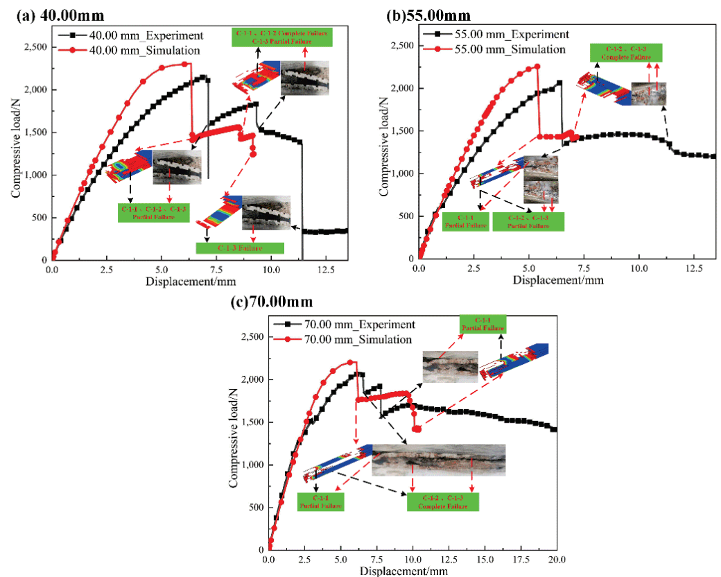
Figure 13. Load–displacement curves for L-joints with different bonding lengths: (a) 40.00 mm, (b) 55.00 mm and (c) 70.00 mm.
