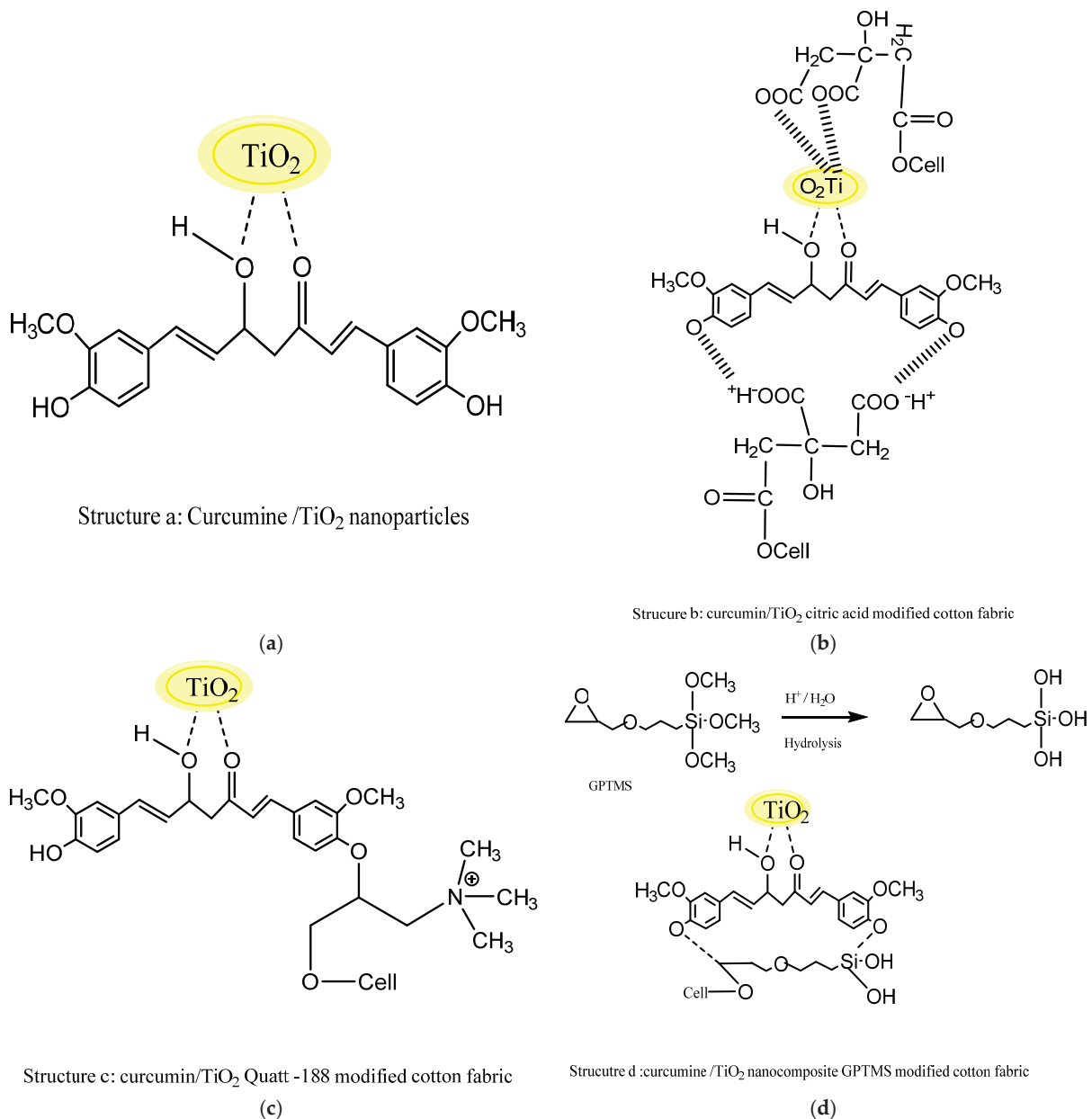
Figure 1. Schematic of the mechanism for the deposition of the curcumin/TiO 2 nanocomposite on cotton fabrics. (a) Structure a: curcumin/TiO 2 nanoparticles; (b) Structure b: curcumin TiO 2 : citric acid modified cotton fabric; (c) Structure c: curcumin/TiO 2 , Quatt-188 modified cotton fabric; (d) Structure d: curcumin/TiO 2 , nanocomposite GPTMS modified cotton fabric.
