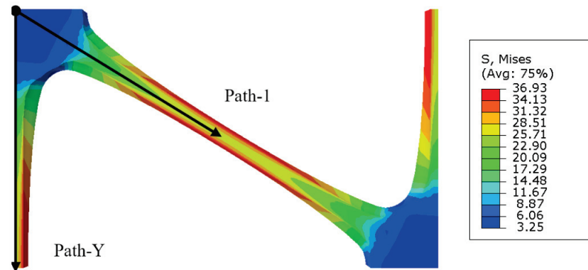
Figure 16. Cross section of the thick symmetry axis and path definition of triaxial geogrid.
