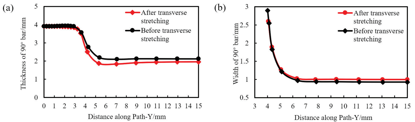
Figure 17. Thickness and width of the 90° rib before and after transverse stretching. (a) Thickness, (b) width.
