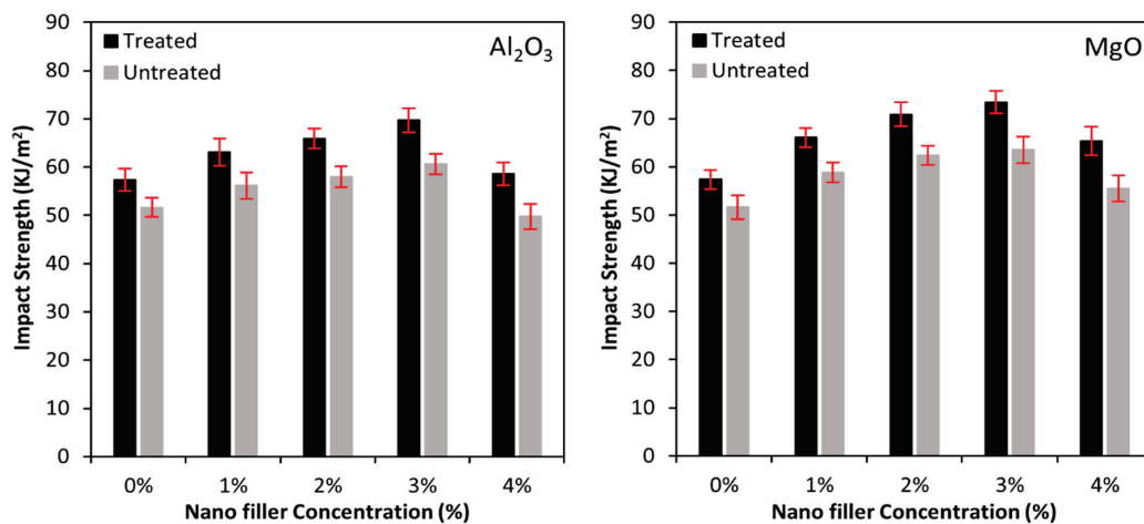
Figure 5. Impact strength of nano Al 2 O 3 and MgO incorporated biotex flax/PLA epoxy hybrid composites.
