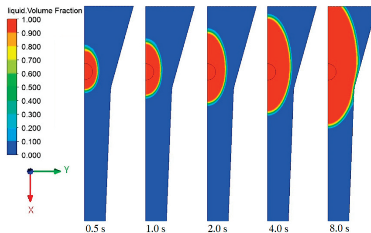
Figure 5. Resin flow distribution in the impregnation box at different times.
