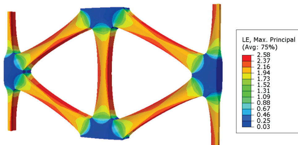
Figure 19. Simulation result of a triaxial geogrid with a pre-punched diameter of 2.6 mm.
