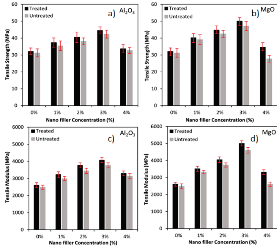
Figure 1. (a) Tensile strength of nano Al 2 O 3 , (b) Tensile strength of MgO, (c) Tensile modulus of nano Al 2 O 3 , (d) Tensile modulus of MgO incorporated flax/PLA epoxy hybrid composites.
