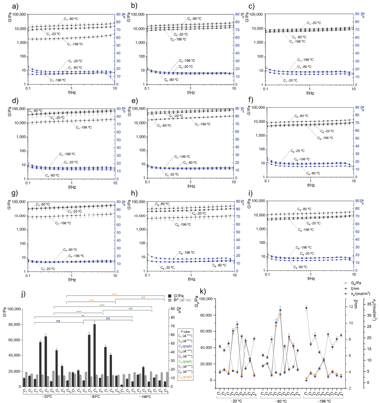
Figure 3. Oscillatory rheological behavior of different marine origin cryogels (a–i) corresponded to the developed cryogels C 1 to C 9 , respectively, produced at −20, −80 and −196 °C. Data show the mean of three values from independent experiments and the standard error for G'/\text{Pa} (black lines) and the phase angle \delta/^\circ (blue lines). (j) Comparison of each marine cryogel as a function of G'/\text{Pa} and the \delta/^\circ , with the average stable zone between 0.5 to 5 Hz. All differences between samples were statistically significant **** p < 0.0001 except those represented with the symbols of ** ( p < 0.01 ) and ns (not significant). (k) Comparative analysis of the storage modulus at the plateau ( G_e/\text{Pa} ), mesh size ( \xi/\text{nm} ), and the crosslinking density ( n_e/\text{mol}/\text{m}^3 ) of the developed marine cryogels.
