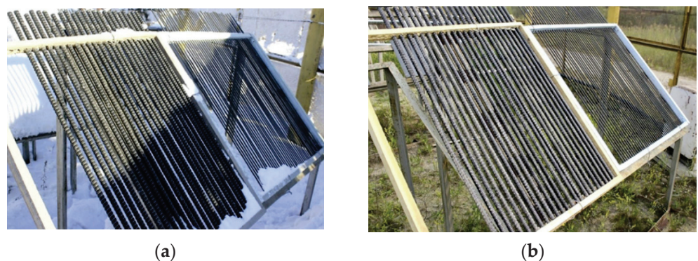
Figure 2. Open stands with BFRP rebar in Yakutsk in winter (a), and in summer (b).
