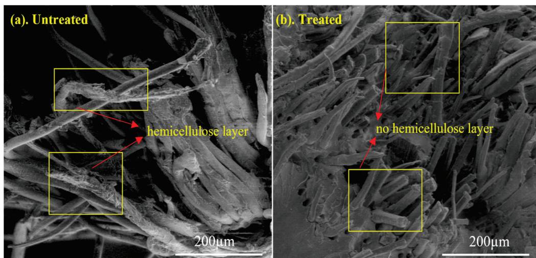
Figure 6. SEM images of tensile fractured (a) Untreated (b) alkali-treated biotex Flax/PLA reinforced epoxy composite.
