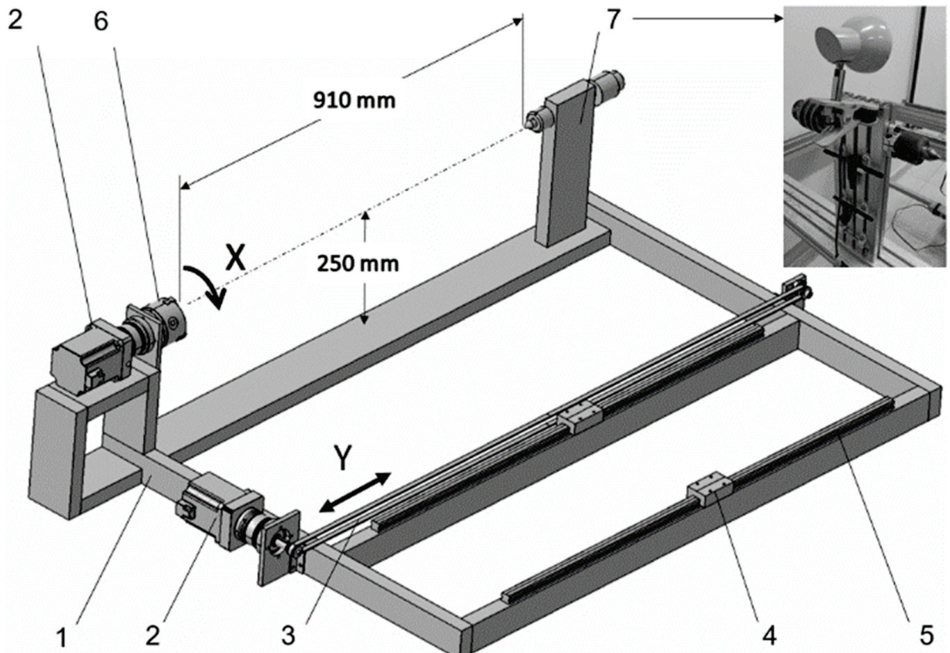
Figure 7. Assembly components of the filament winder frame (sensors are not shown): 1—aluminum V-slot profile; 2—stepper motor with planetary reduction drive; 3—timing belt; 4—slider block; 5—linear guide rail; 6—lathe chuck; 7—tailstock with tool set.
