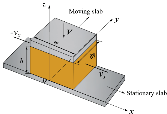
Figure 7. The rectangular coordinate systems used in the theoretical analysis, dy = \Delta l .
