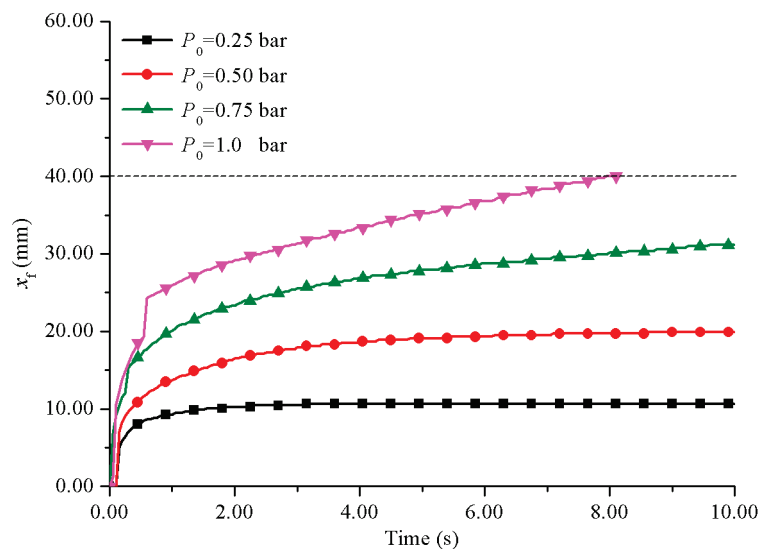
Figure 10. The relationship between resin reflux distance and time at different injection pressures.
