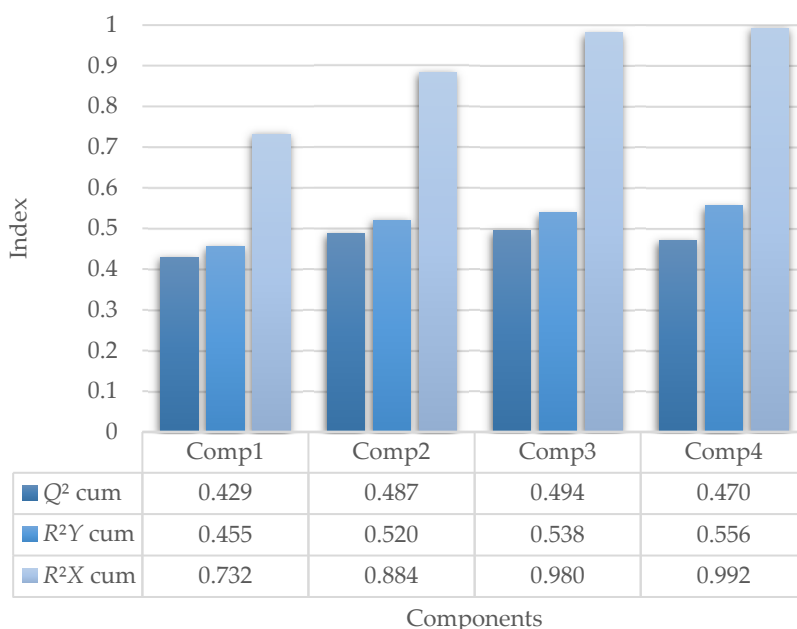
Figure 2. Model quality by number of components. Source: Figure by authors.
