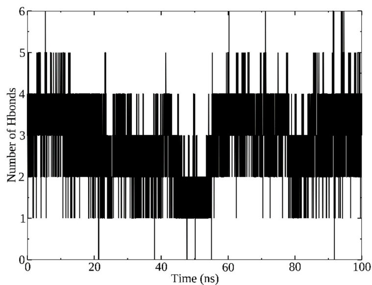
Figure 7. Hydrogen analysis for InhA complexed with ZINC000013629834.
