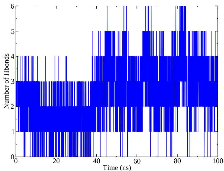
Figure 8. Hydrogen analysis for InhA complexed with ZINC000253411694.
