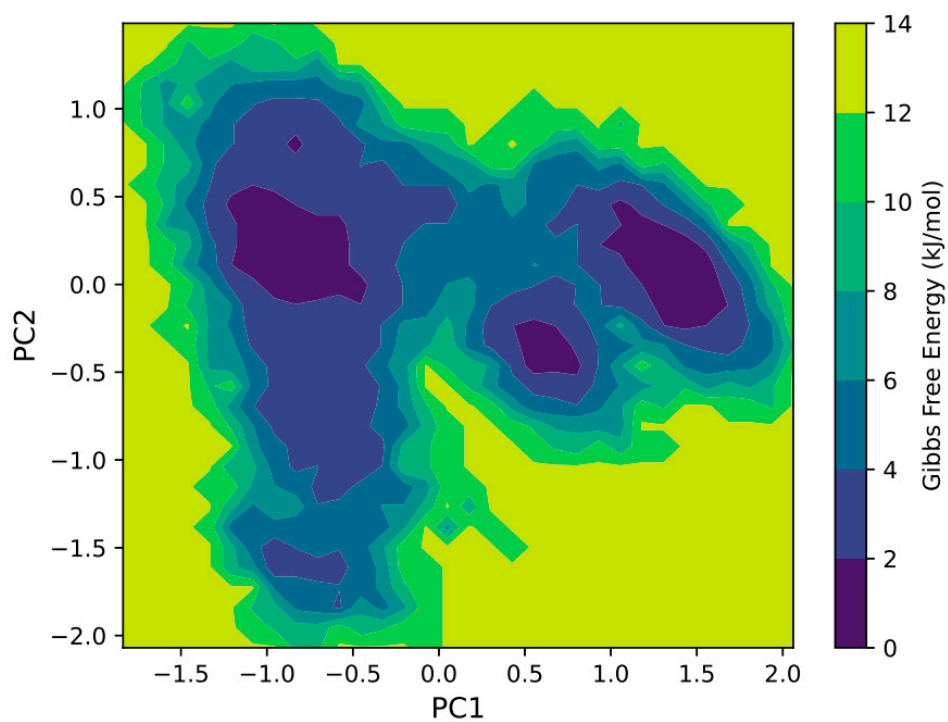
Figure 11. 2D free energy landscape for the complex for the Ligand ZINC000013629834.
