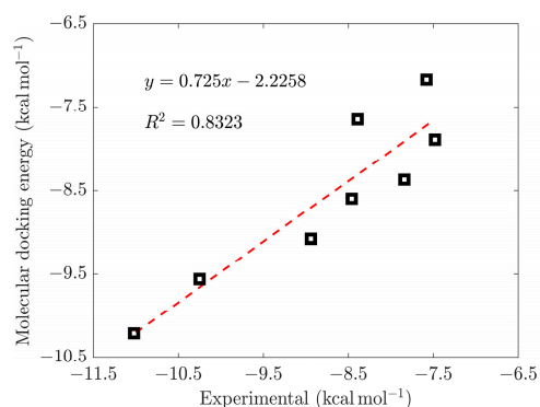
Figure 1. Docking protocol validation showing the relationship between the experimental data from the ITC and those calculated via molecular docking using AutoDock vina. The strong correlation
