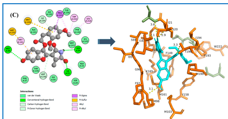
Figure 2. Interaction of residues from InhA with selected three compounds: (A) ZINC000013629834 (B) ZINC000253411694, and (C) Rifampicin.
