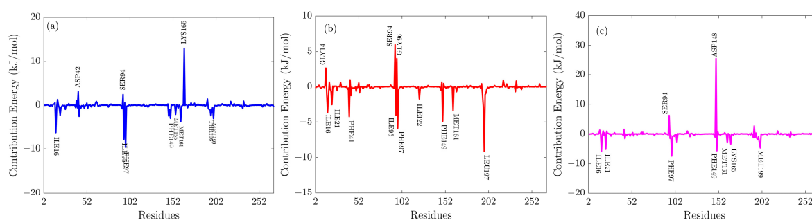
Figure 14. The energy contribution to protein–ligand binding (a) ZINC000013629834, (b) ZINC000253411694 and (c) Rifampicin.
