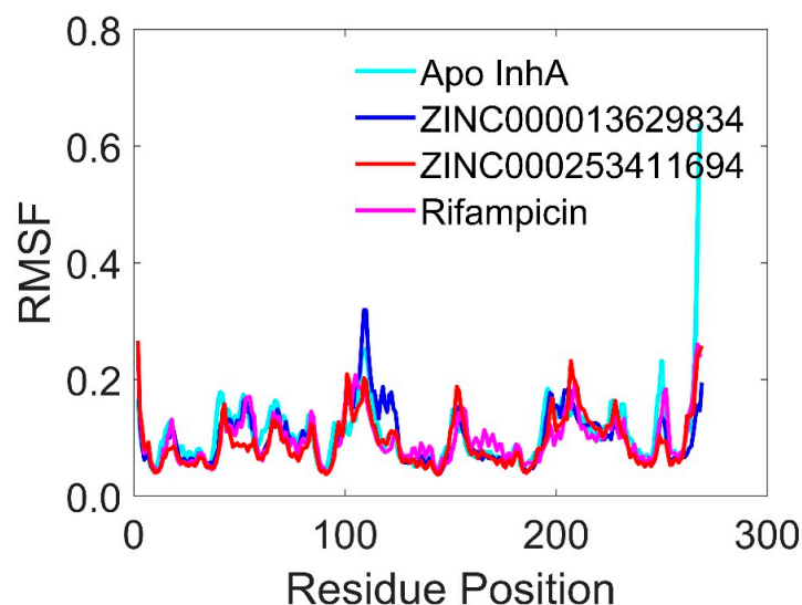
Figure 6. Root Mean Square Fluctuation for InhA , and when complexed with ZINC000013629834, ZINC000253411694 and Rifampicin.
