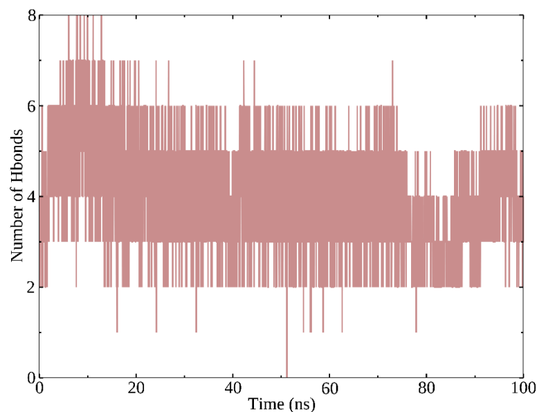
Figure 9. Hydrogen analysis for InhA complexed with Rifampicin.
