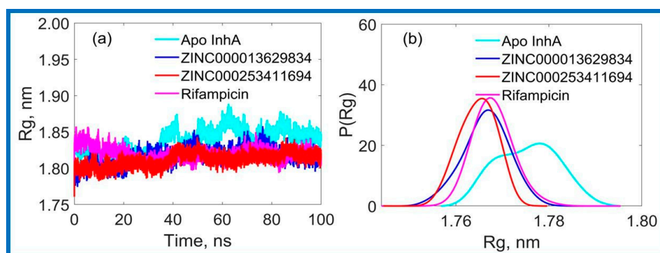
Figure 5. Radius of gyration for InhA , and when complexed with ZINC000013629834, ZINC000253411694, Rifampicin (a) time dependent and (b) probability density of R_g .
