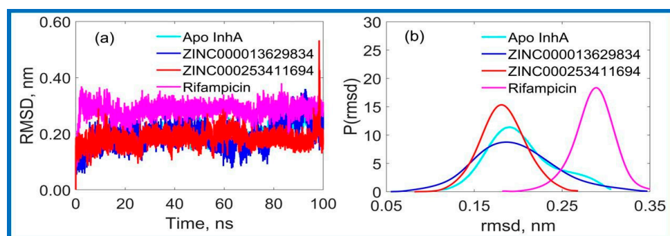
Figure 3. Root Mean Square Deviation of InhA , and when complexed with ZINC000013629834, ZINC000253411694, Rifampicin interacting with Amino Acids from InhA (a) time-dependent and (b) probability density of RMSD.
