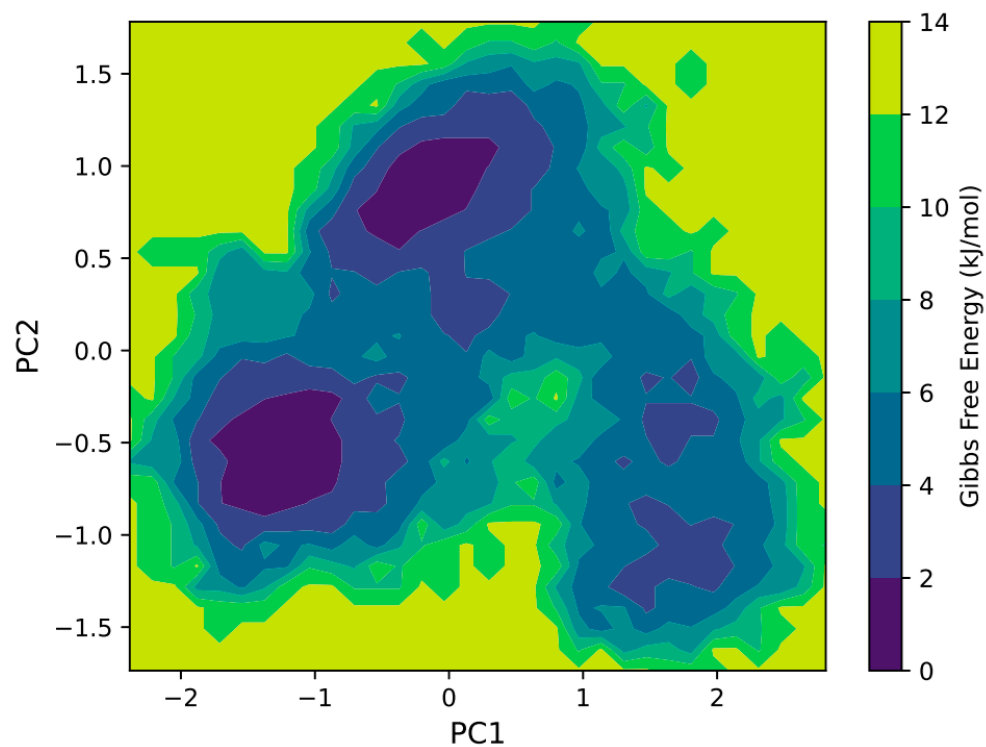
Figure 10. 2D free energy landscape for Apo protein InhA .
