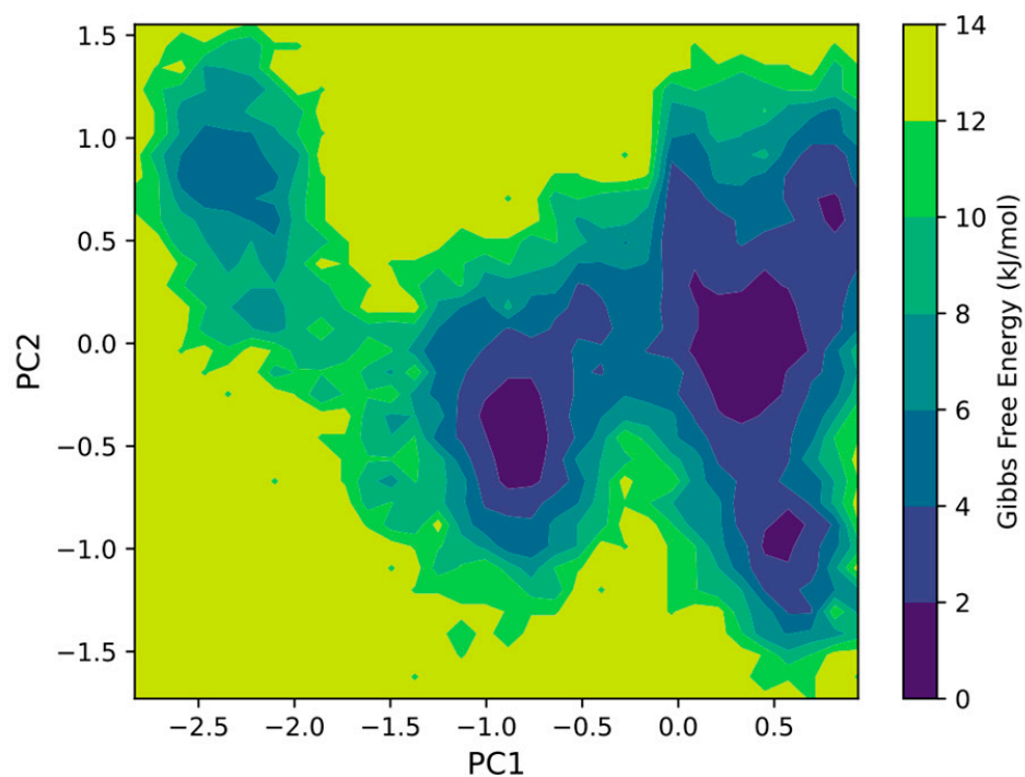
Figure 12. 2D free energy landscape for the complex for the Ligand ZINC000253411694.
