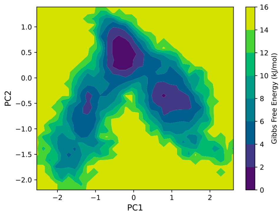
Figure 13. 2D free energy landscape for the complex of the Ligand Rifampicin.
