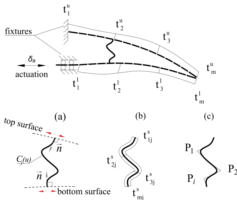
Figure 2. Top image: Setup for optimization, showing boundary conditions and thickness distribution on the top and bottom trailing-edge surfaces (thickness variation shown outward for clarity; in the algorithm, the outer surface is fixed and variations are shifted inward). Bottom image: Support structure represented by a spline. (a) Boundary conditions and initial-position variation on top/bottom surfaces; (b) thickness variables; (c) spline control variables.
