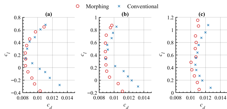
Figure 16. Lift to drag dependency at different flap and trailing-edge deflections from -0.05c to 0.05c in steps of 0.01c : (a) At 0^\circ angle of attack, (b) At 2^\circ angle of attack, (c) At 4^\circ angle of attack.
