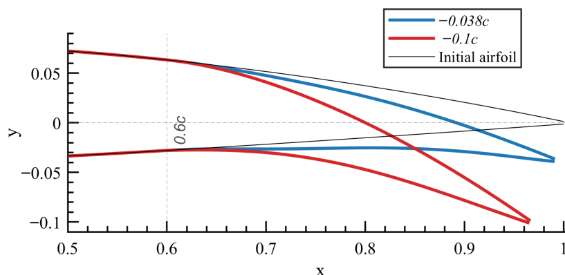
Figure 5. Aerodynamically optimized trailing-edge outer geometry, at -0.038c and -0.1c trailing edge displacement.
