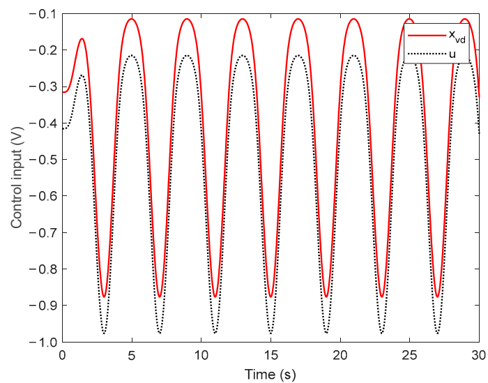
Figure 5. The actual control input and desired valve position of C1.
