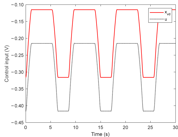
Figure 8. The actual control input and desired valve position of C1.
