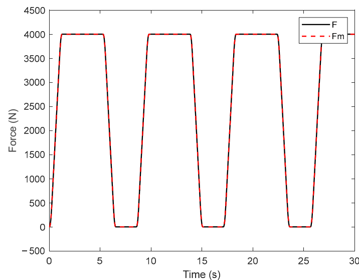
Figure 6. The desired trajectory and output of C1.
