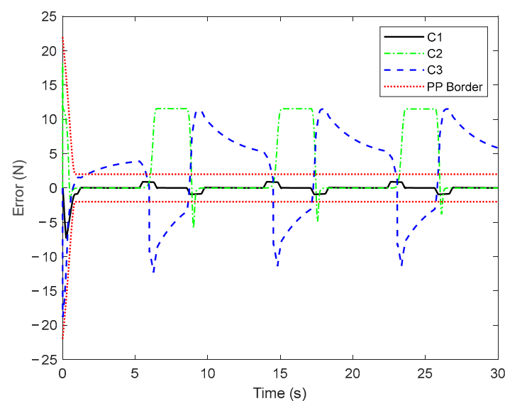
Figure 7. Tracking errors of the three compared controllers.
