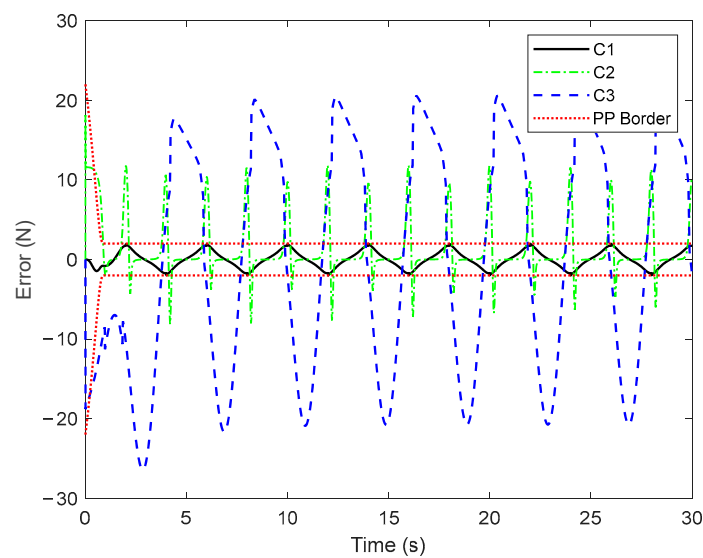
Figure 4. Tracking errors of the three compared controllers.
