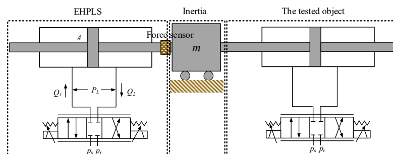
Figure 1. The schematic diagram of EHPLS.
