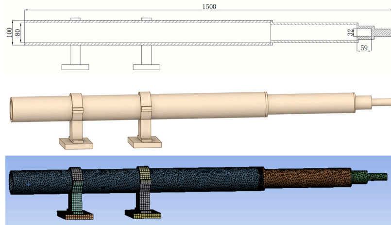
Figure 1. Three-dimensional geometric model, sectional view, and finite element meshing of the slender cantilever actuator.
