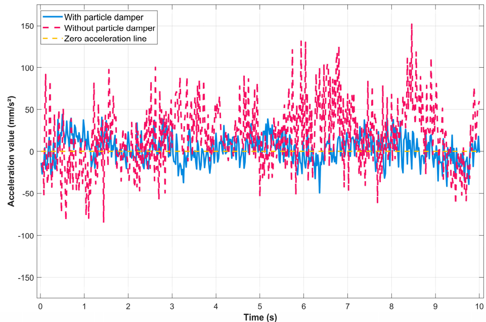
Figure 17. Time domain diagram of measuring points before and after damper installation.
