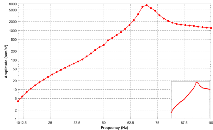
Figure 4. Harmonic response characteristics.
