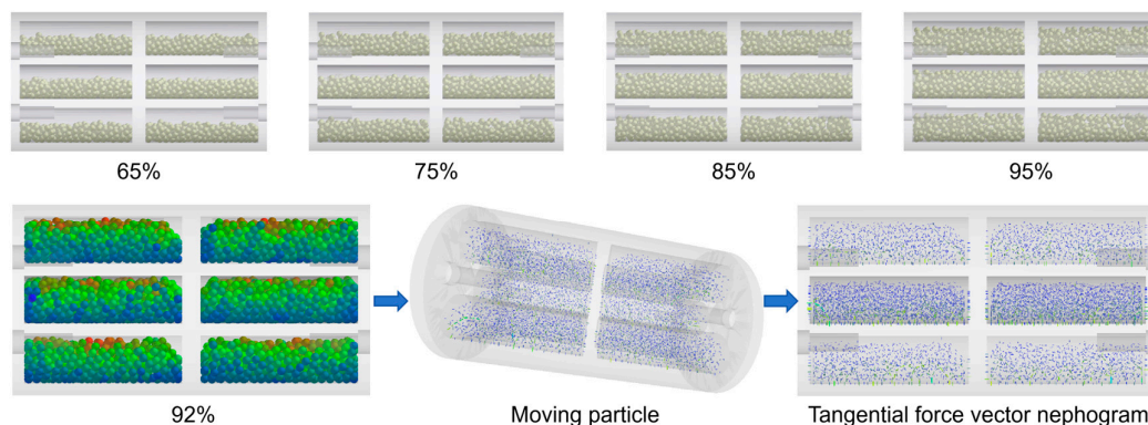
Figure 8. Diagram of different filling rates and particle motion energy.
