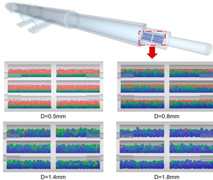
Figure 6. Simulation model and partial particle size filling diagram.
