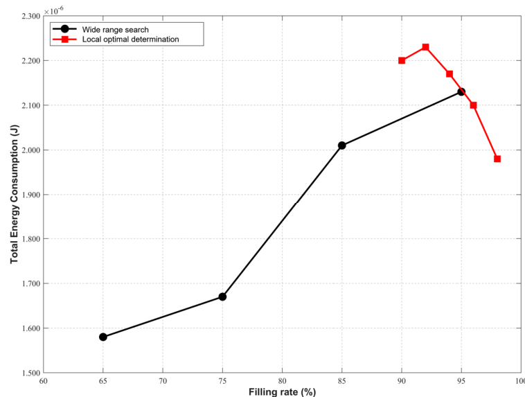
Figure 9. Energy consumption diagram for different filling rates.
