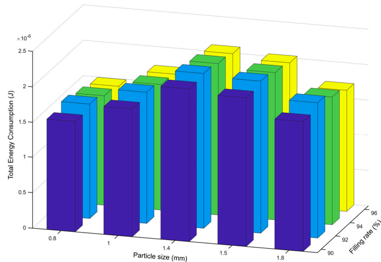
Figure 16. Experimentally derived energy consumption under different particle size and filling ratio combinations.
