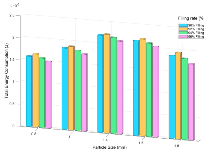
Figure 10. Optimal solution for energy consumption of particle damper.
