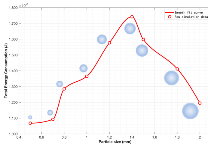
Figure 7. Single-cycle energy dissipation performance of particle dampers with varying particle sizes.
