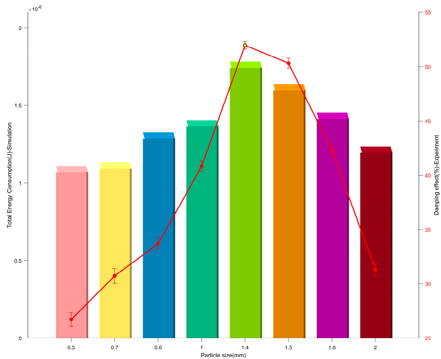
Figure 14. Figure of experimental and simulation data.
