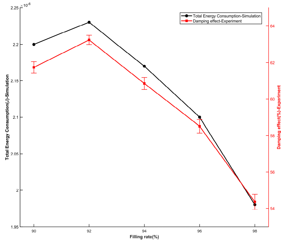
Figure 15. Comparison between experiment and simulation under different filling rates.
