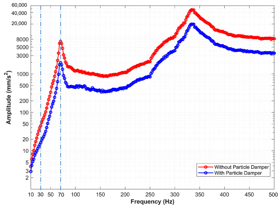
Figure 18. Broadband sweep response diagram under optimal damping parameters.
