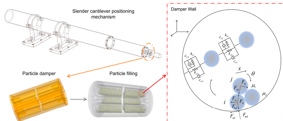
Figure 5. Micro-contact and energy transfer mechanism of particle damping under low-frequency micro-vibration.
