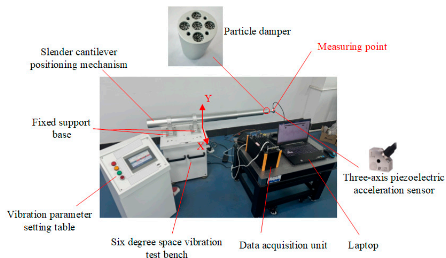
Figure 11. Integral fixed orientation and measuring points.
