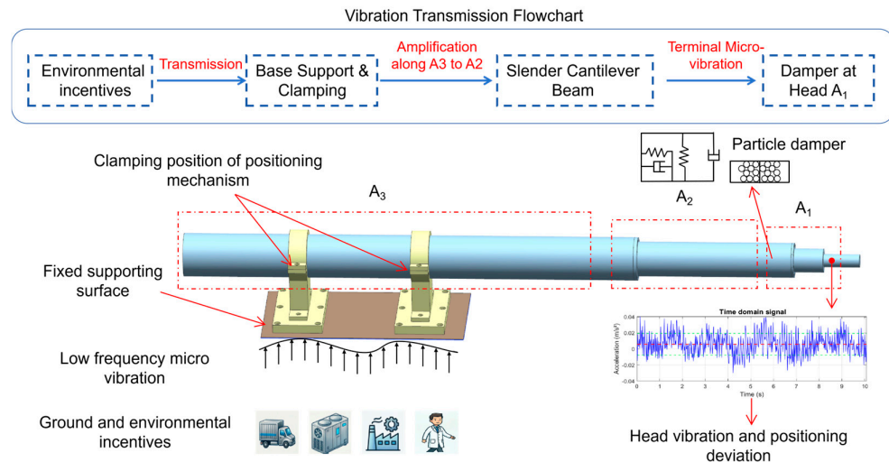
Figure 3. Schematic of environmental vibration excitation, particle damper installation layout, and vibration transmission route.
