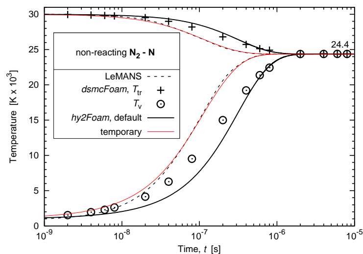
Figure 5. V-T relaxation of a N_2-N heat bath.
