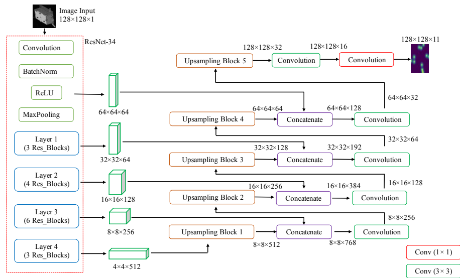
Figure 11. ResNet34-U-Net Architecture.
