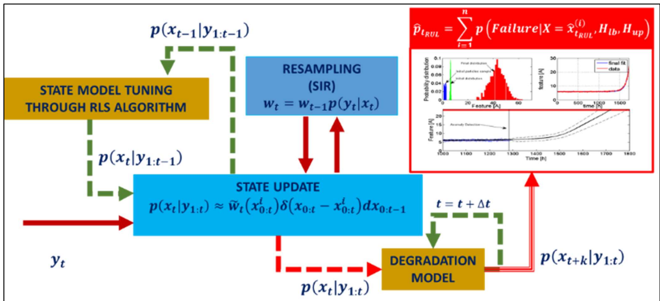
Figure 17. Scheme of the employed particle-filtering algorithm.
