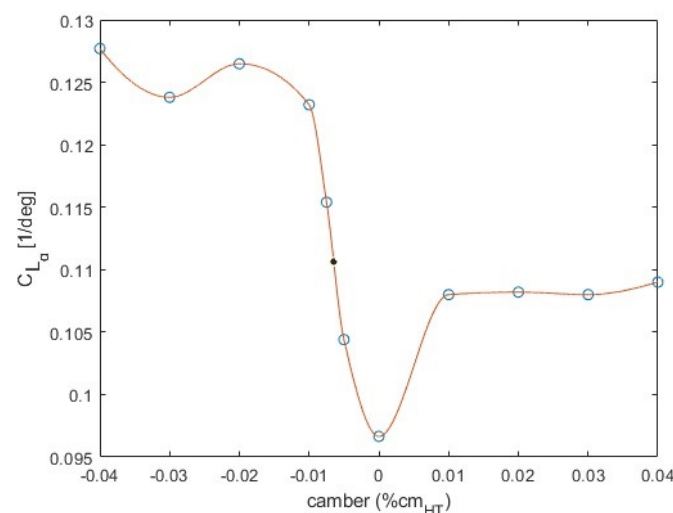
Figure 5. Variation of C_{L_\alpha} with camber at X_{c_{max}} = 0.5 .
