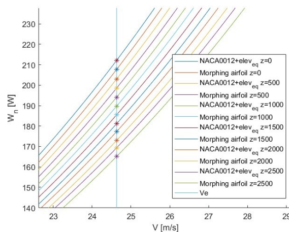
Figure 19. Detail of aircraft power required curves at the studied altitudes.
