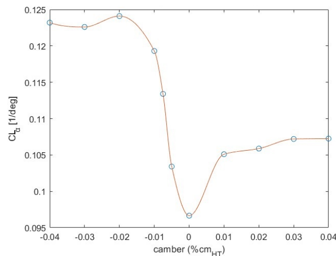
Figure 4. Variation of C_{L_\alpha} with camber at X_{c_{max}} = 0.4 .
