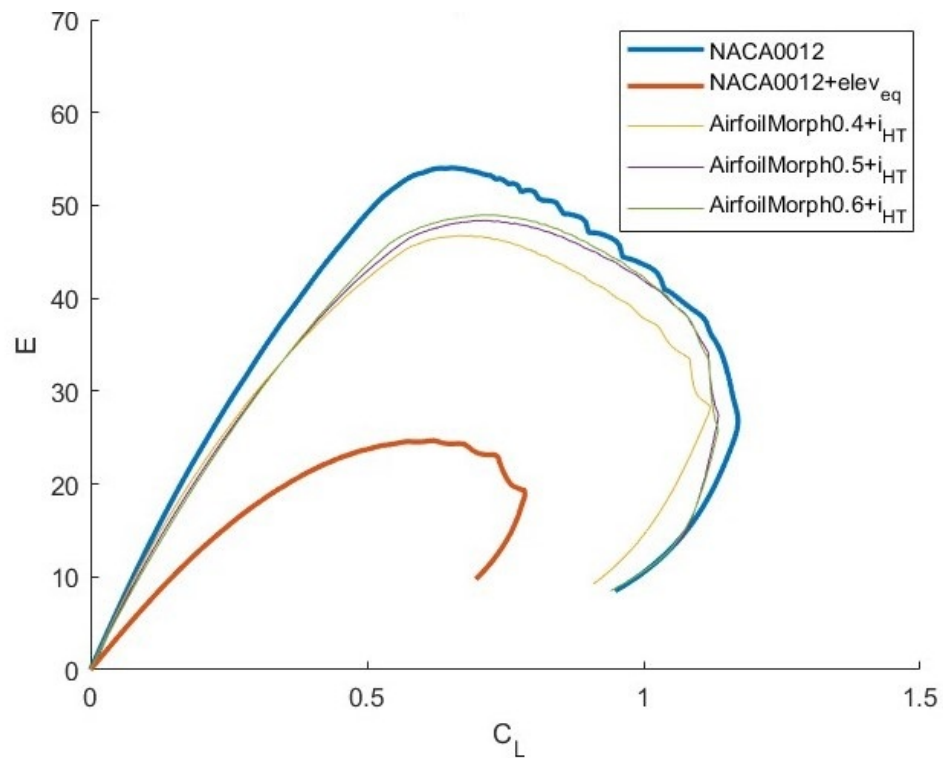
Figure 11. E vs. C_L curve of NACA 0012, NACA 0012+ \delta_{eq} and the three morphing airfoils with i_{HT} .
