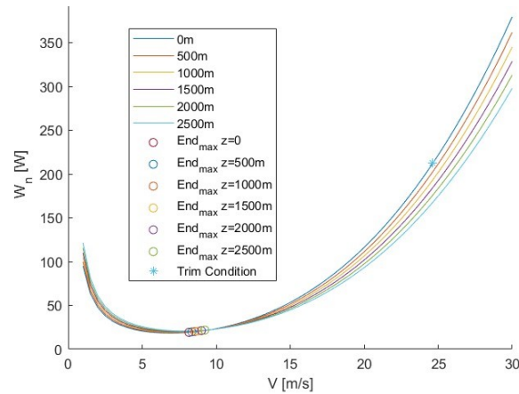
Figure 17. Aircraft power required curves (HT with NACA 0012 + \delta_{e_{eq}} ) at studied altitudes.
