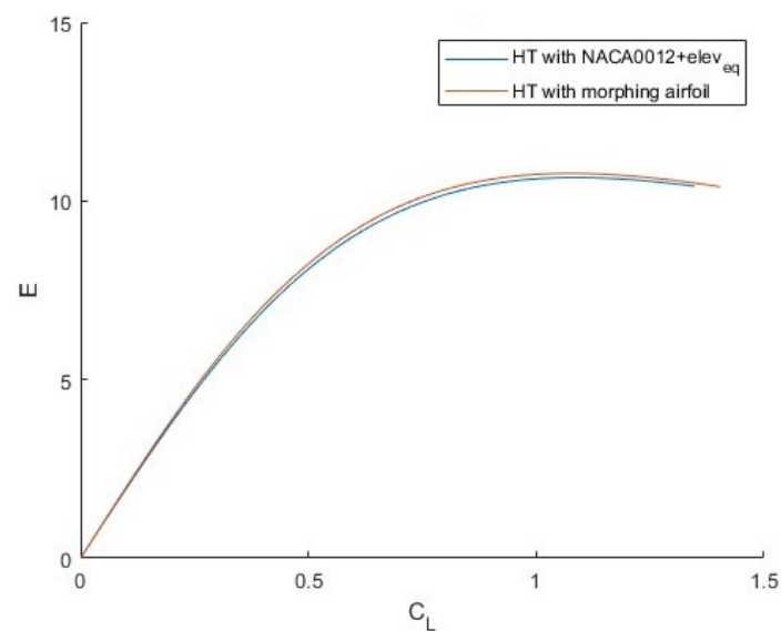
Figure 16. E vs. C_L for aircraft equipped with standard tail and with a morphing tail.
