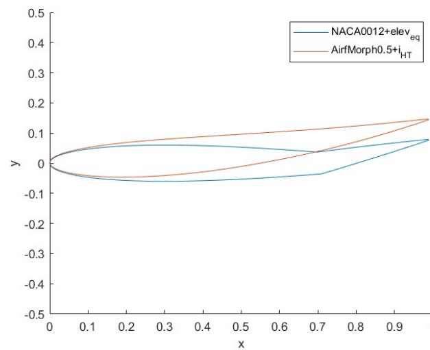
Figure 12. NACA 0012 + \delta_{e_{eq}} and morphing airfoil.
