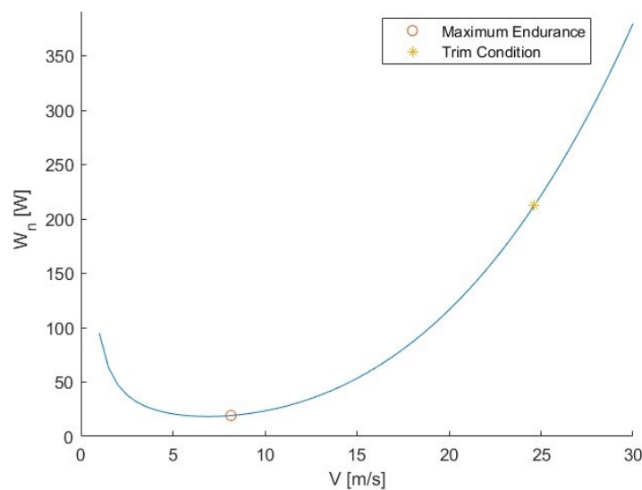
Figure 13. Aircraft power required curves (HT with NACA 0012+ \delta_{eq} ) at z = 0 .
