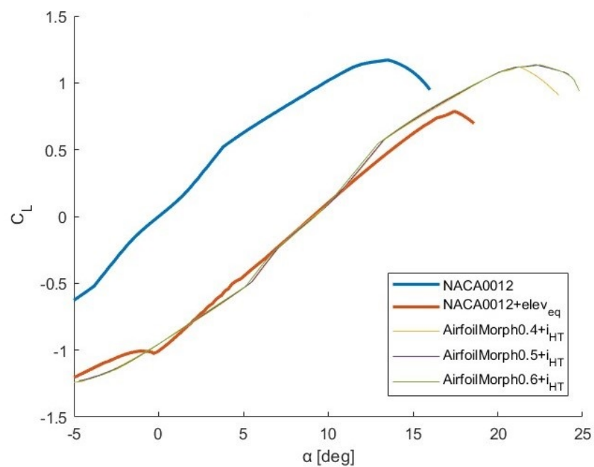
Figure 8. C_L vs. \alpha curve of NACA 0012, NACA 0012 + \delta_{eq} and the three morphing airfoils with i_{HT} .
