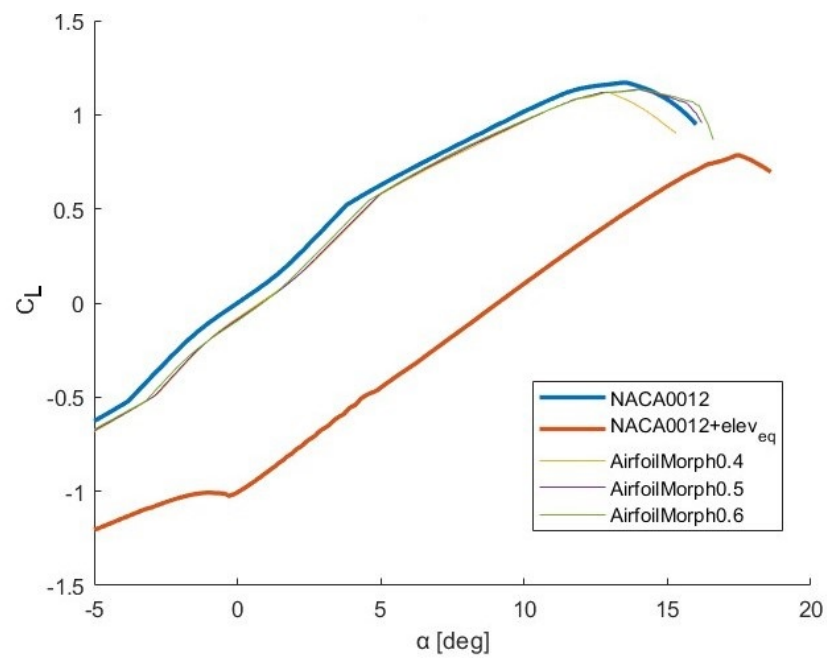
Figure 7. C_L vs. \alpha curve of NACA 0012, NACA 0012 + \delta_{eq} and the three morphing airfoils.
