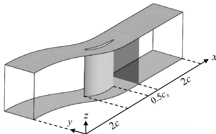
Figure 1. Flow domain for PVD compressor cascade.
