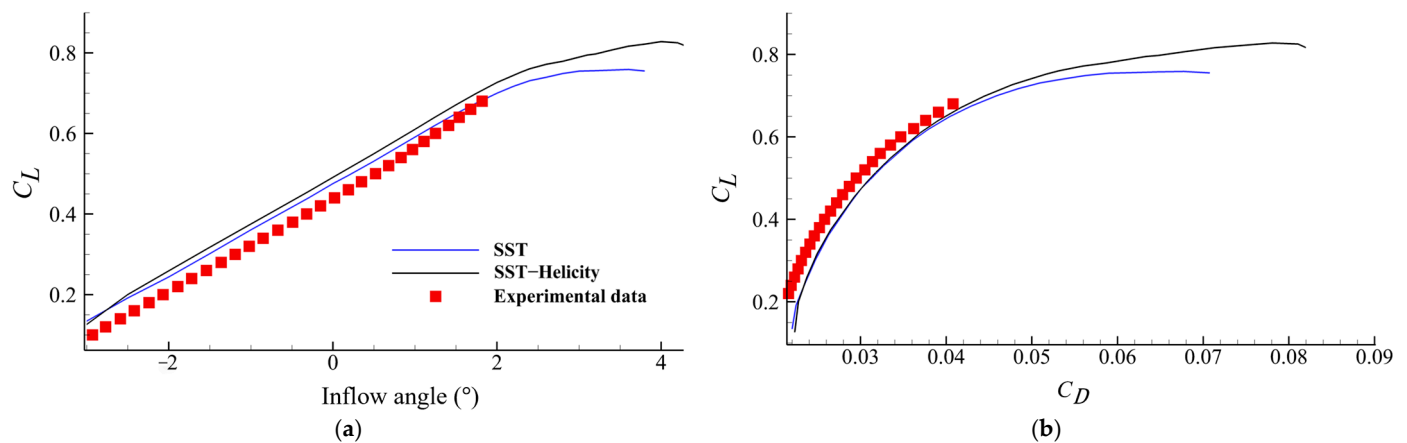
Figure 12. DLR-F6 aerodynamic characteristics: (a) C_L vs. angle of attack; (b) lift-drag polar.
