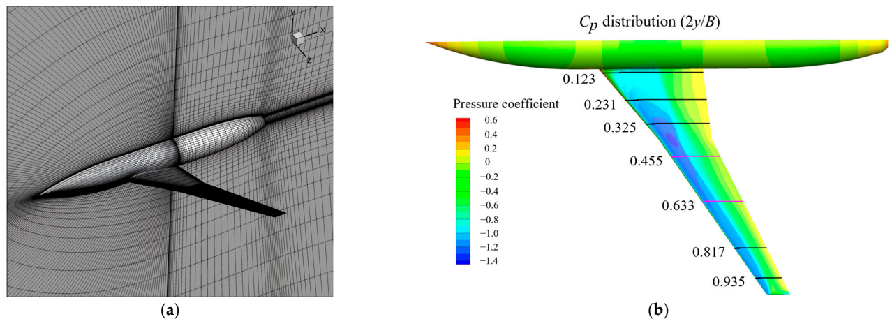
Figure 8. Configuration of ARA M100 wing–fuselage: (a) 3D mesh view; (b) pressure coefficient contour.
