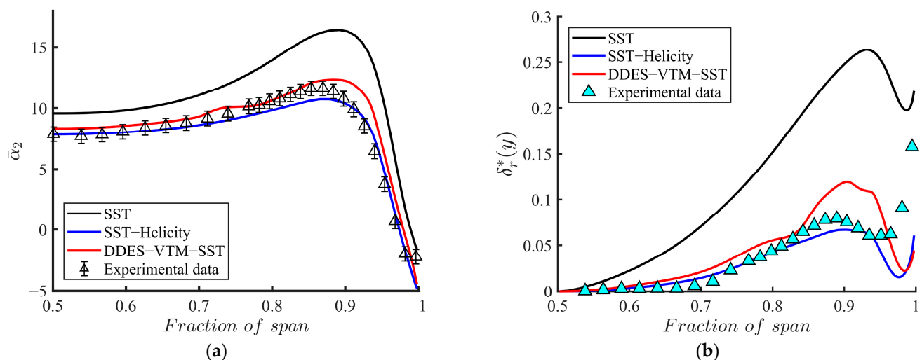
Figure 5. Evaluation of blockage due to corner separation: (a) mass-averaged yaw angle at 1.5c_x cut plane; (b) relative displacement thickness at 0.99c_x cut plane.
