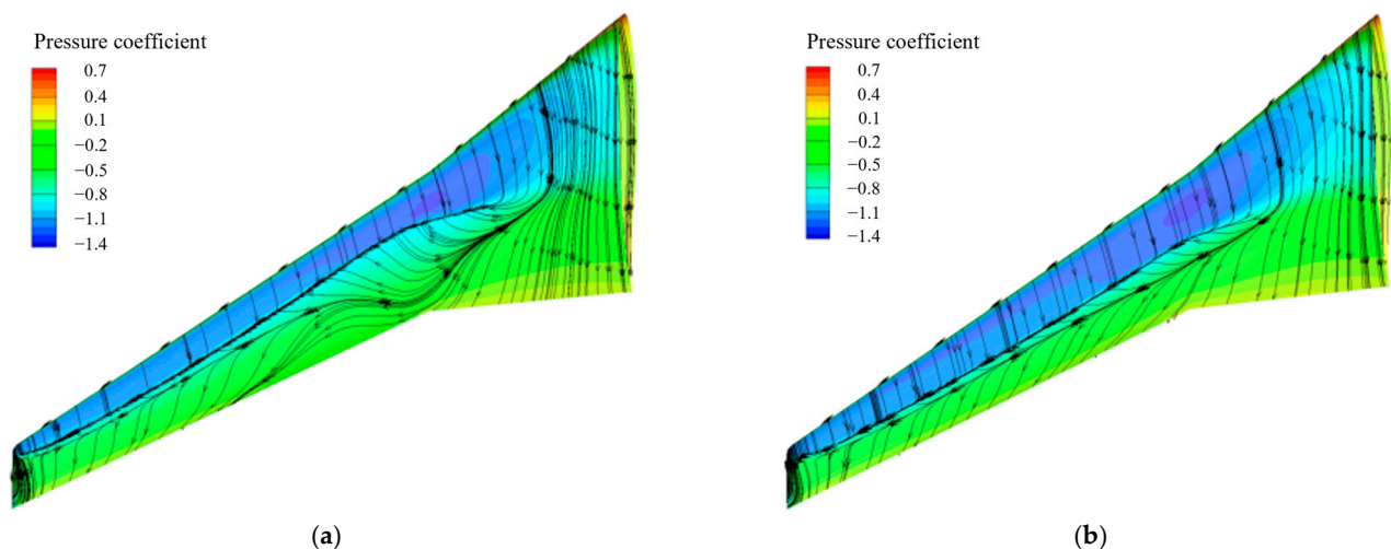
Figure 9. Comparison of surface pressure and streamline patterns: (a) SST; (b) SST-Helicity.
