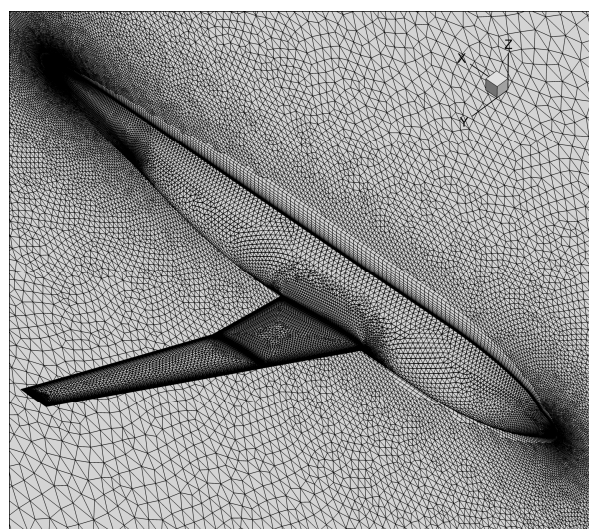
Figure 11. DLR-F6 configuration.
