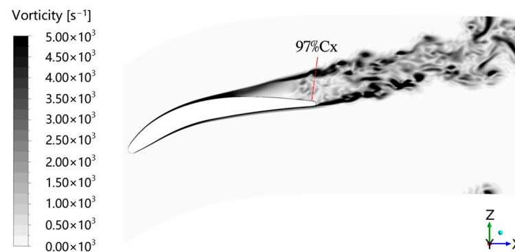
Figure 6. Vorticity magnitude at 11%h (DDES-VTM-SST) with analysis line location (97% c_x ).
