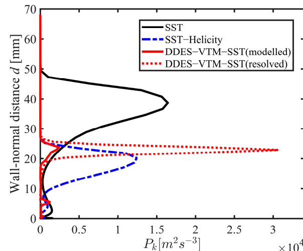
Figure 7. Wall-normal profiles of TKE production rate along the analysis line.
