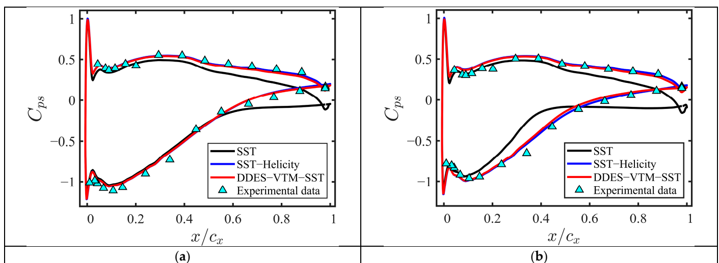
Figure 4. Pressure coefficient ( C_{ps} ) distributions: (a) near midspan (46% h ); (b) near endwall (11% h ).
