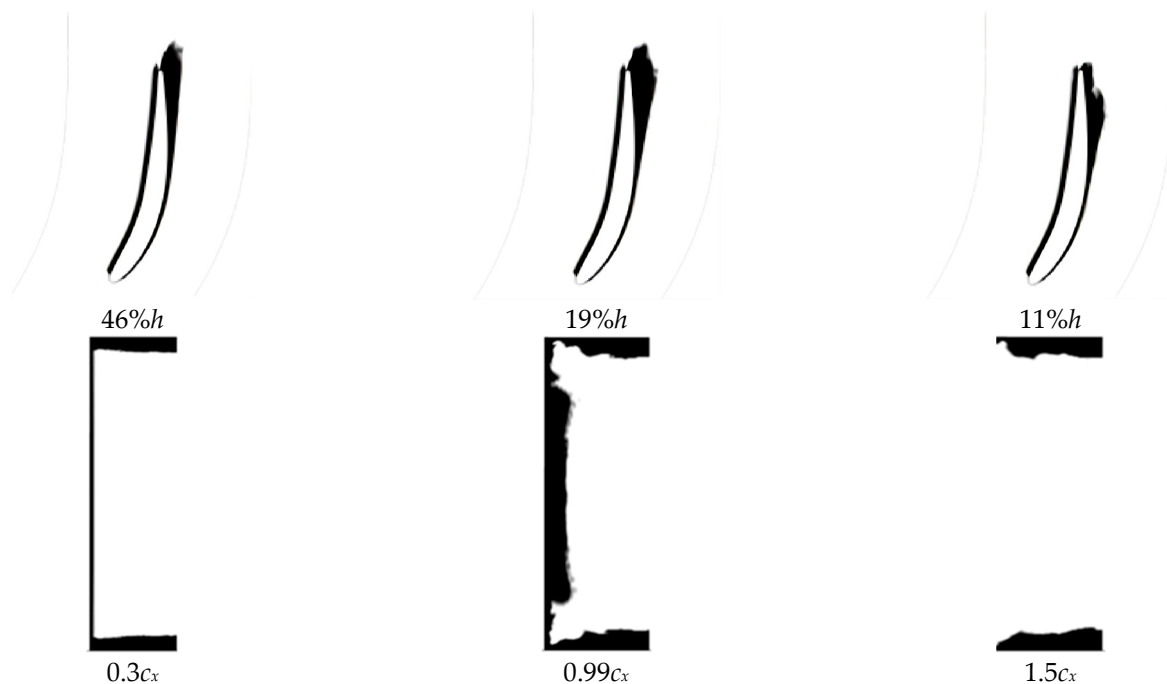
Figure 2. Comparison of f_{DES} distributions between DDES-SST and DDES-VTM-SST models at selected cross-sections.
