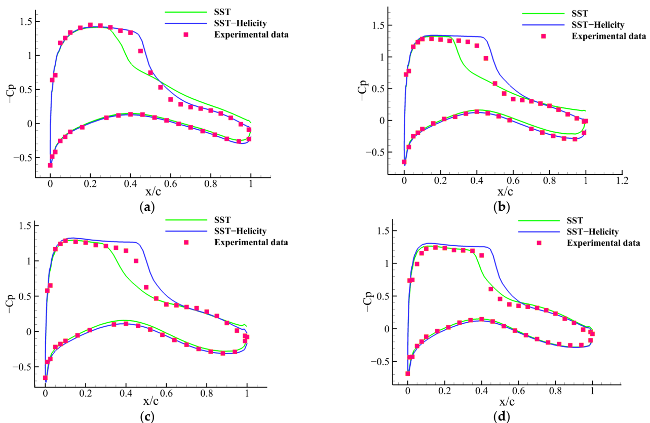
Figure 10. Comparison of surface pressure coefficient distributions at four spanwise stations: (a) 2y/B = 0.325 ; (b) 2y/B = 0.455 ; (c) 2y/B = 0.633 ; and (d) 2y/B = 0.817 .
