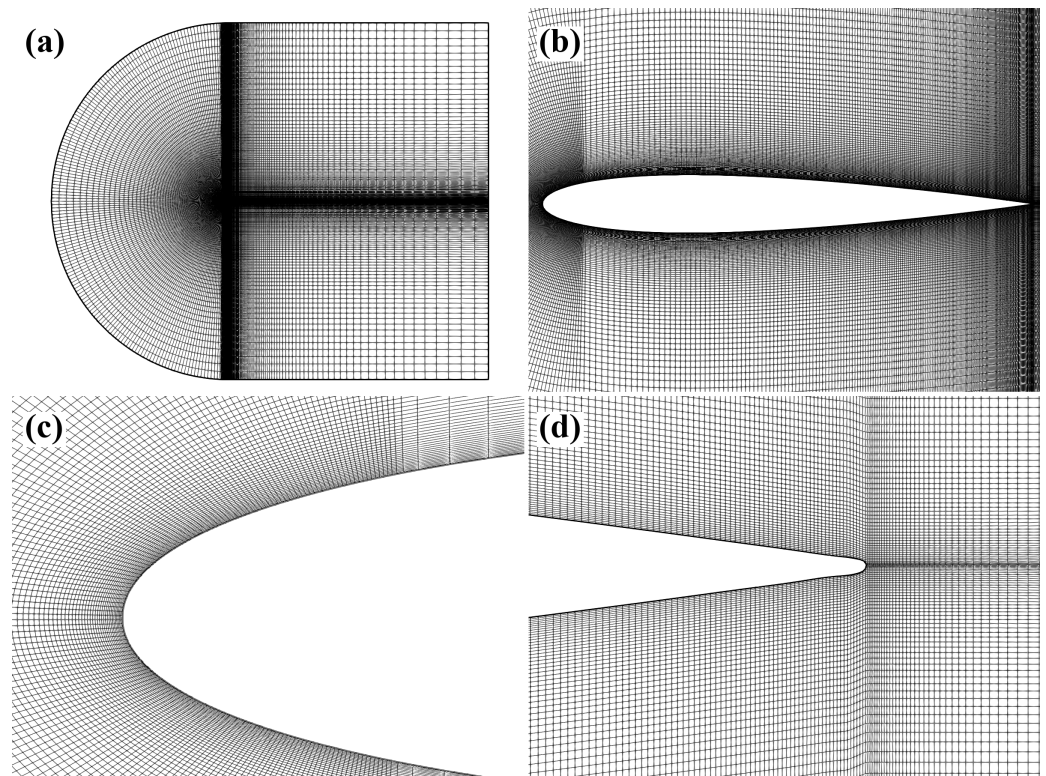
Figure 1. Structured C-grid topology for the NACA 0012 airfoil: (a) global computational domain; (b) mesh distribution around the airfoil; (c) magnified view of the leading edge; (d) trailing edge and wake refinement. Representative structured mesh (188 k cells) used for production runs.
