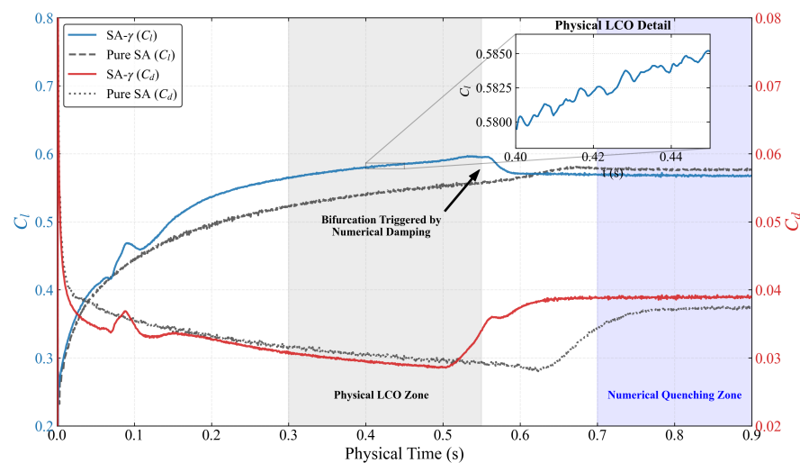
Figure 9. Dual-axis time-history of C_l and C_d at \alpha = 6^\circ (Time step \Delta t = 2 \times 10^{-5} \text{ s} , Inner iterations = 20): Visualization of the transition from physical LCO to numerical quenching. The simultaneous lift collapse and drag surge highlights the catastrophic failure of the pseudo-steady attractor. The physical time step is \Delta t = 2 \times 10^{-5} \text{ s} , meaning 0.1 s corresponds to 5000 iterations.
