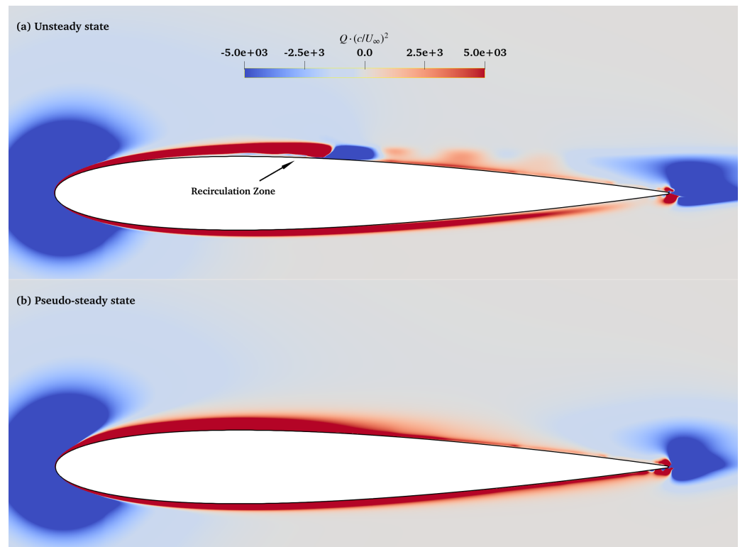
Figure 16. Instantaneous vortical structures visualized by the Q-criterion ( Q = 5 \times 10^3 ). (a) The physical attractor resolves coherent vortex shedding. (b) The pseudo-steady attractor exhibits numerical silence , visually confirming the suppression of the Kelvin-Helmholtz instability by numerical dissipation.
