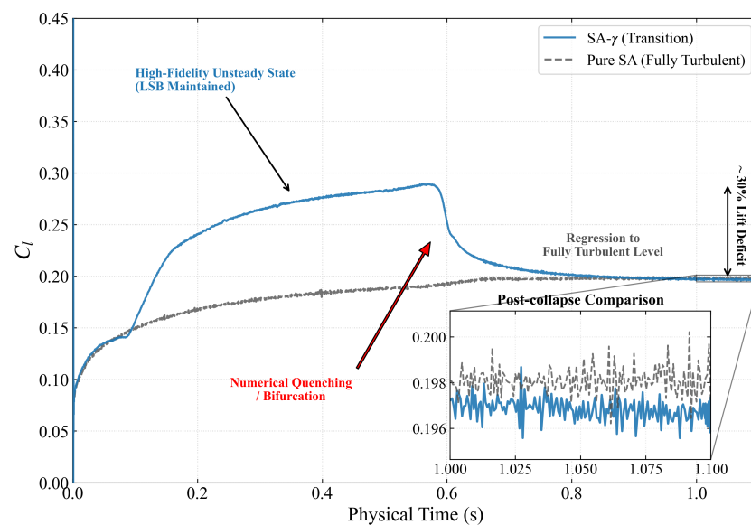
Figure 8. Time-history of lift coefficient at \alpha = 2^\circ (Time step \Delta t = 2 \times 10^{-5} s, Inner iterations = 20): Demonstration of the “pseudo-convergence trap” where the transition model regresses to the fully turbulent baseline level. The physical time step is \Delta t = 2 \times 10^{-5} s, meaning 0.1 s corresponds to 5000 iterations.
