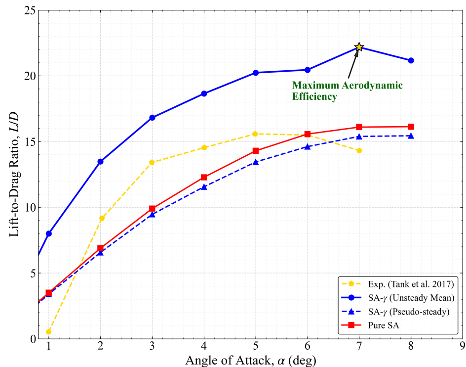
Figure 7. Lift-to-drag ratio ( L/D ) comparison: Identification of peak efficiency and the deficit induced by numerical quenching.
