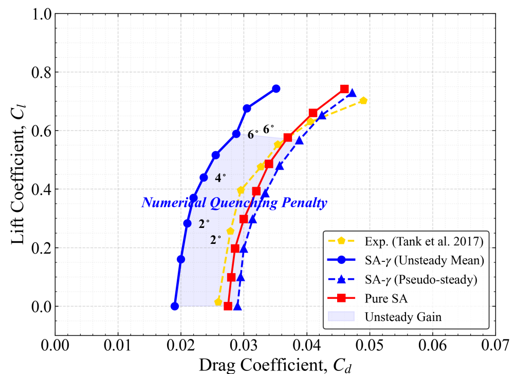
Figure 6. Aerodynamic drag polar ( C_l vs. C_d ): Visualization of the topological separation between the physical limit-cycle attractor and the pseudo-steady attractor.
