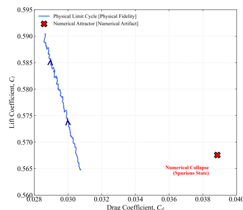
Figure 11. Phase portrait in the C_d - C_l plane at \alpha = 6^\circ : Geometric separation between the physical limit-cycle attractor and the spurious fixed-point attractor.
