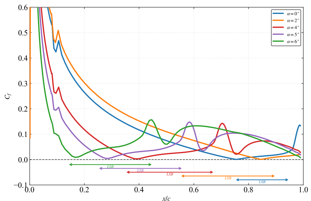
Figure 12. Chordwise distribution of the time-averaged skin friction coefficient ( C_f ) identifying the LSB extent ( C_f < 0 ). The topological contraction of the bubble with increasing \alpha is a critical physical feature that is lost during numerical quenching.
