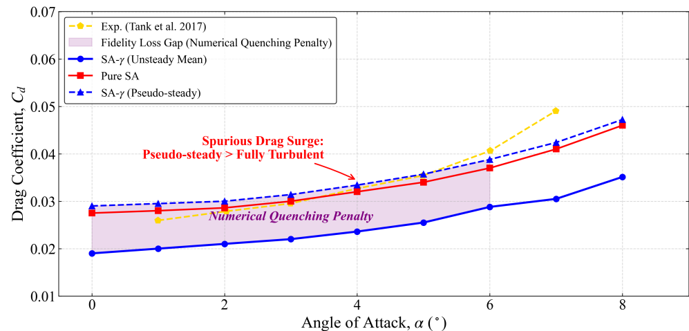
Figure 5. Drag coefficient ( C_d ) vs. angle of attack ( \alpha ): Evidence of the “Drag Mechanism Inversion” where numerical quenching leads to a spurious drag surge exceeding turbulent levels.
