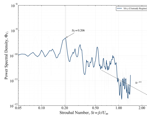
Figure 10. PSD of lift fluctuations at \alpha = 6^\circ : The dominant peak at St \approx 0.2 is consistent with shear-layer shedding reported in the experimental benchmarks of Yarusevych et al. [18]. The spectrum also exhibits broadband high-frequency content prior to numerical quenching.
