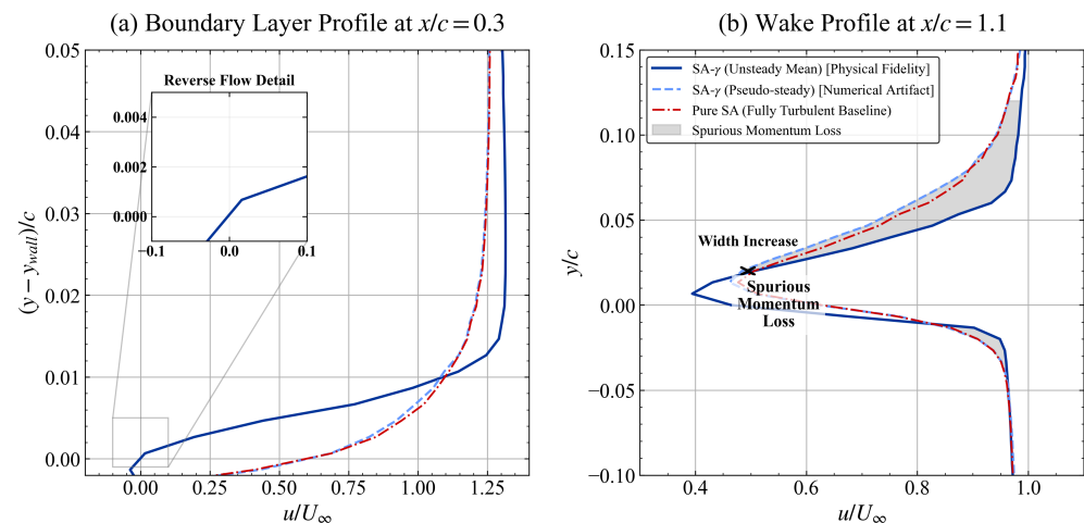
Figure 14. Velocity profiles at \alpha = 6^\circ comparing unsteady-mean and pseudo-steady states. The “Spurious Momentum Loss” in the wake (b) provides a kinematic explanation for the drag inversion, linking wake broadening to entropy generation.
