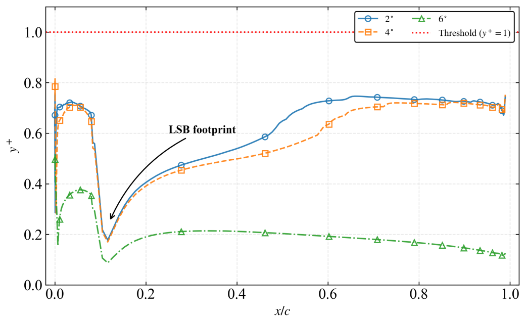
Figure 2. Chordwise distribution of the wall-normal dimensionless distance y^+ on the suction surface. The threshold y^+ < 1.0 is maintained for all investigated angles of attack to ensure viscous sublayer resolution.
