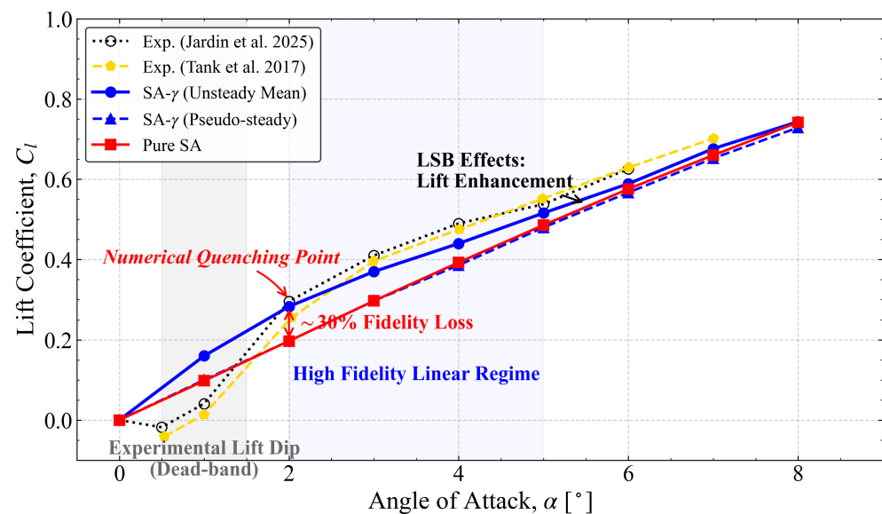
Figure 4. Lift coefficient ( C_l ) vs. angle of attack ( \alpha ): Comparison showing the LSB-induced lift enhancement. The “Numerical Quenching Point” at \alpha = 2^\circ marks the collapse of the physical attractor.
