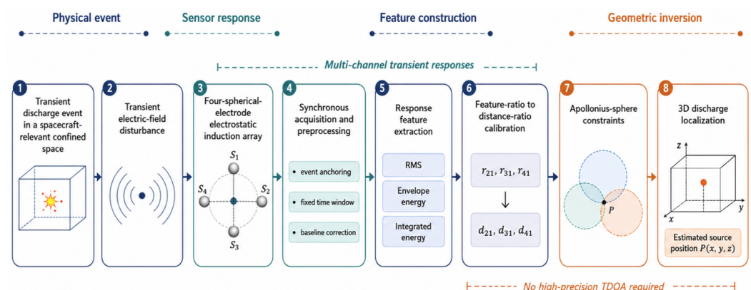
Figure 1. Overall system and method framework for electrostatic-induction-array-based discharge localization. The figure defines four stages: physical event generation, four-channel electrostatic-induction sensing and preprocessing, feature-ratio construction with Power + offset calibration, and Apollonius-sphere-based three-dimensional inversion. RMS denotes root-mean-square value. The distance ratios d_{21} , d_{31} , and d_{41} are estimated from calibrated feature ratios relative to sensor 1. The dashed note indicates that high-precision TDOA estimation is not required.
