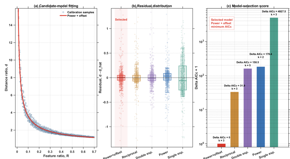
Figure 6. Representative model comparison for selecting the feature-ratio–distance-ratio calibration function using the simulated RMS dataset. Here, R denotes the feature ratio, d denotes the geometric distance ratio, and AICc denotes the corrected Akaike information criterion. (a) Fitting curve of the selected Power + offset model. (b) Residual distributions d - \hat{d} of the evaluated models. (c) Model selection scores expressed as \Delta AICc + 1 , where the minimum-AICc Power + offset model has \Delta AICc = 0 . Adding 1 enables logarithmic-scale visualization. This representative result indicates that the selected model provides a favorable balance between fitting accuracy and model complexity.
