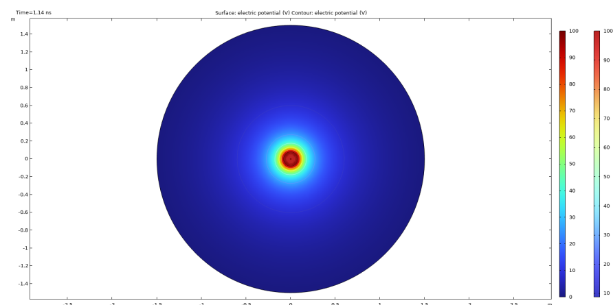
Figure 4. Representative COMSOL electrostatic-potential distribution for one sampled needle–plate source position. The potential is concentrated near the source region and decays over the surrounding computational air domain. This result is used as a qualitative visualization of the electrostatic coupling field in the auxiliary simulation rather than as a direct transient plasma-discharge waveform.
