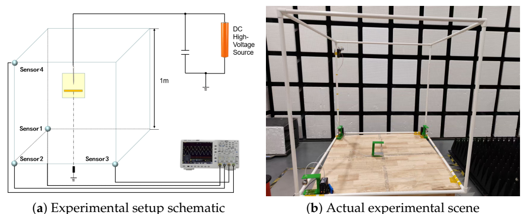
Figure 3. Experimental platform for validating the proposed localization framework. (a) Schematic arrangement of the 1 m 3 confined-space platform, four electrostatic induction sensors, needle–plate discharge source, high-voltage source, grounding path, and acquisition system. (b) Actual laboratory scene of the confined-space validation platform, showing the physical frame, sensor supports, and discharge-source arrangement.
