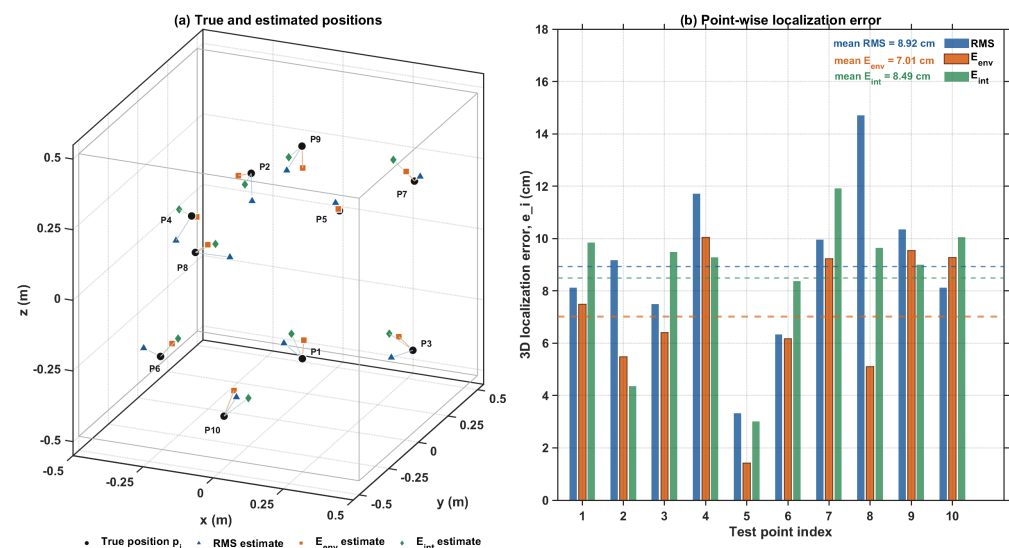
Figure 8. Localization results for the ten discharge test points. (a) Three-dimensional comparison between the true discharge positions p_i and the estimated positions \hat{p}_i obtained using RMS, envelope energy, and integrated energy. (b) Three-dimensional localization error comparison, where e_i = \|\hat{p}_i - p_i\|_2 . The dashed horizontal lines denote the mean localization errors of the corresponding feature groups, and the envelope-energy result is emphasized because it gives the lowest mean three-dimensional localization error in the present test dataset.
