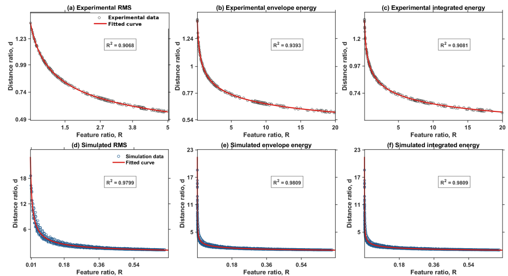
Figure 7. Feature-ratio–distance-ratio fitting results for the RMS, envelope-energy, and integrated-energy features. Solid curves denote the fitted Power + offset mapping \hat{d} = aR^b + c , where R is the feature ratio and \hat{d} is the estimated distance ratio. In the upper panels, markers denote experimental fitting data; in the lower panels, markers denote simulation samples. The envelope-energy feature provides the highest experimental fitting consistency among the three response representations.
