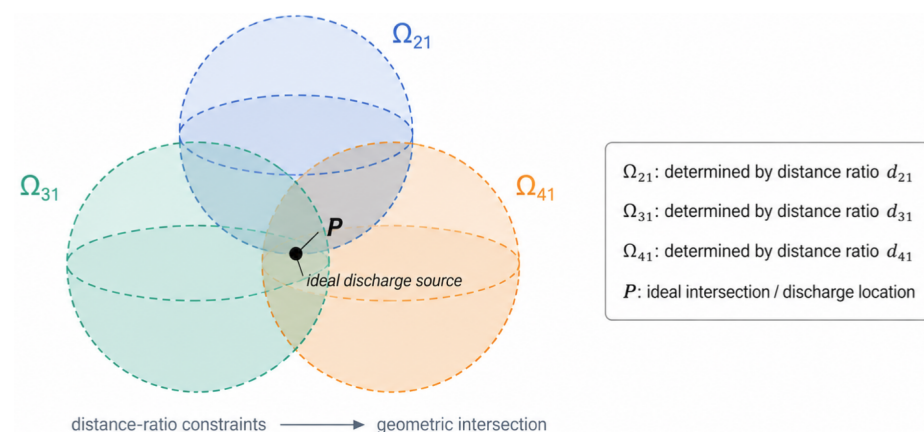
Figure 2. Schematic illustration of the Apollonius-sphere localization principle. Three independent distance-ratio constraints, d_{21} , d_{31} , and d_{41} , define the corresponding Apollonius spheres \Omega_{21} , \Omega_{31} , and \Omega_{41} . Their ideal intersection gives the discharge position P , while in noisy cases, the final coordinate is obtained by nonlinear residual minimization.
