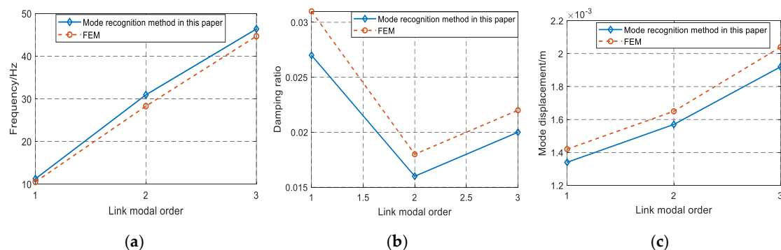
Figure 10. Modal parameters of link deformation under different identification methods: (a) Frequency, (b) Damping ratio, (c) Mode displacement.
