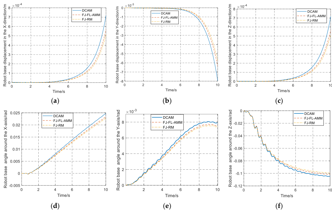
Figure 6. Pose changes of space robot base under different analysis models: Position: (a) X-direction, (b) Y-direction, (c) Z-direction; attitude: (d) X-axis, (e) Y-axis, (f) Z-axis.
