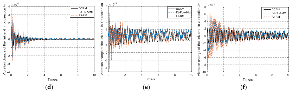
Figure 8. Flexible vibration of space robot link under different analysis models: Link 1: (a) X direction, (b) Y direction, (c) Z direction; Link 2: (d) X direction, (e) Y direction, (f) Z direction.
