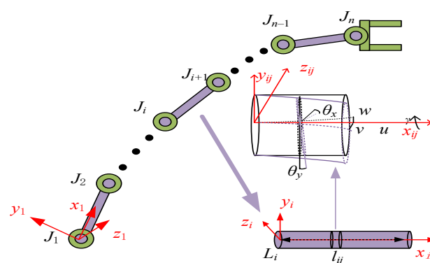
Figure 2. Force analysis of flexible link.
