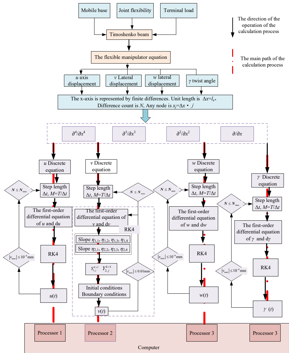
Figure 3. Parallel computing process with double difference and limited resources.
