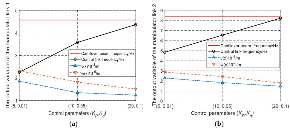
Figure 9. The output variables of the mechanical system under different control parameters: (a) Link 1, (b) Link 2.
