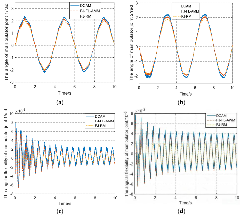
Figure 7. Joint change for space robots under different analysis models: (a) joint angle 1, (b) joint angle 2, (c) joint flexibility 1, (d) joint flexibility 2.
