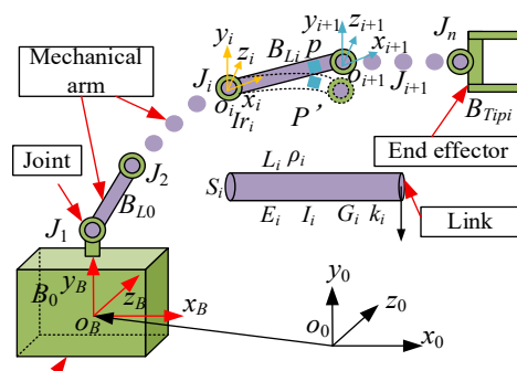
Figure 1. The simplified structure model of the space robot.
