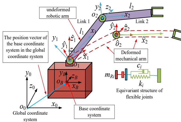
Figure 5. The overall structure of 2DOF flexible space robot.
