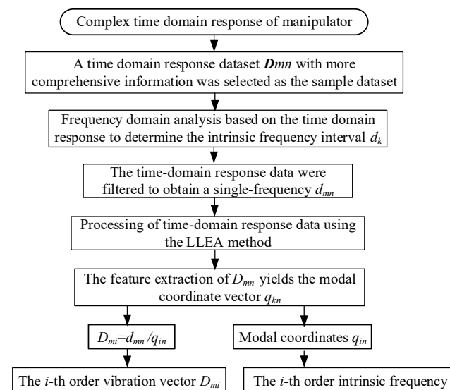
Figure 4. Modal recognition process by time-domain response of flexible link.
