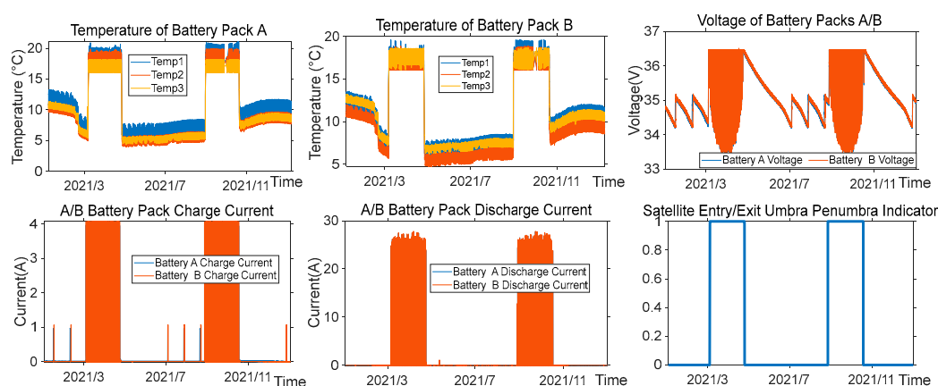
Figure 1. Satellite battery pack: temperature and electrical parameter graphs (one eclipse season).
