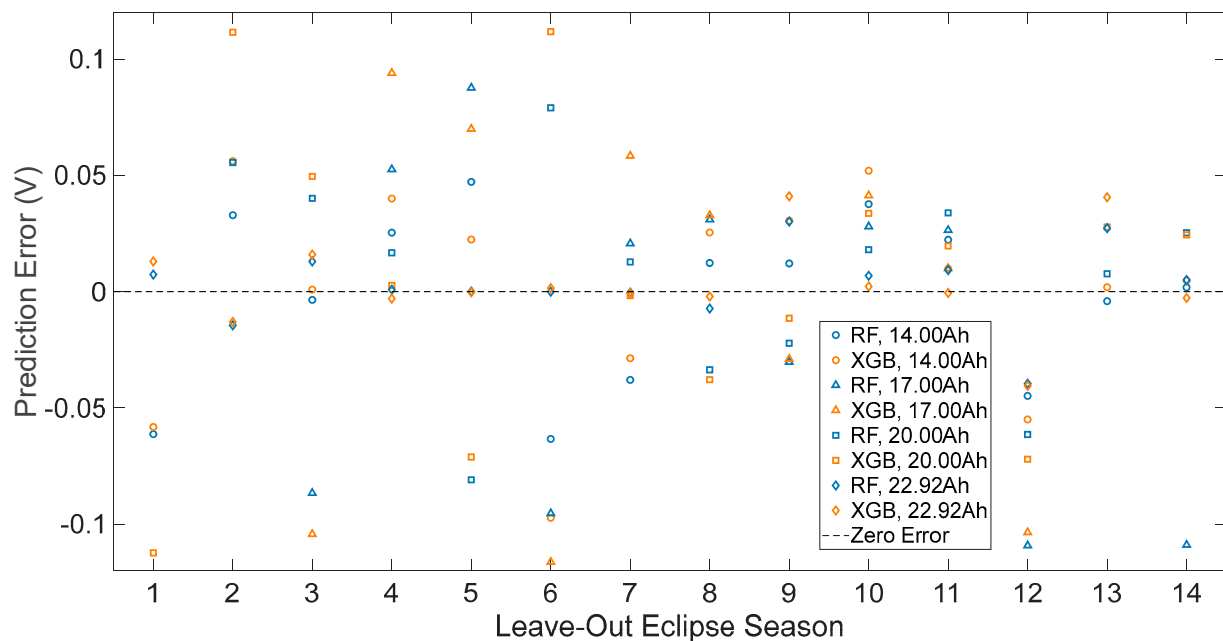
Figure 11. Leave-one-eclipse-season-out cross-validation prediction error.
