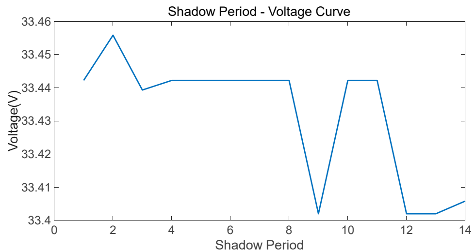
Figure 10. Trend of voltage variation with eclipse shadow period.
