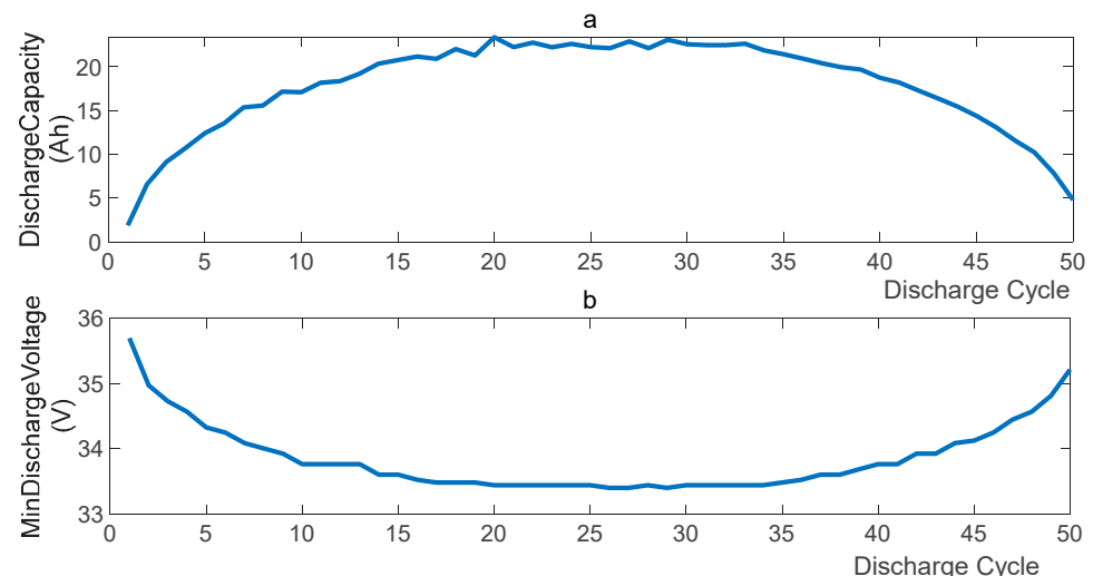
Figure 3. Discharge capacity vs. cut-off voltage and cycles (one eclipse season). (a) Discharge capacity curve, (b) Minimum discharge voltage curve.
