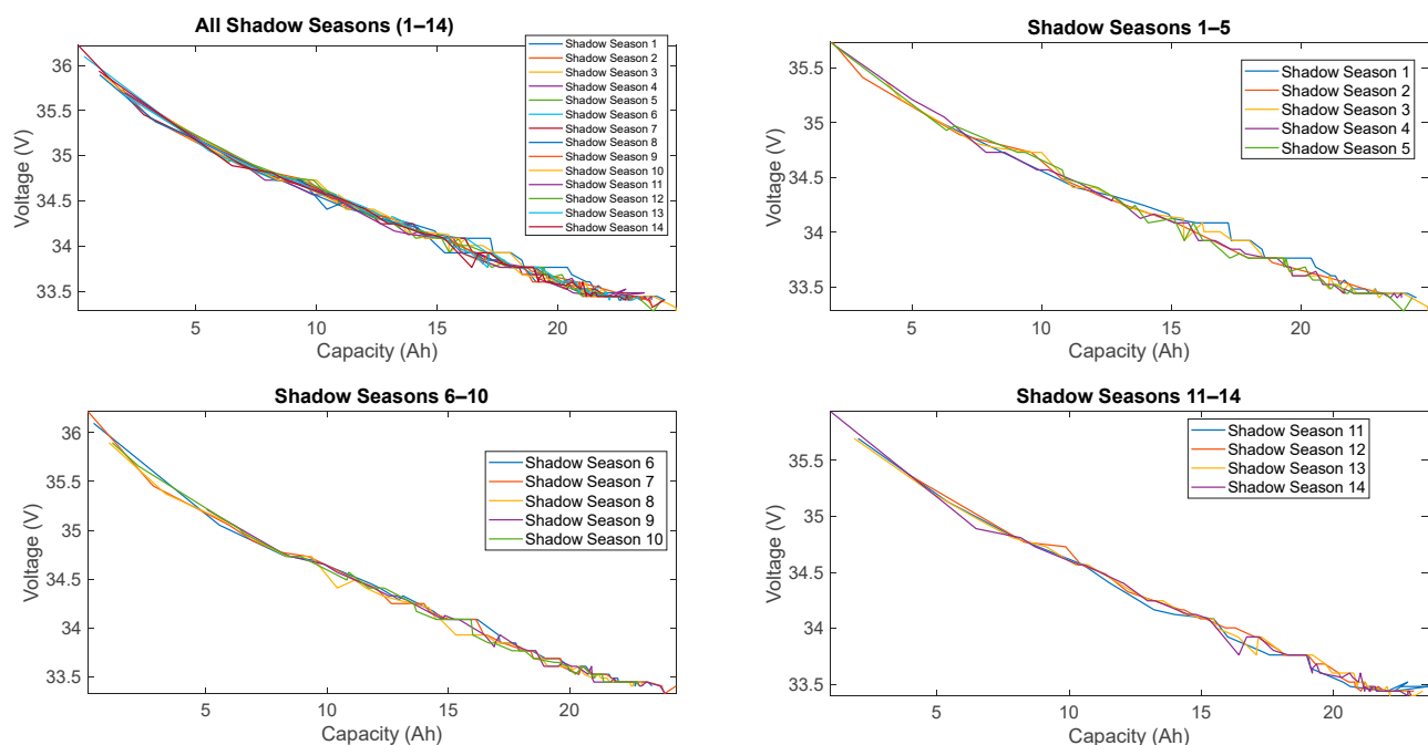
Figure 4. Battery discharge capacity vs. voltage curve.
