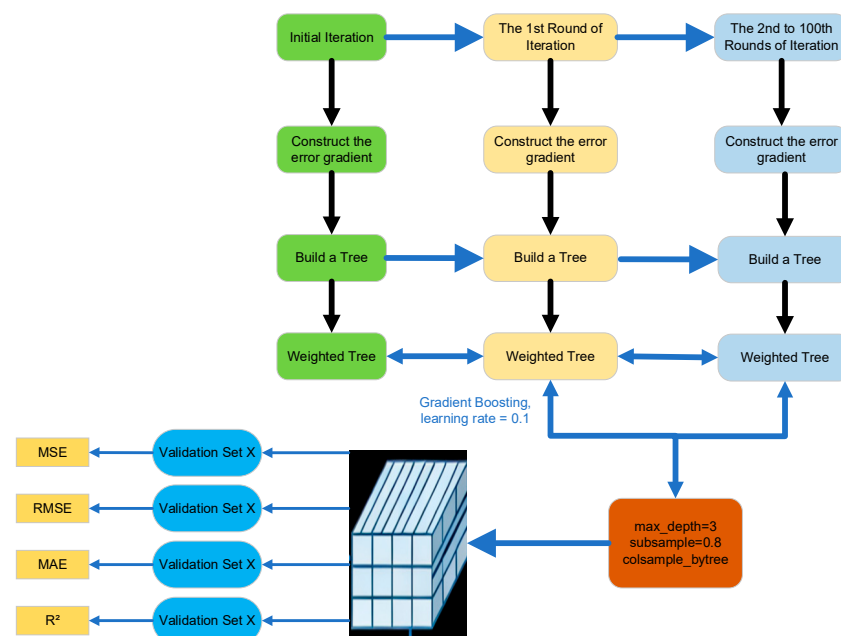
Figure 6. XGBoost algorithm-specific implementation flowchart.
