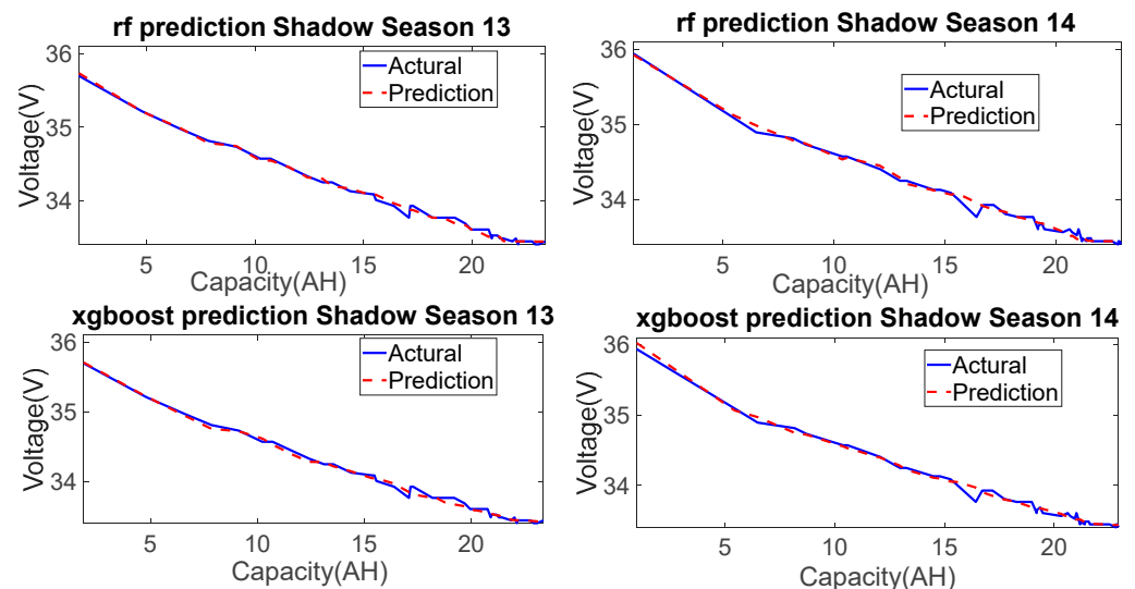
Figure 7. Prediction charts of battery voltage for shadow seasons 13–14.
