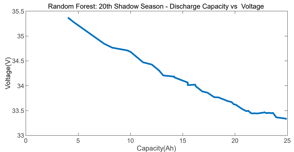
Figure 9. Relationship curve between discharge capacity and cut-off discharge voltage of satellite battery at end of 10-year service life (20th eclipse season).
