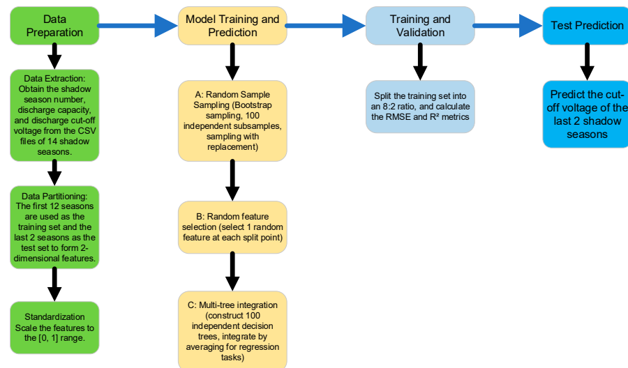
Figure 5. Random Forest algorithm-specific implementation flowchart.
