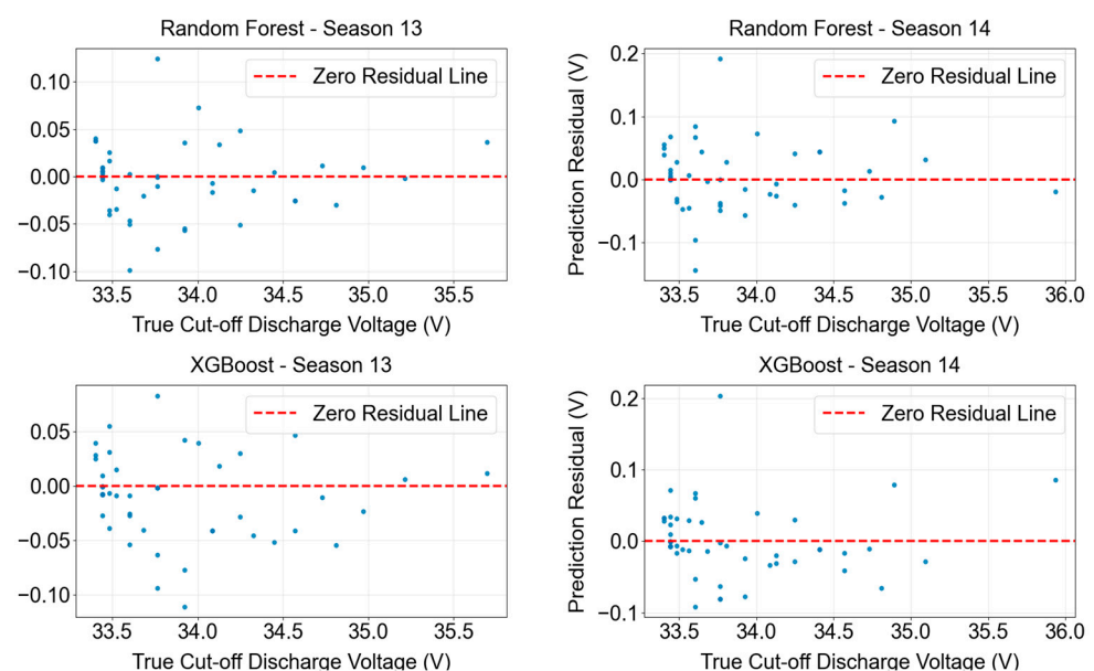
Figure 8. Residual plots under different cut-off voltages.
