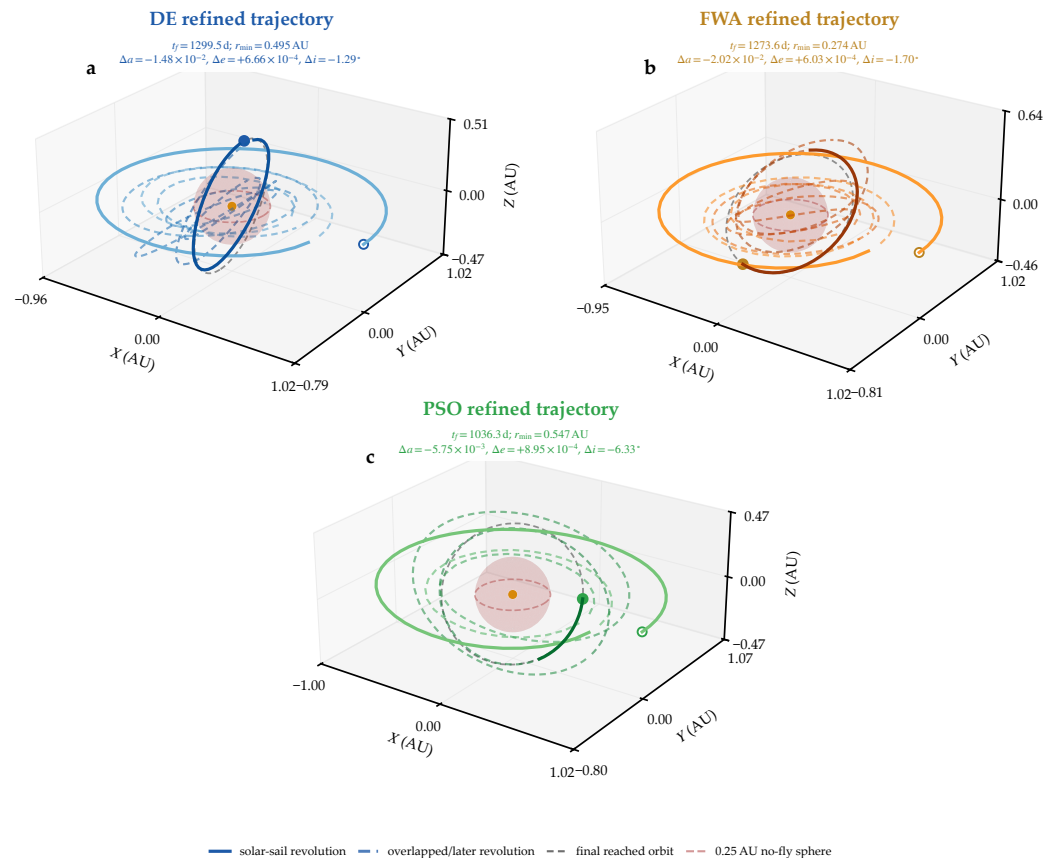
Figure 10. Case C two-stage NLP refined trajectories: (a) DE refined trajectory (blue); (b) FWA refined trajectory (orange); (c) PSO refined trajectory (green). The minimum solar distance is taken from the high-fidelity perihelion monitor used for the hard-veto safety check; the 0.25 AU thermal no-fly sphere is marked in red. Continuous curves show downsampled solar-sail revolutions; highlighted arcs indicate overlapped or later revolutions.
