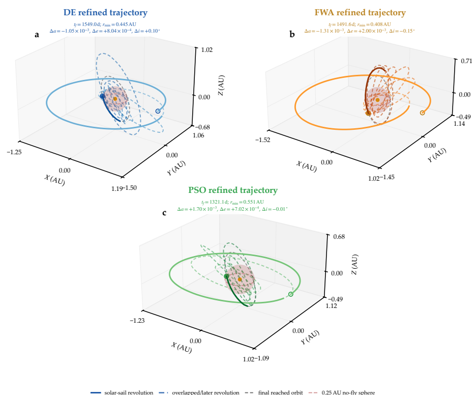
Figure 9. Case C free NLP refined trajectories. Continuous downsampled skeletons preserve the overall path, while highlighted revolutions show the key outline. (a) DE refined solution (blue); (b) FWA refined solution (orange); (c) PSO refined solution (green). Annotations report t_f , r_{\min} , and terminal errors.
