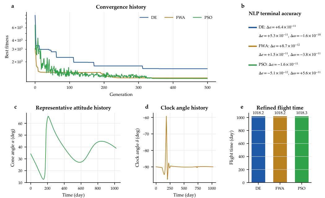
Figure 6. Case A convergence histories, representative attitude histories, terminal accuracy, and refined flight-time comparison.
