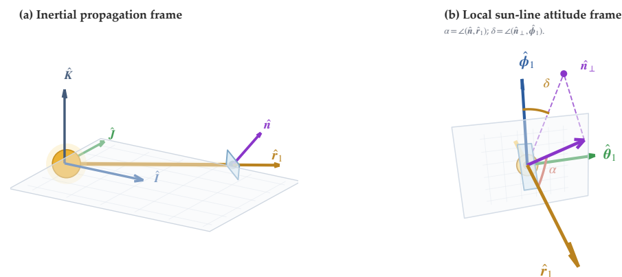
Figure 3. Sun-Line Reference Frame.
