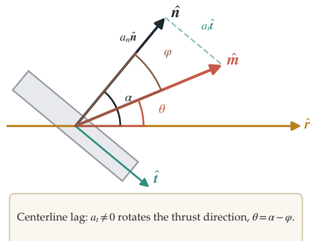
Figure 4. Non-ideal solar-sail force direction and the centerline lag between the commanded sail normal and the resultant acceleration direction.
