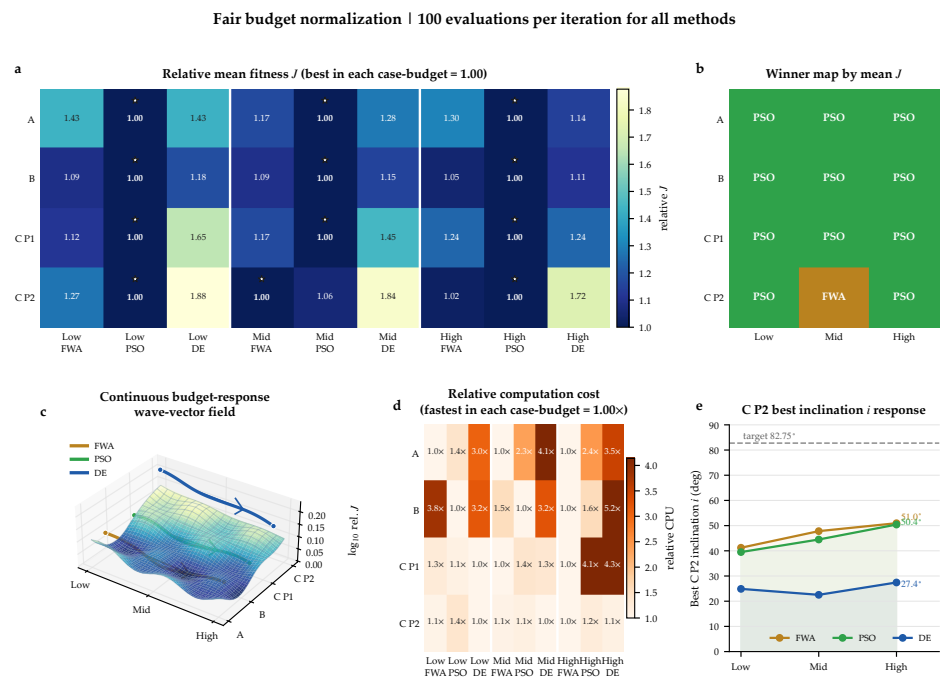
Figure 12. Fair budget-normalization summary (100 evaluations per iteration for all algorithms). (a) Relative mean fitness J , normalized so that the best algorithm in each case-budget cell equals 1.00 (marked with *); (b) winner map identifying the lowest- J algorithm per cell; (c) continuous budget-response curves showing \log_{10} relative J versus budget level; (d) relative computation cost, normalized so that the fastest algorithm in each cell equals 1.00×; (e) Case C Phase 2 terminal inclination response under deeper but narrower iterative search, with the dashed line marking the 82.75° target. Color encodes algorithm: orange for FWA, green for PSO, blue for DE.
