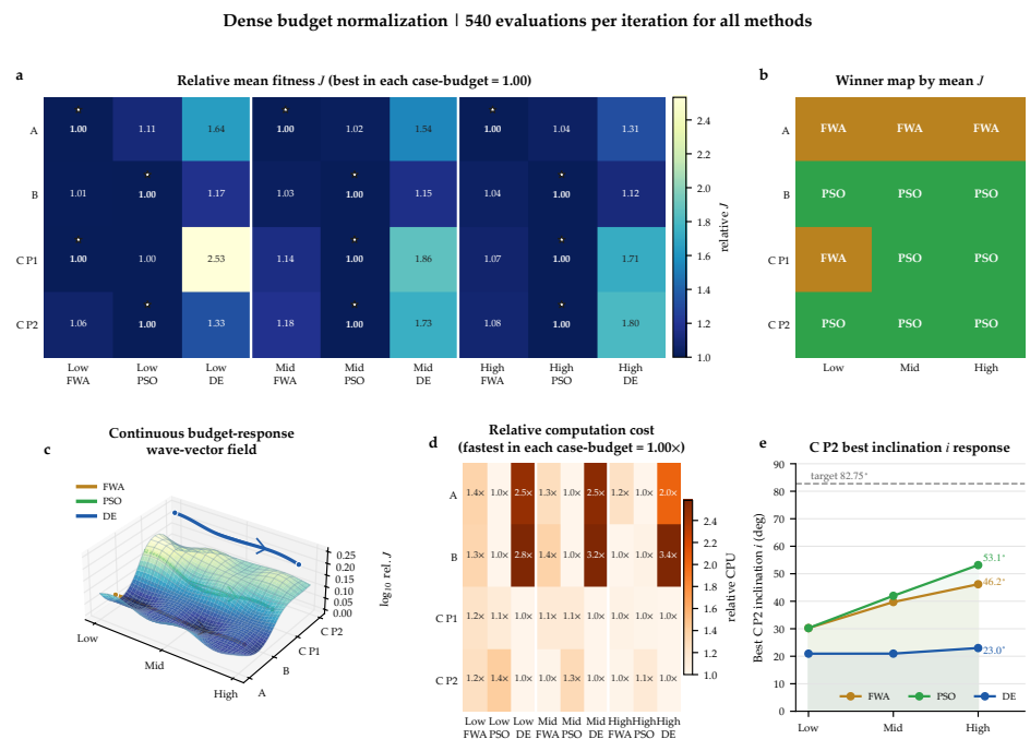
Figure 11. Dense budget-normalization summary (540 evaluations per iteration for all algorithms). (a) Relative mean fitness J , normalized so that the best algorithm in each case–budget cell equals 1.00 (marked with *); (b) winner map identifying the lowest- J algorithm per cell; (c) continuous budget-response curves showing \log_{10} relative J versus budget level; (d) relative computation cost, normalized so that the fastest algorithm in each cell equals 1.00×; (e) best Case C Phase 2 terminal inclination versus budget, with the dashed line marking the 82.75° target. Color encodes algorithm: orange for FWA, green for PSO, blue for DE.
