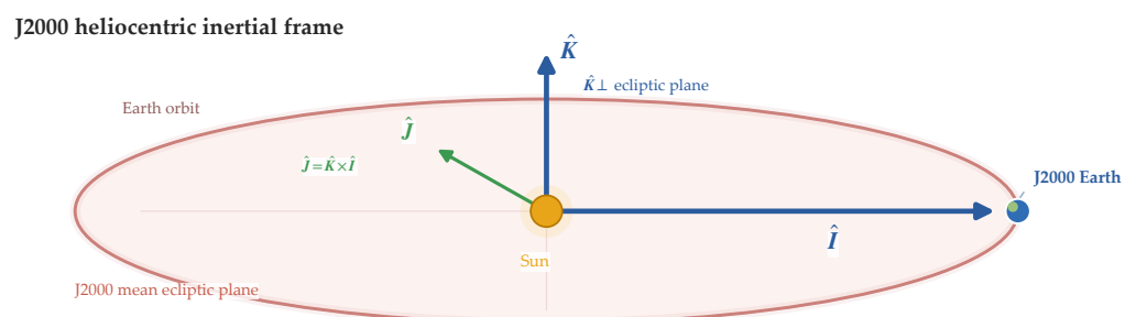
Figure 2. J2000 Heliocentric Inertial reference frame. The \hat{I} axis points toward the J2000 vernal equinox, while \hat{K} is normal to the J2000 mean ecliptic plane of Earth's orbit.
