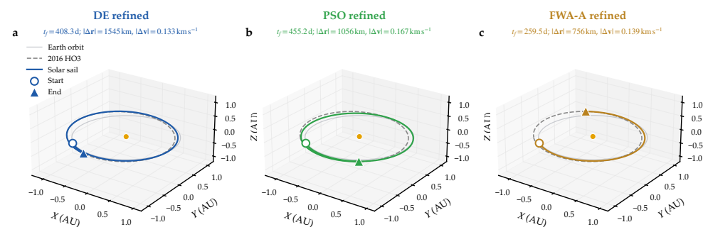
Figure 8. Case B warm-start NLP refined trajectories for DE, PSO, and the FWA Family A solution. Terminal position and velocity errors are annotated in each panel. (a) DE refined trajectory (blue); (b) PSO refined trajectory (green); (c) FWA Family A refined trajectory (orange).
