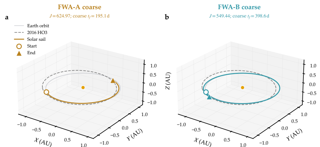
Figure 7. Case B FWA coarse-search family comparison. (a) Short-transfer Family A (orange trajectory), intercepting 2016 HO3 near its first favorable phase angle after departure; (b) longer position-accurate Family B (blue trajectory) achieving near-zero position error. The grey dashed line indicates 2016 HO3's orbit.
