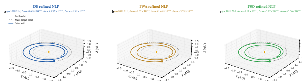
Figure 5. Case A NLP-refined solar sail trajectories. The panel annotations report refined flight time and terminal element errors in semimajor axis, eccentricity, and argument of periapsis.
