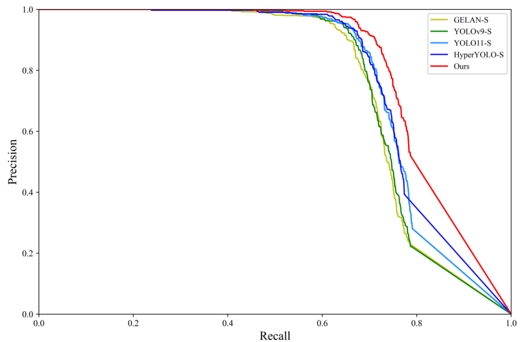
Figure 8. PR curves of GELAN-S, YOLOv9-S, YOLO11-S, HyperYOLO-S and the EWH-YOLO.
