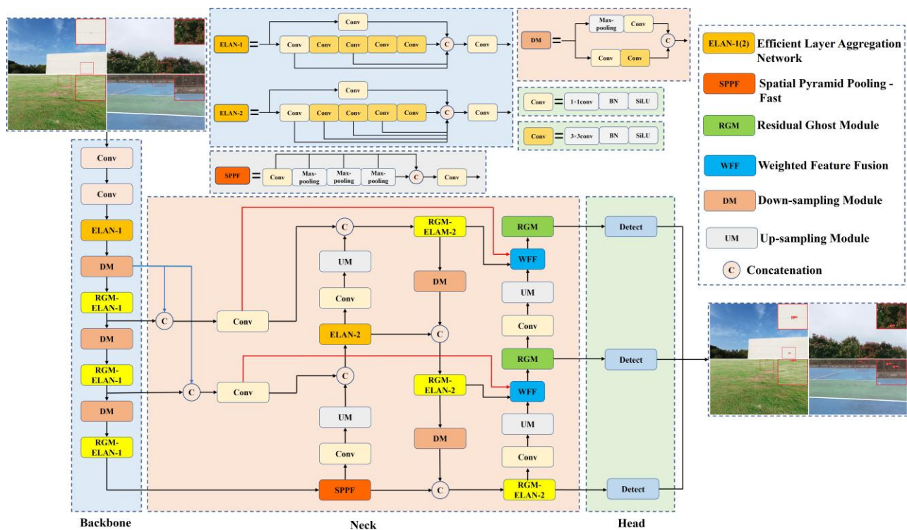
Figure 1. The overall structure of the proposed EWH-YOLO.
