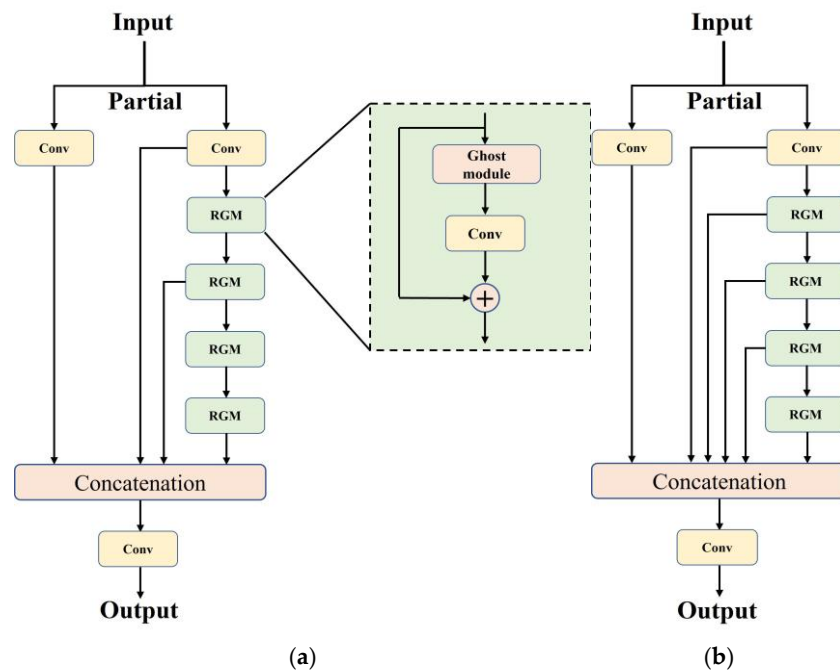
Figure 2. The detailed structure of RGM-ELAN. (a) RGM-ELAN-1. (b) RGM-ELAN-2.
