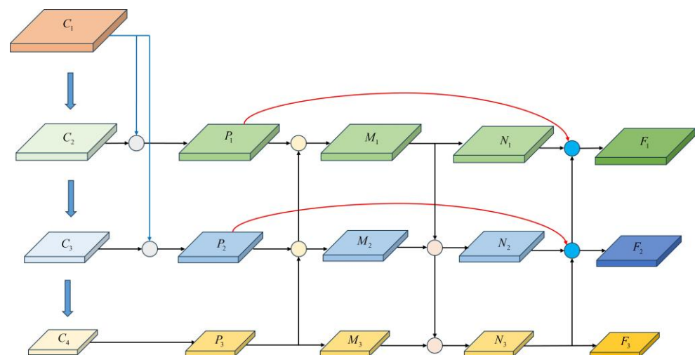
Figure 4. The detailed structure of the WBFFN.
