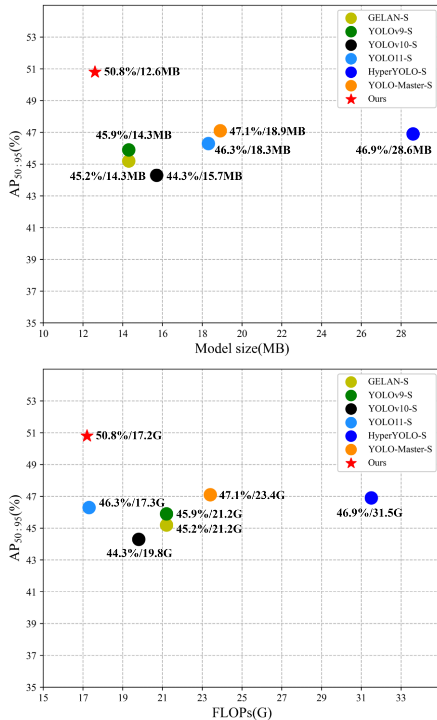
Figure 9. Comparison of AP 50:95 with parameters, model size and FLOPs.
