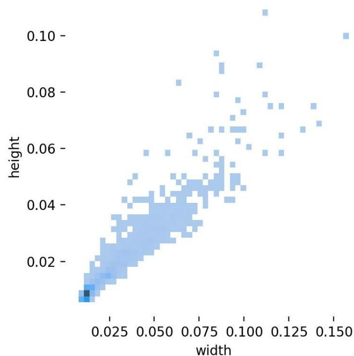
Figure 7. The object size distribution of the self-constructed dataset.
