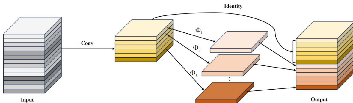
Figure 3. The detailed structure of the Ghost module.
