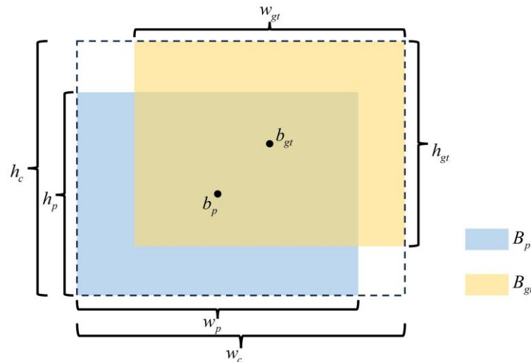
Figure 5. Illustration of EIoU loss.
