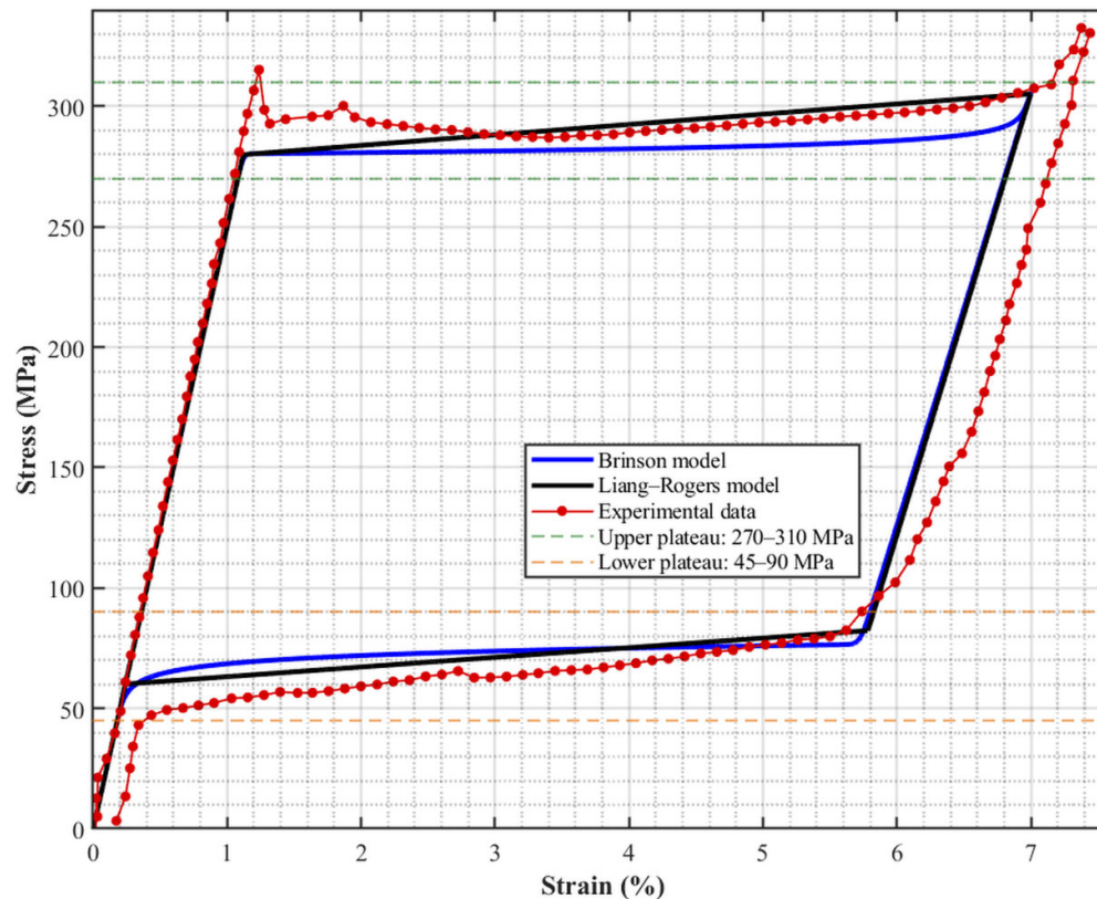
Figure 3. Comparison of experimental and numerical stress–strain responses predicted by the Brinson and Liang–Rogers constitutive models for Test 2.
