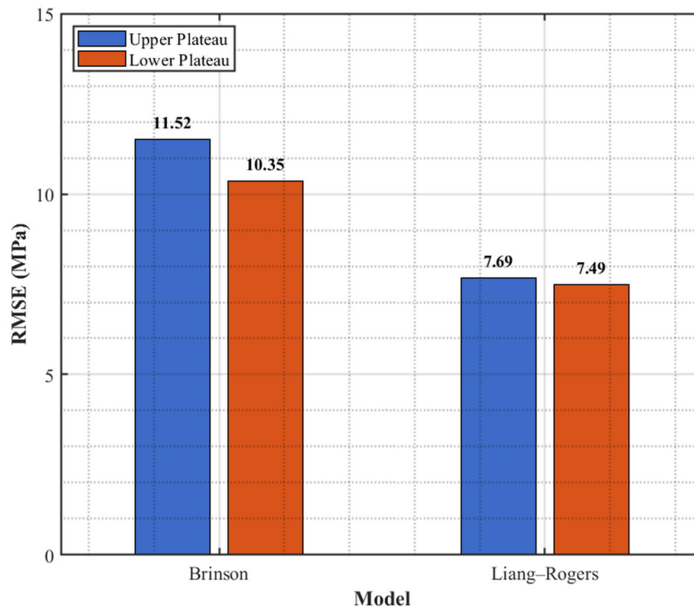
Figure 4. Comparison of localized plateau RMSE values for the Brinson and Liang–Rogers models (Test 2).
