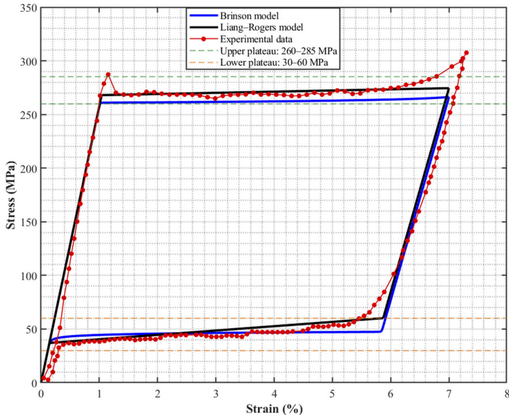
Figure 1. Comparison of experimental and numerical stress–strain responses predicted by the Brinson and Liang–Rogers constitutive models for Test 1.
