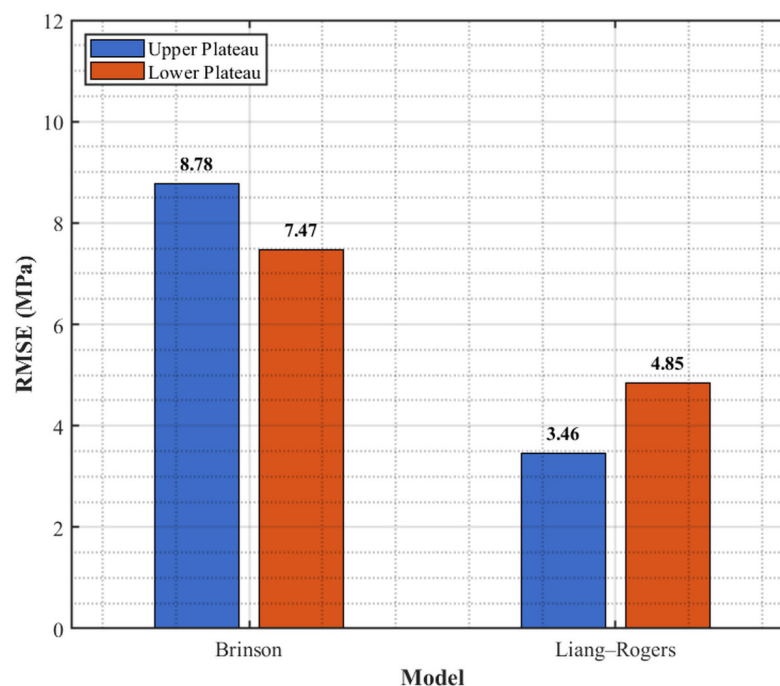
Figure 2. Comparison of localized plateau RMSE values for the Brinson and Liang–Rogers models (Test 1).
