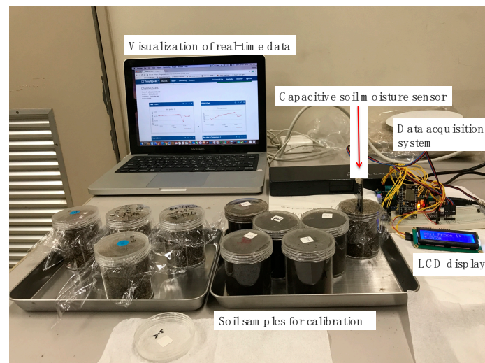
Figure 1. Acquisition and visualization of real-time data during the soil sample calibration process.
