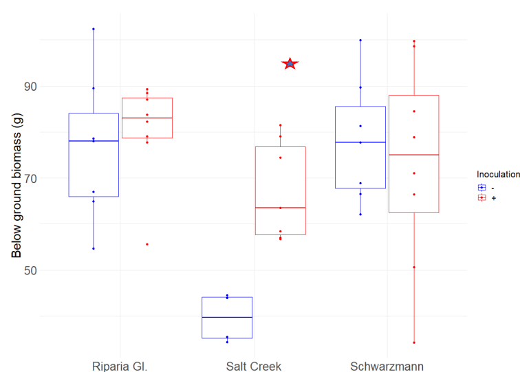
Figure 3. Below ground biomass (grams) of grapevine rootstocks after two years of field cultivation. Blue plots represent uninoculated while red plots represent inoculated rootstocks. Red stars above inoculated plots depict significant positive AM fungal response compared to uninoculated control. Statistical analysis was performed on the log scale.
