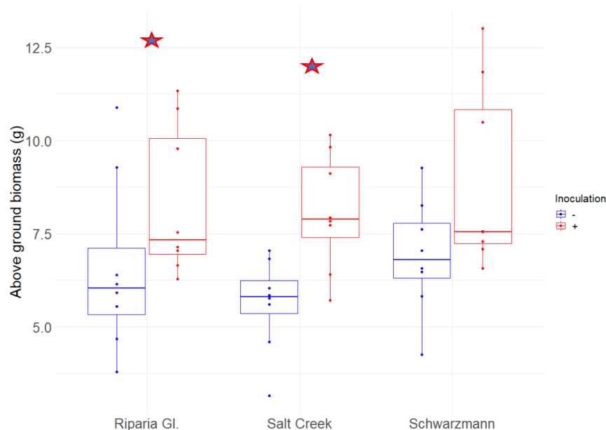
Figure 1. Above ground biomass (grams) of greenhouse-grown rootstocks during the first year. Blue plots represent uninoculated while red plots represent inoculated rootstocks. Red stars above inoculated plots depict significant positive AM fungal response compared to uninoculated control. Statistical analysis was performed on the log scale.
