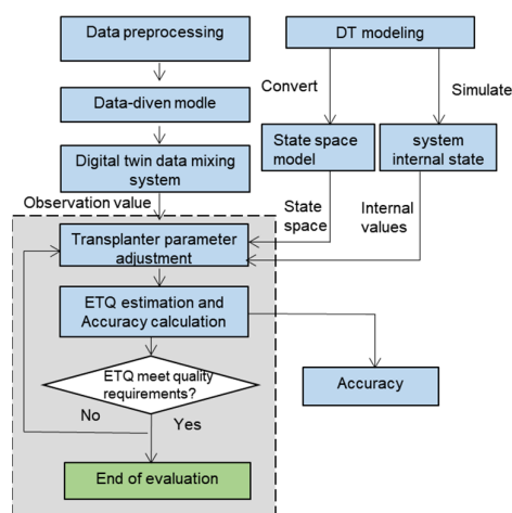
Figure 10. DT-based and data-driven hybrid approach steps.
