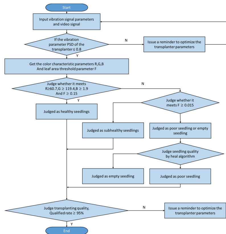
Figure 12. Hybrid evaluation method of PFT transplanting effect.
