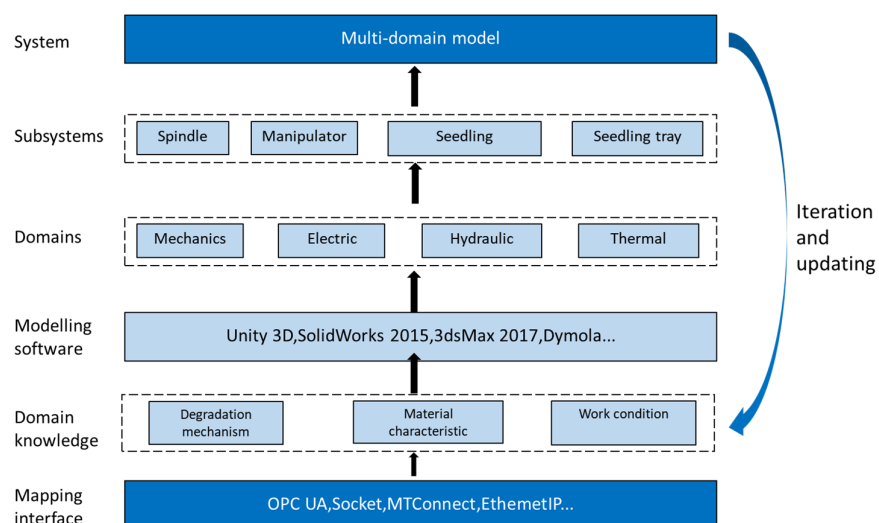
Figure 3. Implementation of the multi-domain model.
