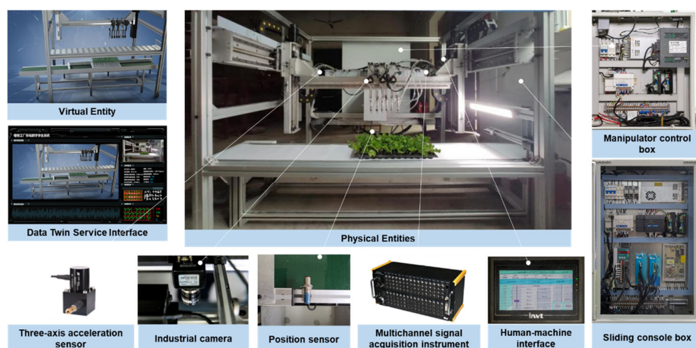
Figure 5. Overall design of PFT digital twin experiment platform.
