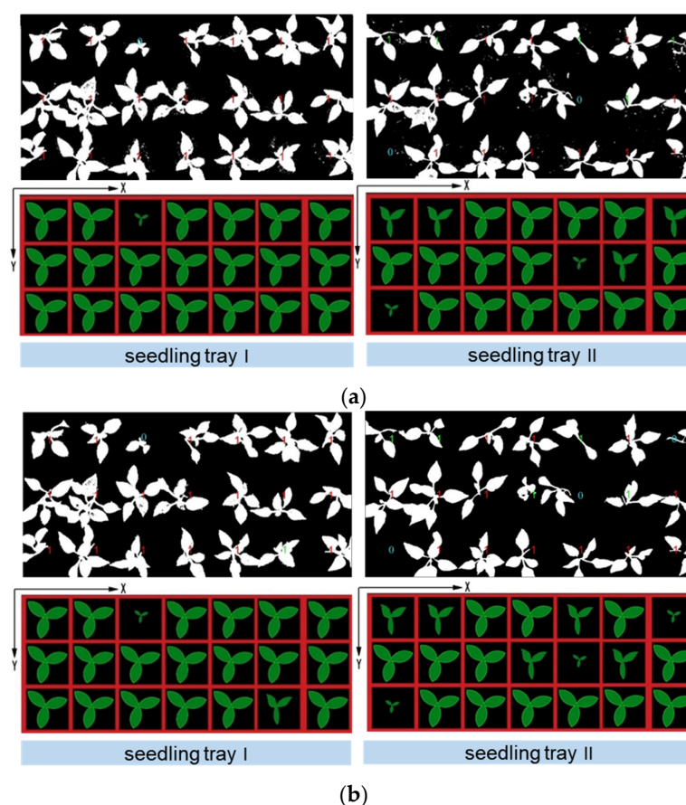
Figure 16. Virtual mapping reproduction of digital twin seedling tray. (a) Bowl seedling classification and digital twin Mapping based on traditional Wiener Algorithm. (b) Bowl seedling classification and digital twin mapping based on 3D block matching filtering algorithm.
