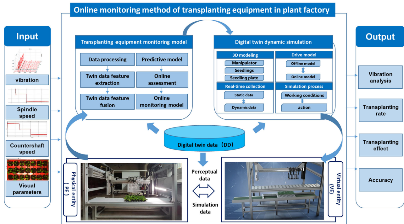
Figure 2. A digital twin-based hybrid approach to monitoring and maintenance framework.
