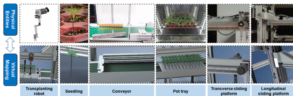
Figure 6. Construction of the virtual entity model.
