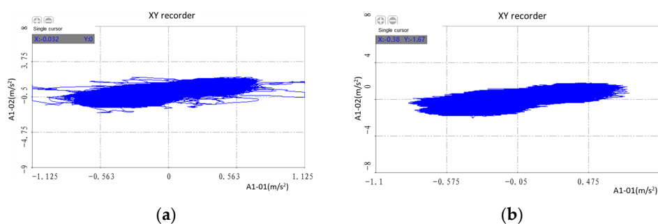
Figure 9. Elimination of trends using polynomials of different orders. (a) Raw data signal. (b) Signal after removing trend term.
