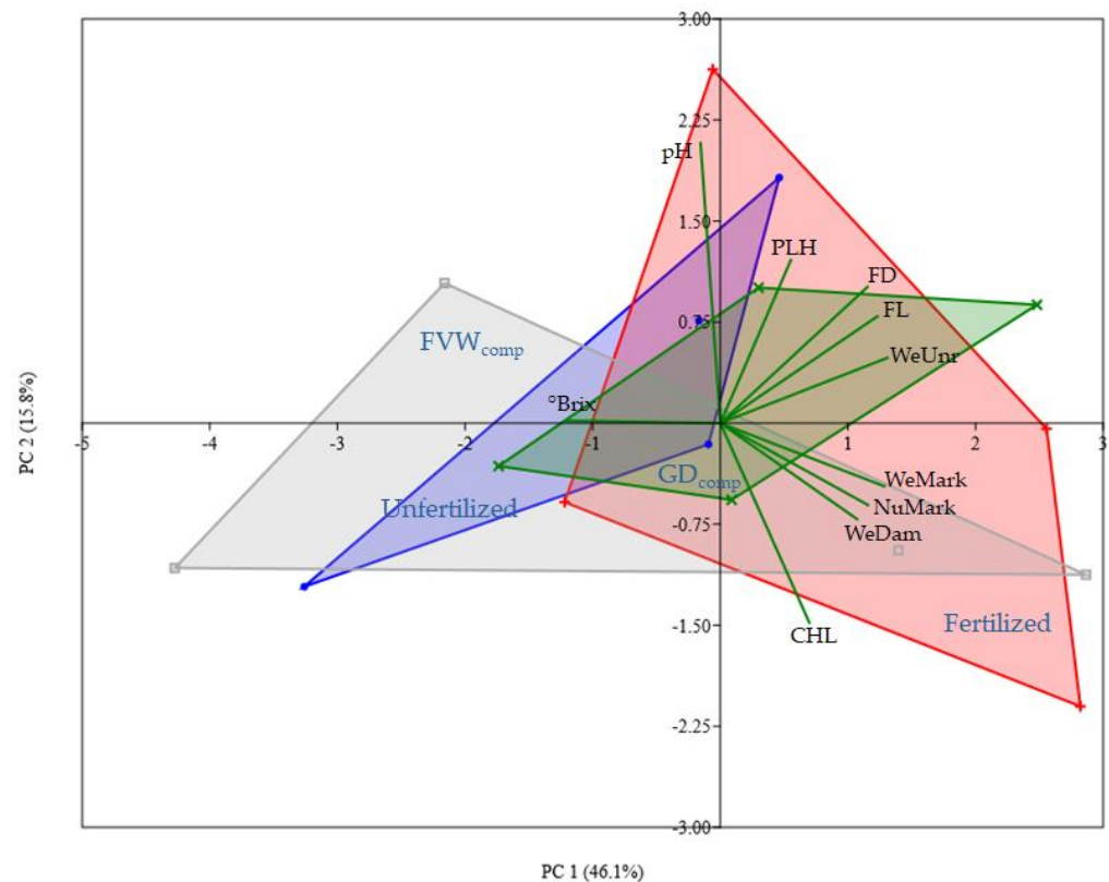
Figure 8. Biplot showing the PCA results of treatment separation based on the observed traits. °Brix (soluble solids); CHL, chlorophyll content; FD, fruit diameter; FL, fruit length; NuMark, number of marketable fruits per plant; PLH, plant height; WeMark, weight of marketable fruits per plant; WeUnr, weight of unripened fruits per plant; WeDam, weight of damaged fruits per plant. Polygon colors: purple, Unfertilized; pink, Fertilized; green, GD comp , compost from Gainesville diet; grey, FVW comp , compost from fruit and vegetable waste.
