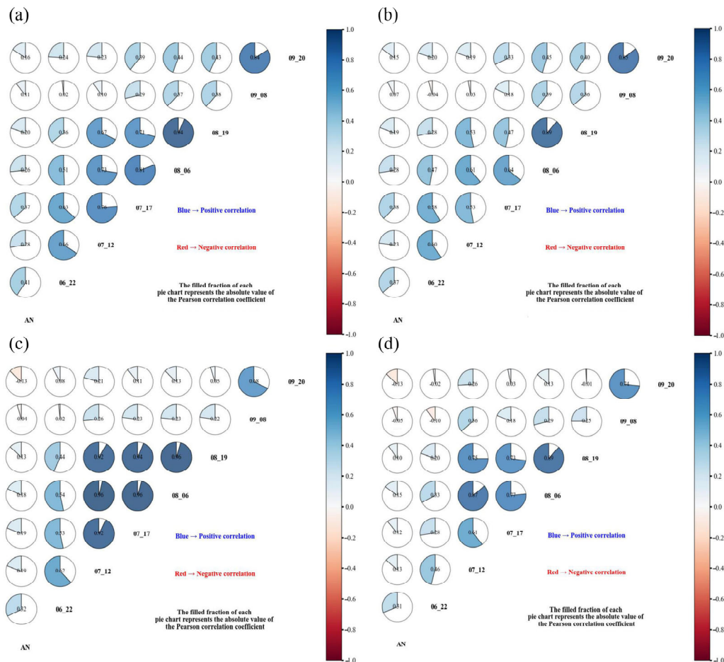
Figure A1. The correlation between variables. Soybean Plantations: (a) NDVI; (b) EVI. Maize Plantations: (c) NDVI; (d) EVI.
