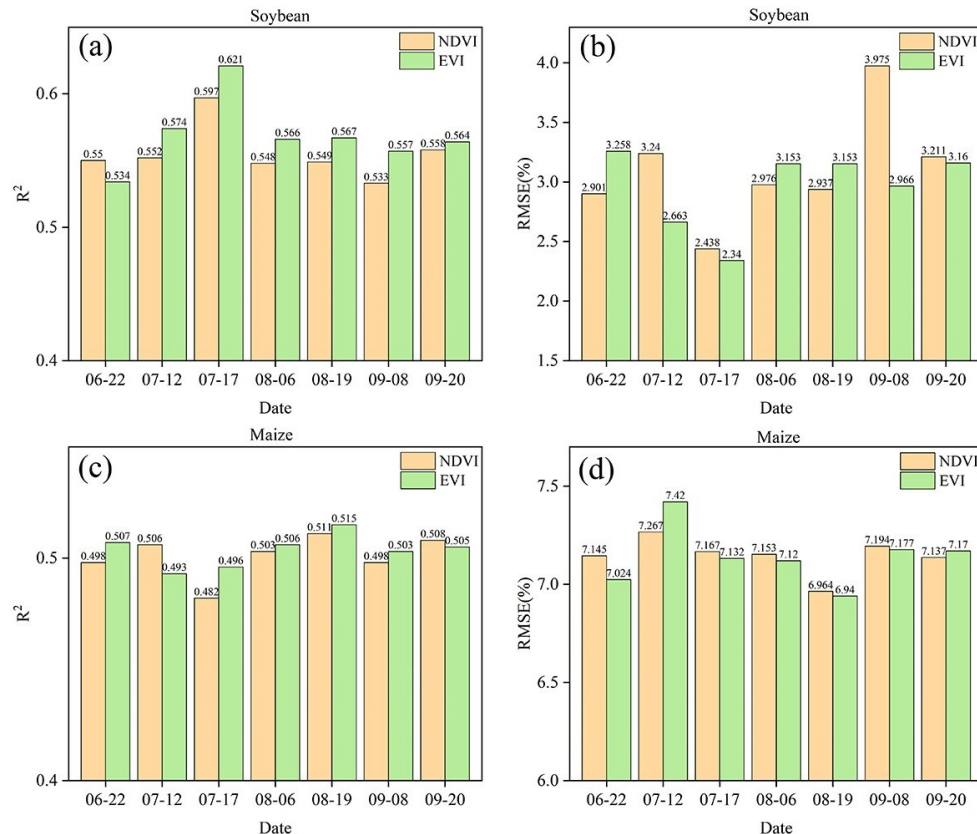
Figure 7. AN mapping accuracy of soybean and maize plantations based on remote sensing imagery, introducing growth information at different growth periods. (a,b) Soybean plantations, (c,d) maize plantations.
