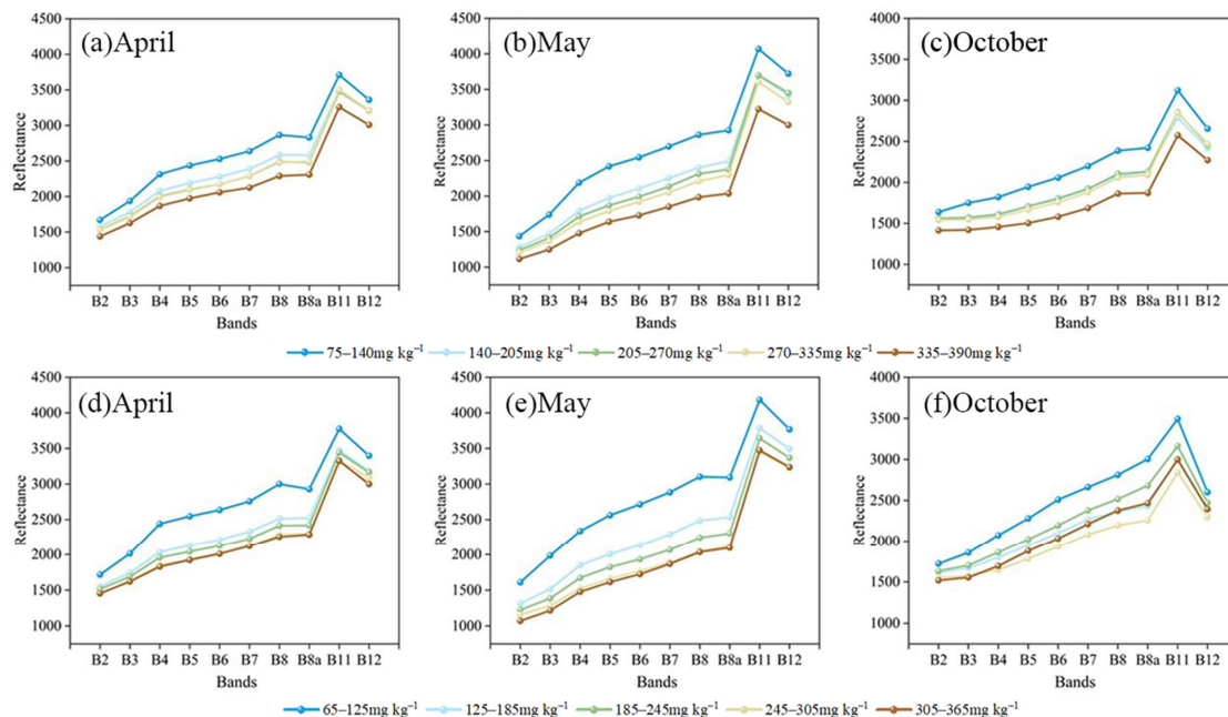
Figure 5. Soil spectral reflectance of Sentinel-2 satellite for different crop bare soil periods ((a–c) for soybean plantations and (d–f) for maize plantations).
