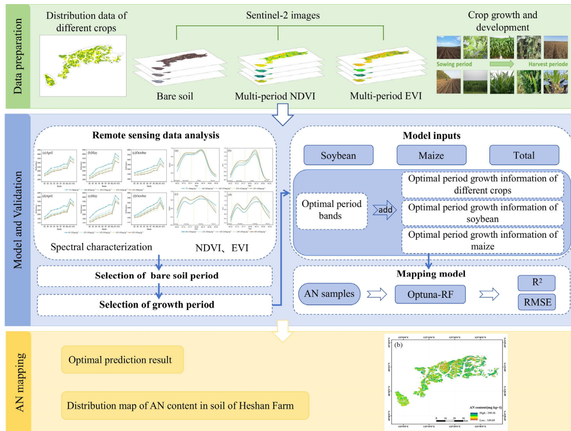
Figure 4. Technology roadmap for mapping soil AN content.
