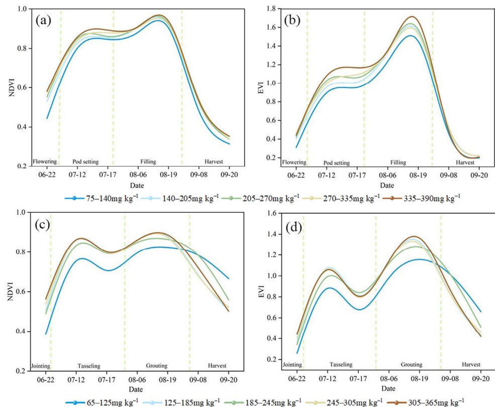
Figure 6. (a,b) NDVI and EVI time series curves for soybean plantations; (c,d) NDVI and EVI time series curves for maize plantations.
