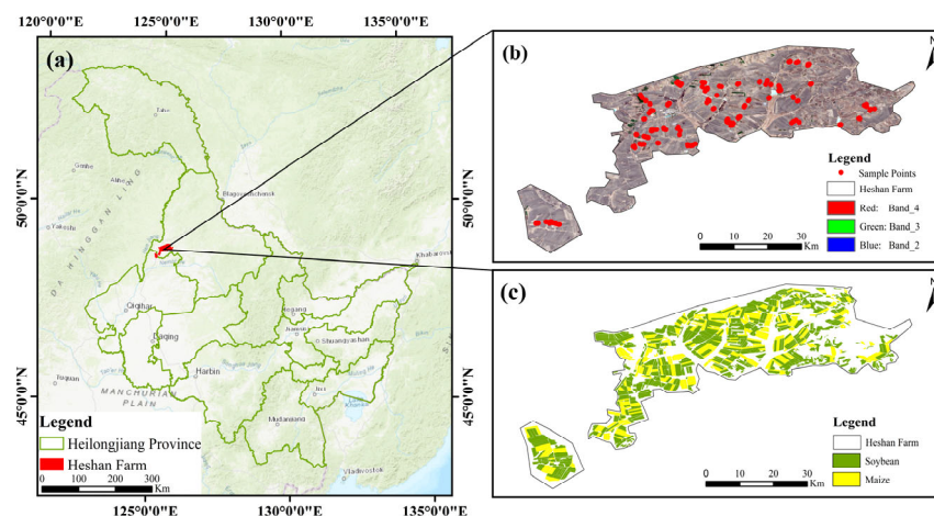
Figure 1. Overview of the study area. (a) Location map of the study area, (b) Sentinel-2 multispectral image and location of sampling points in the study area, and (c) distribution of planting structures in the study area.
