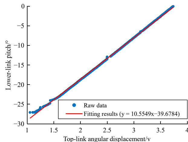
Figure 10. Correlation between AD value of top-link angular displacement and lower link pitch.
