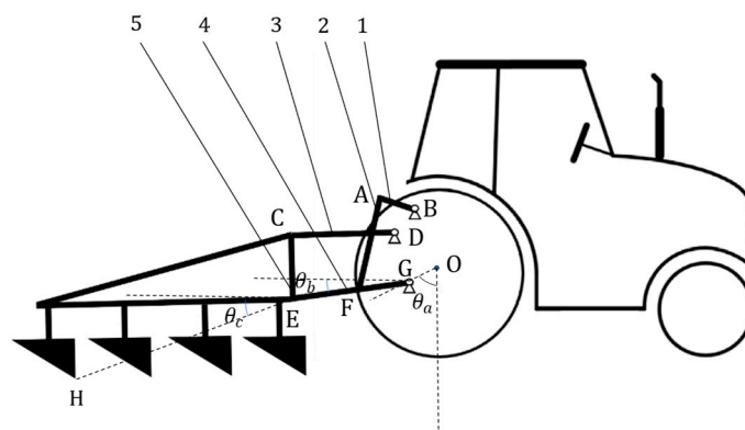
Figure 3. Projection of the three-point hitch adjustment process. 1. Upper lift arm; 2. lift rod; 3. upper link; 4. lower link; 5. plough frame.
