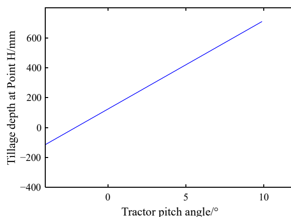
Figure 8. Correlation between tractor pitch angle and tillage depth.
