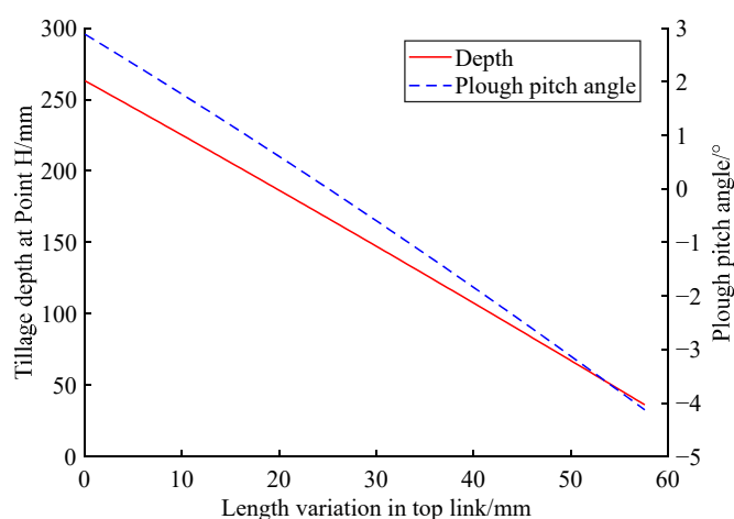
Figure 7. Correlation of top-link length variation with tillage depth and implement pitch.
