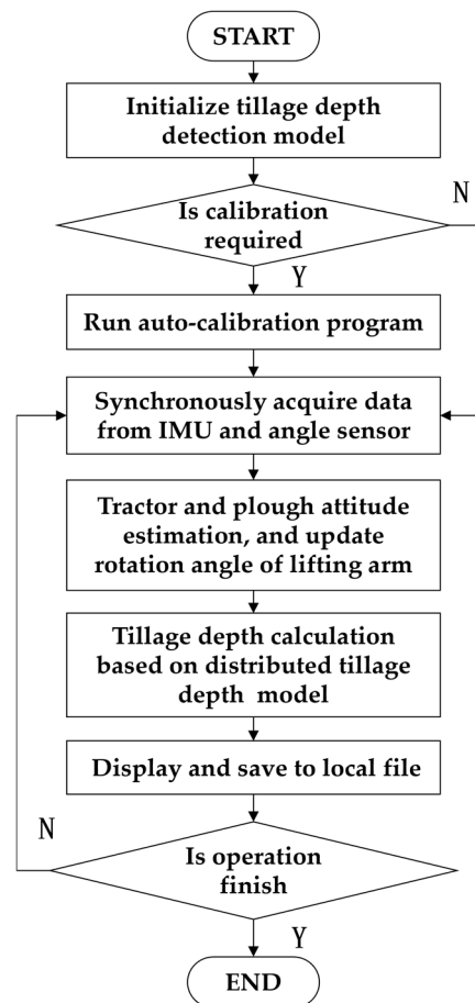
Figure 2. The flowchart of distributed tillage depth detection.
