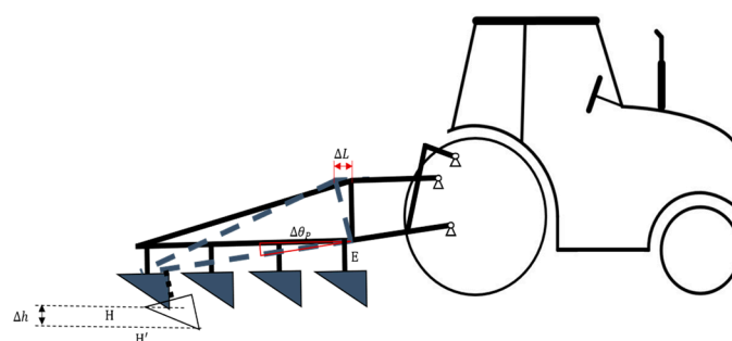
Figure 4. Projection of the top link adjustment process.
