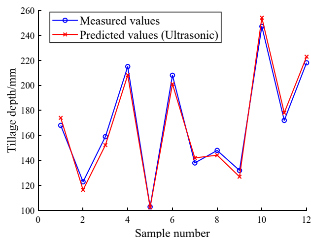
Figure 13. Results of ultrasonic-calculated tillage depth.
