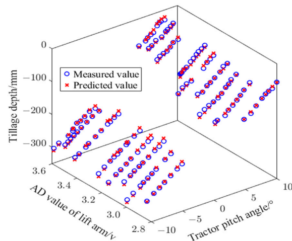
Figure 11. Results of distributed tillage depth model calibration.
