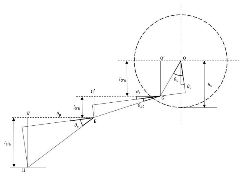
Figure 9. Simplification of the tillage depth detection linkage.
