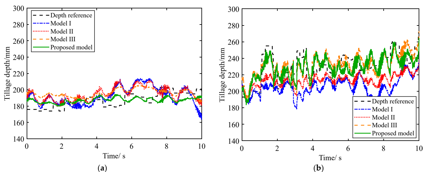
Figure 15. Results of different tillage depth models. (a) Flat farmland, and (b) bumpy farmland.
