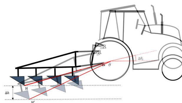
Figure 4. Projection of the top link adjustment process.
