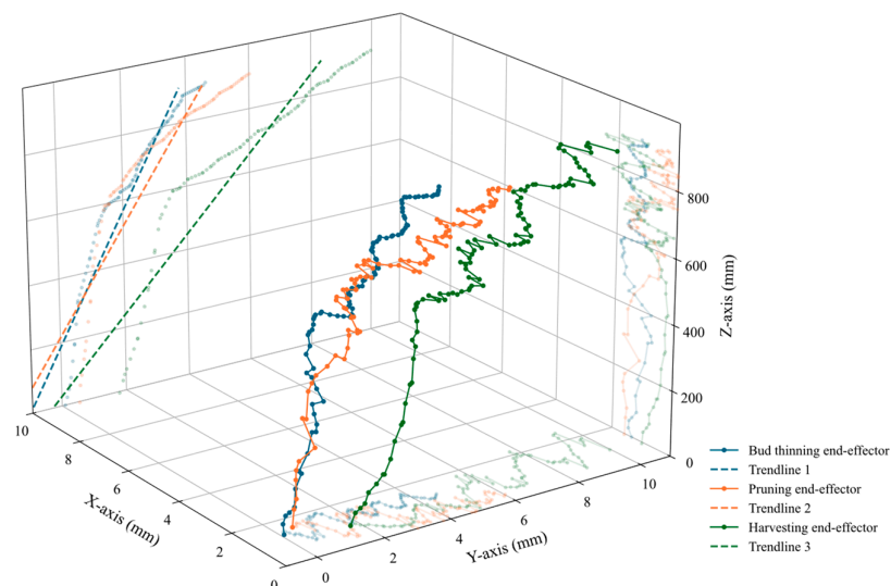
Figure 9. Three-dimensional motion trajectories of the telescopic manipulator during the extension process under varying end-effector loads. For each payload condition, the displayed trajectory was
