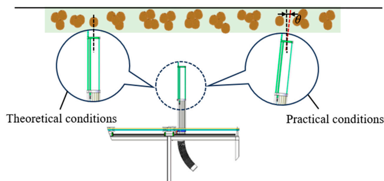
Figure 4. Structural deflection of the telescopic manipulator during vertical extension. The left side displays the theoretical conditions with perfect vertical alignment. The right side illustrates the practical conditions. The symbol \theta denotes the actual deflection angle caused by structural bending.
