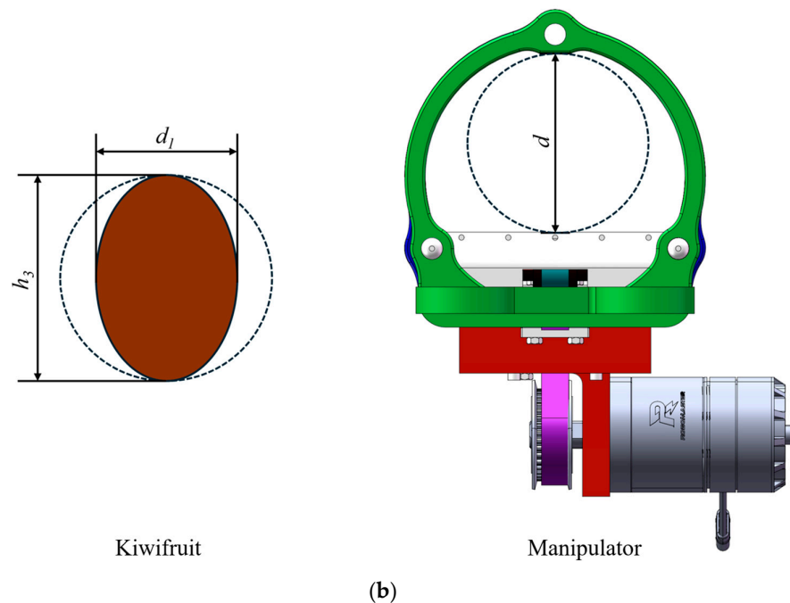
Figure 3. Dimensional design and spatial constraint analysis of the telescopic manipulator. (a) Vertical spatial constraints of the Cartesian mechanism operating under the kiwifruit hanging zone. (b) Dimensional matching between kiwifruit geometric parameters and the hollow manipulator.
