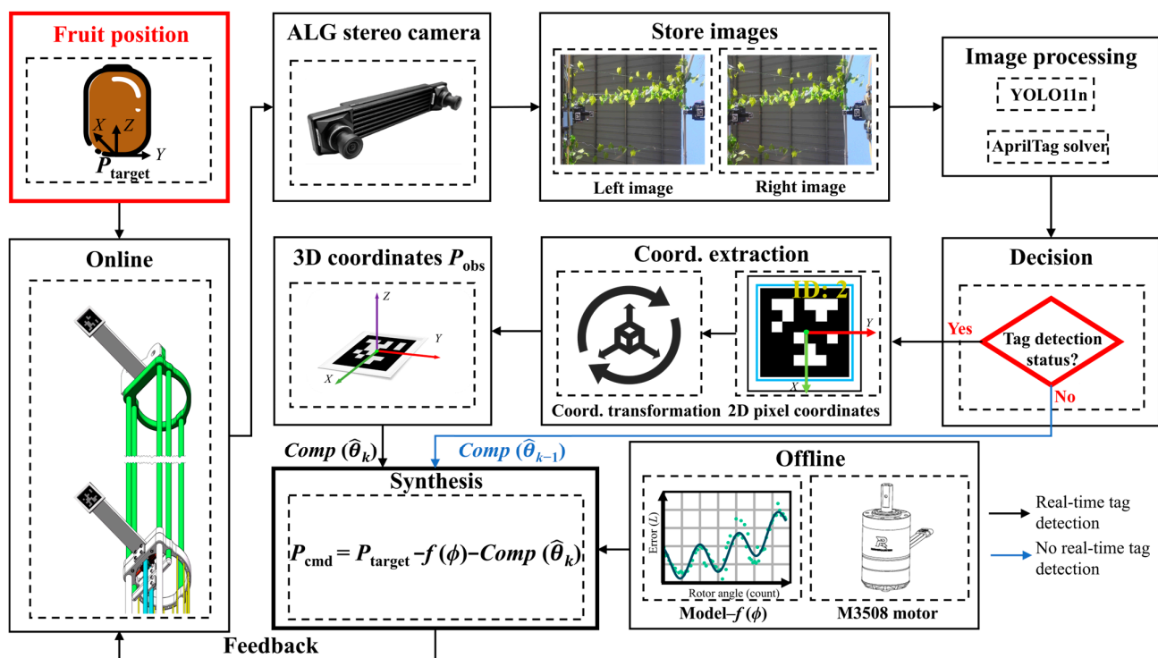
Figure 8. The proposed hybrid adaptive control architecture. It integrates an offline polynomial–Fourier feedforward model for static error compensation and a real-time visual feedback loop driven by YOLO11n and AprilTag methods to handle dynamic disturbances.
