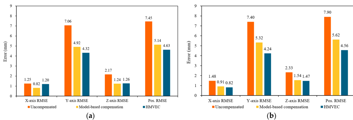
Figure 13. RMSE-based comparative analysis of positioning accuracy under different compensation strategies for the (a) left and (b) right manipulators, illustrating both individual-axis errors and overall positioning error.
