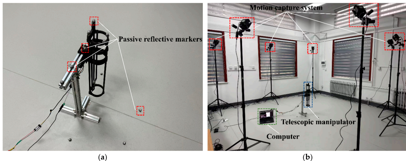
Figure 5. Experimental setup for kinematic trajectory acquisition. (a) The telescopic manipulator instrumented with passive reflective markers for pose tracking. (b) Global layout of the Mars 1.3H optical motion capture system environment, the system consists of a host computer, a telescopic manipulator, and seven optical cameras.
