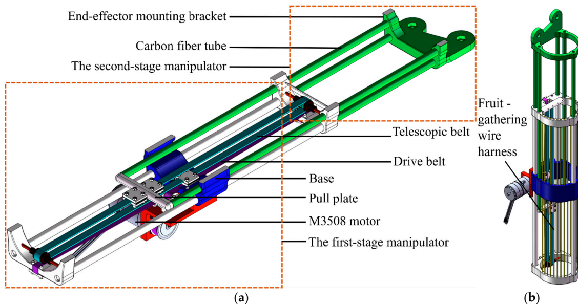
Figure 2. Hollow telescopic manipulator design. (a) Belt-driven cascaded mechanism with labeled components. The drive belt extends the first-stage manipulator while the constrained telescopic belt simultaneously extends the second-stage manipulator, achieving 1.83:1 kinematic ratio. (b) Overall structure of the telescopic manipulator.
