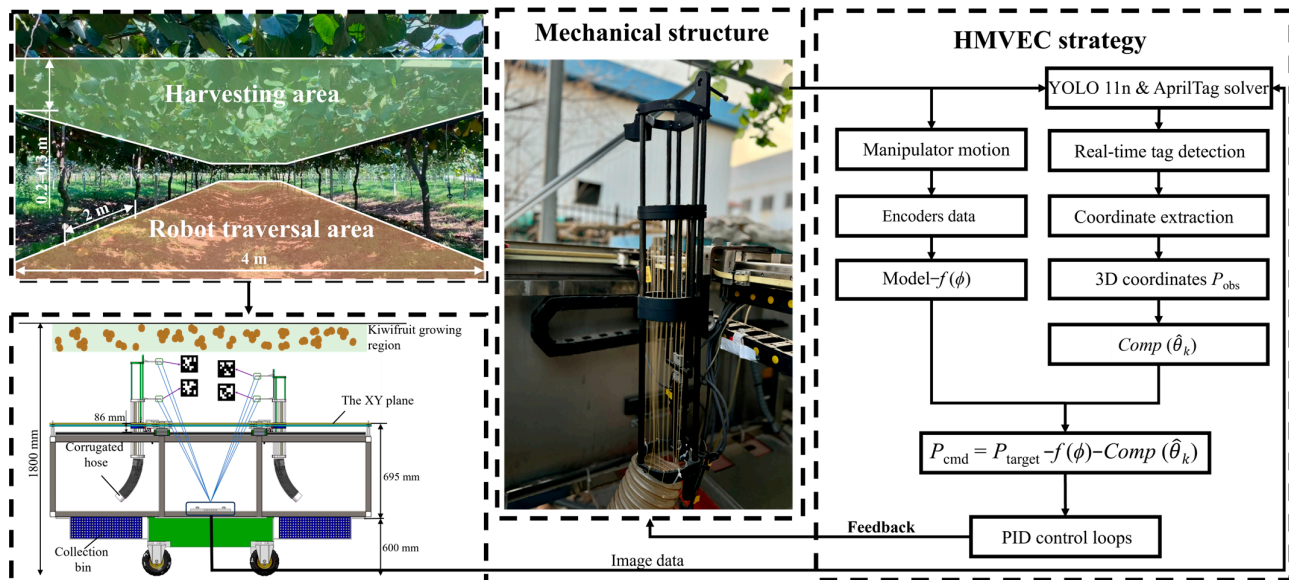
Figure 1. Overall architecture of the telescopic manipulator system for terminal positioning-error compensation and post-detachment fruit transfer in trellis-grown kiwifruit harvesting. The top-left panel illustrates the spatial constraints of the standardized kiwifruit trellis environment. The bottom-left schematic details the hardware integration, including the mobile platform and the binocular stereo vision system. The central photograph displays the physical prototype of the hollow telescopic manipulator. The right panel presents the control flowchart of the hybrid model–vision error compensation (HMVEC) strategy.
