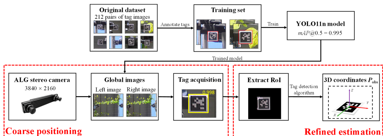
Figure 7. Two-stage detection module workflow. YOLO11n detection was used to acquire the RoI while the AprilTag detection processed the extracted tag pair to estimate the refined position.
