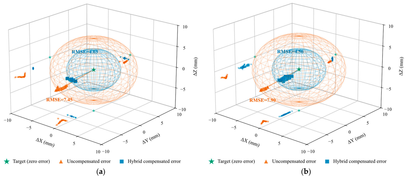
Figure 14. Three-dimensional distributions of positioning errors of the (a) left and (b) right manipulators under uncompensated and hybrid predictive compensated conditions, where RMSE spheres represent the overall error magnitude and visualize the reduction of positioning errors after compensation.
