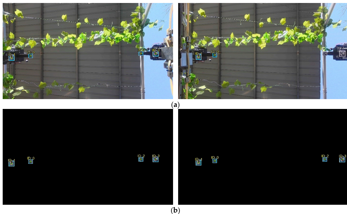
Figure 11. Comparative evaluation of AprilTag detection performance. (a) Traditional direct tag detection methods. (b) The proposed coarse-to-fine detection method. This strategy integrates the YOLO11n model for initial RoI extraction (coarse), followed by precise tag localization within the cropped bounding box (fine).
