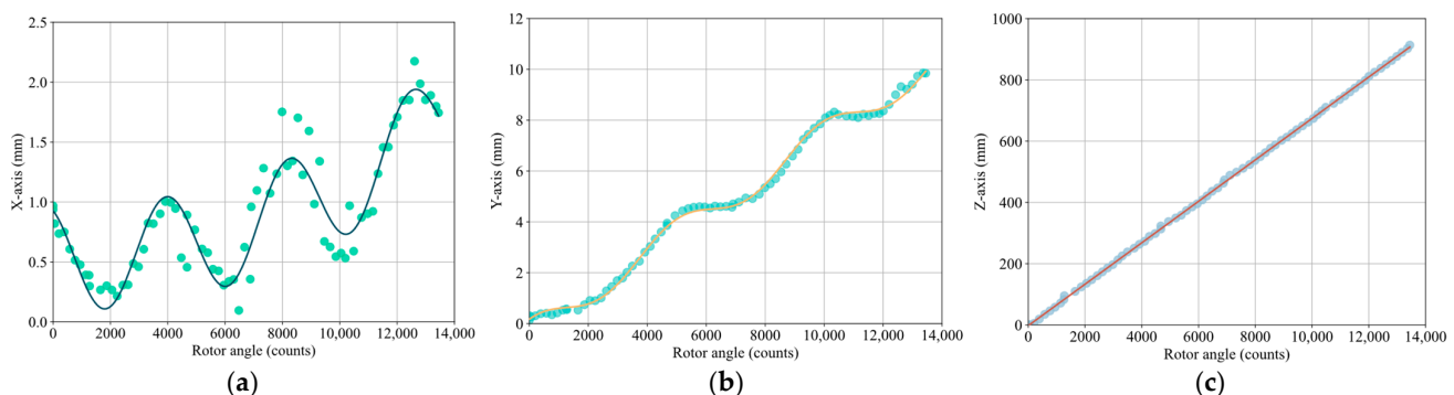
Figure 10. Regression analysis of the relationship between the 3D pose of the harvesting manipulator’s end-effector and the motor rotor angle. (a) X-axis displacement, showing the lateral oscillation trend and the fitted polynomial–Fourier curve; (b) Y-axis displacement, showing the nonlinear deflection trend mainly caused by gravitational loading and the fitted polynomial–Fourier curve; and (c) Z-axis displacement, showing the approximately linear extension trend and the fitted linear curve.
