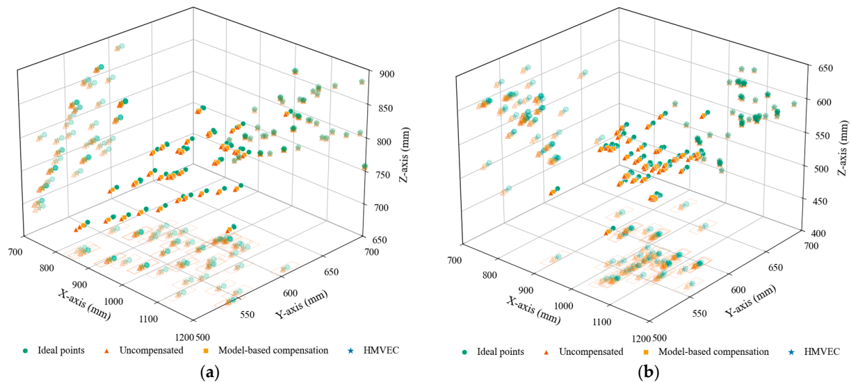
Figure 12. Comparison of 3D trajectories of the manipulator end point under different compensation strategies for the (a) left and (b) right manipulators.
