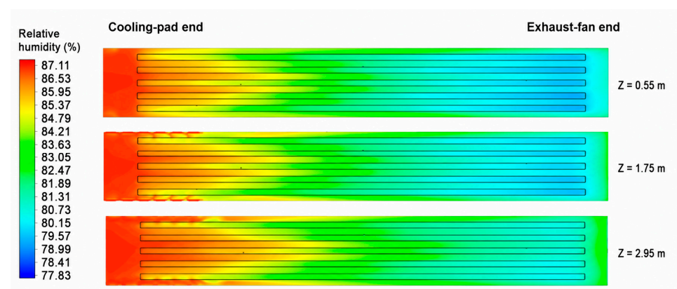
Figure 15. Relative humidity field at different heights.
