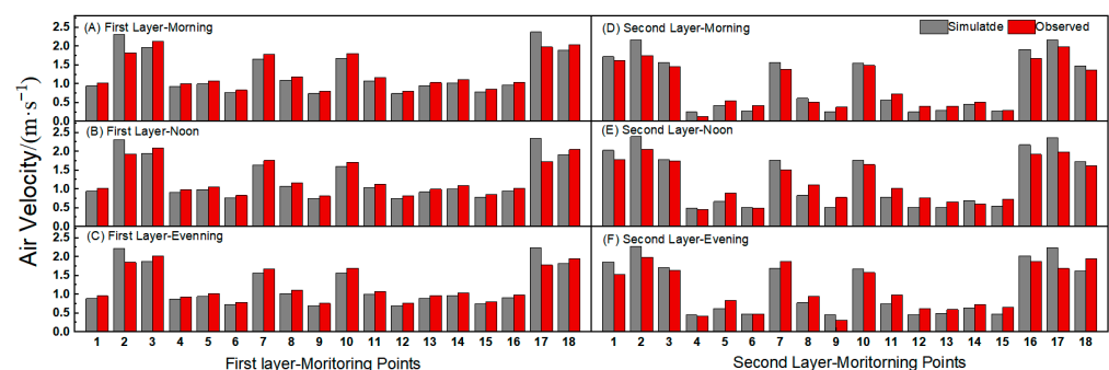
Figure 10. Comparison of simulated and measured air velocities at the monitoring locations.
