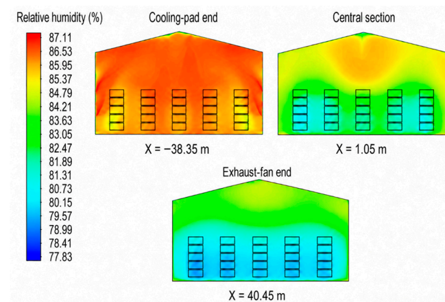
Figure 14. Relative humidity fields at different distances.
