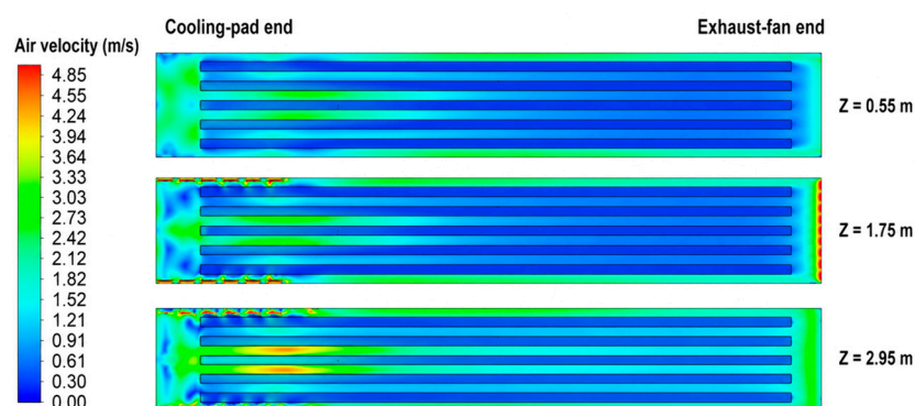
Figure 17. Wind speed fields at different heights.
