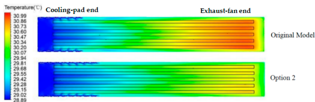
Figure 20. Comparison diagram of temperature field.
