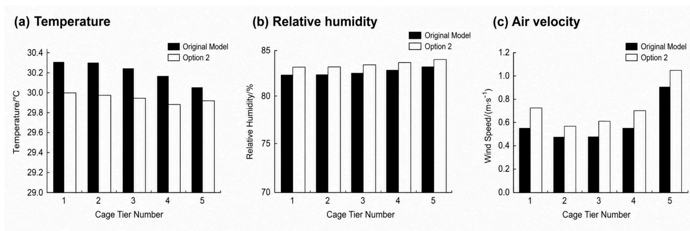
Figure 24. Comparison of cage-tier environmental variables before and after parameter optimization: (a) temperature, (b) relative humidity, and (c) air velocity.
