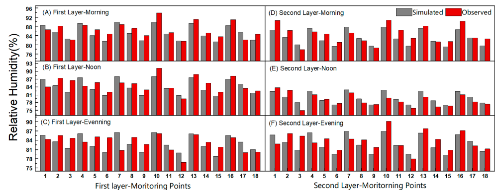
Figure 9. Comparison of simulated and measured relative humidity at the monitoring locations.
