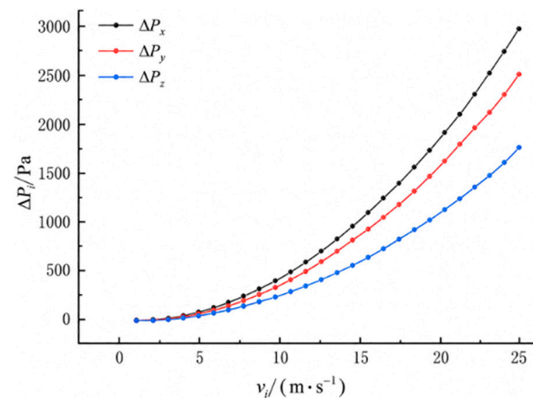
Figure 7. Velocity–pressure-drop fitting plots in different directions.
