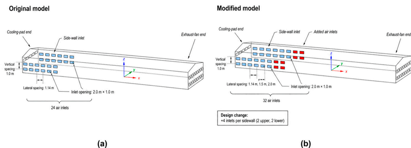
Figure 18. Schematic diagram of air inlet configuration optimization schemes: (a) original model; (b) optimized model with additional air inlets.
