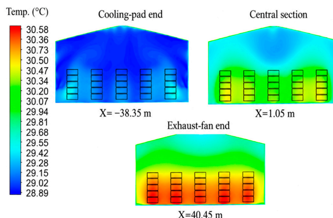
Figure 12. X-direction temperature field comparison.
