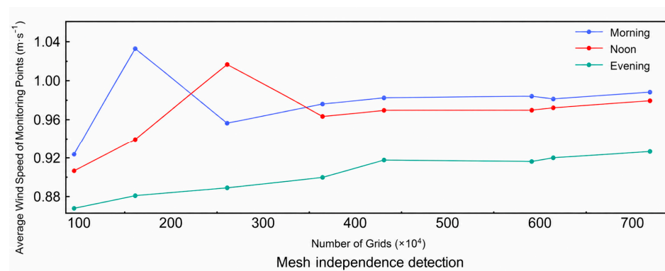
Figure 5. Results of mesh independence test.
