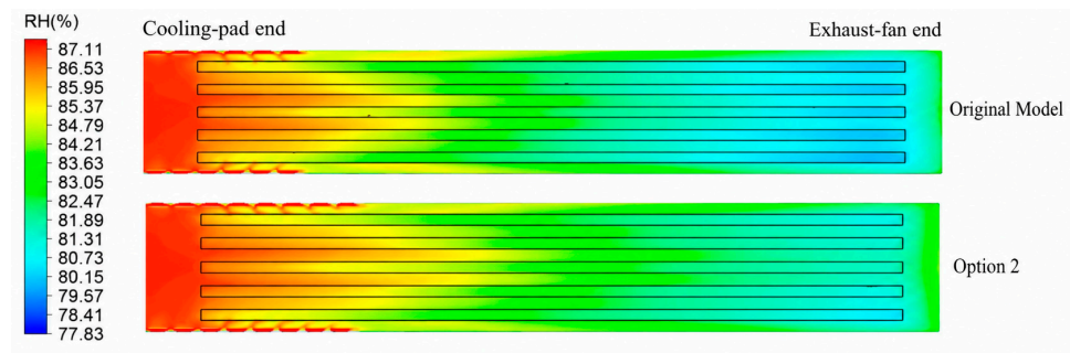
Figure 21. Comparison diagram of relative humidity field.
