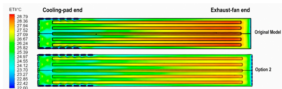
Figure 23. Comparison diagram of perceived temperature fields.
