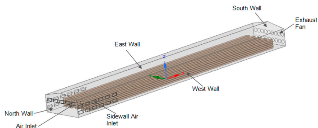
Figure 3. Laying hen house model diagram.
