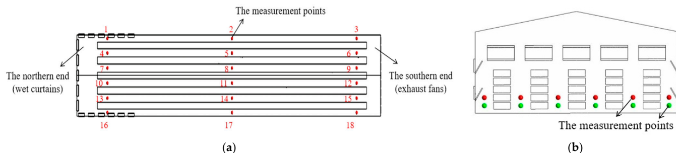
Figure 2. Schematic diagram of the measurement locations: (a) measurement locations along the laying hen house; (b) front view of the chicken coop.
