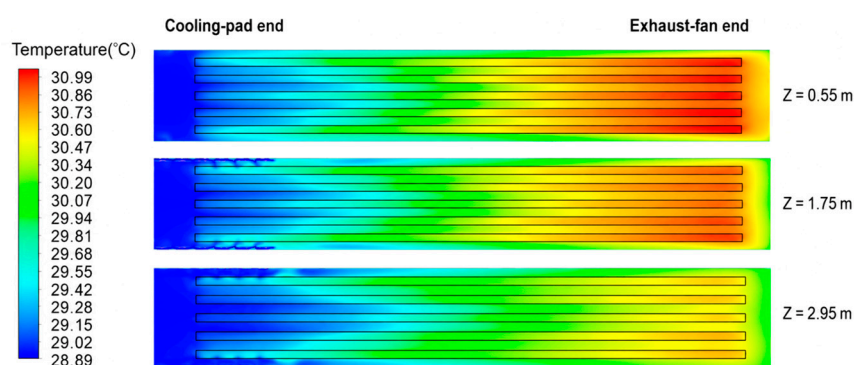
Figure 13. Temperature distributions on three horizontal plans at heights of 0.5, 1.75, and 2.95 m from the floor.
