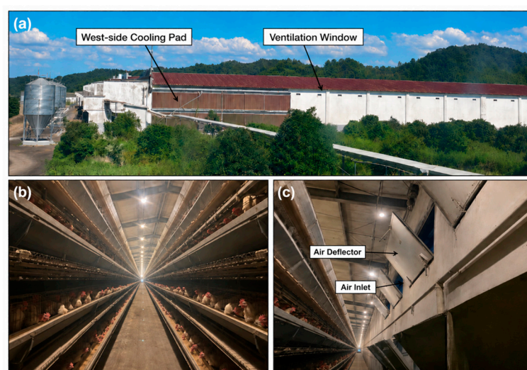
Figure 1. Experimental laying hen house and ventilation system configuration: (a) exterior view of the laying hen house; (b) interior view of the laying hen house; (c) sidewall ventilation structure with air inlet and air deflector.
