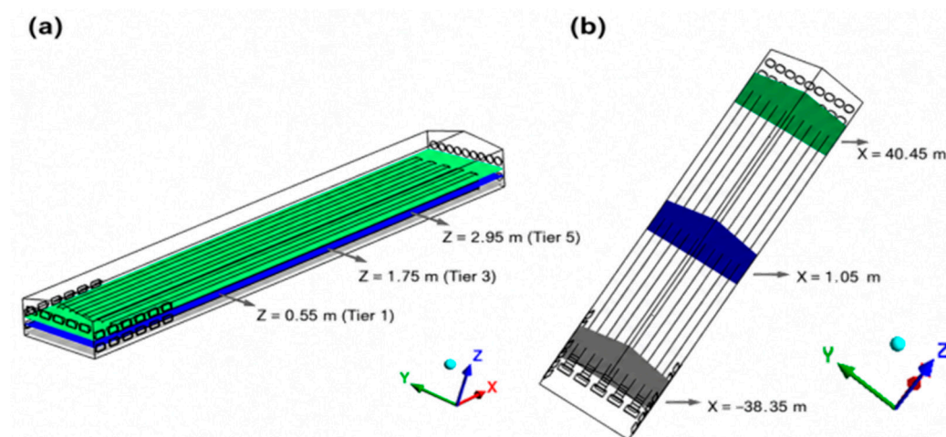
Figure 11. Locations of the environmental analysis planes: (a) horizontal planes at Z = 0.55 , 1.75 , and 2.95 m; (b) transverse vertical planes at X = -38.35 , 1.05 , and 40.45 m.
