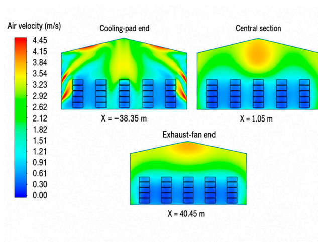
Figure 16. Wind speed fields at different distances.
