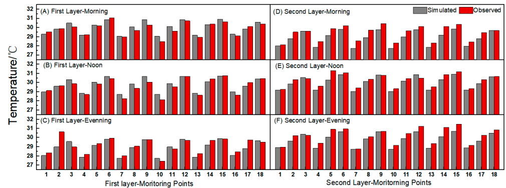
Figure 8. Comparison of simulated and measured air temperatures at the monitoring locations.
