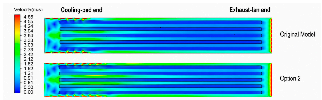
Figure 22. Comparison diagram of air velocity fields.
