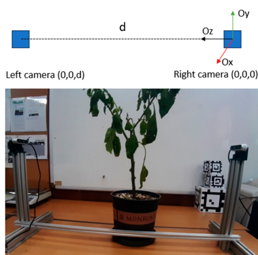
Figure 5. Experimental setup of leaf area estimation using two RGB-D cameras.
