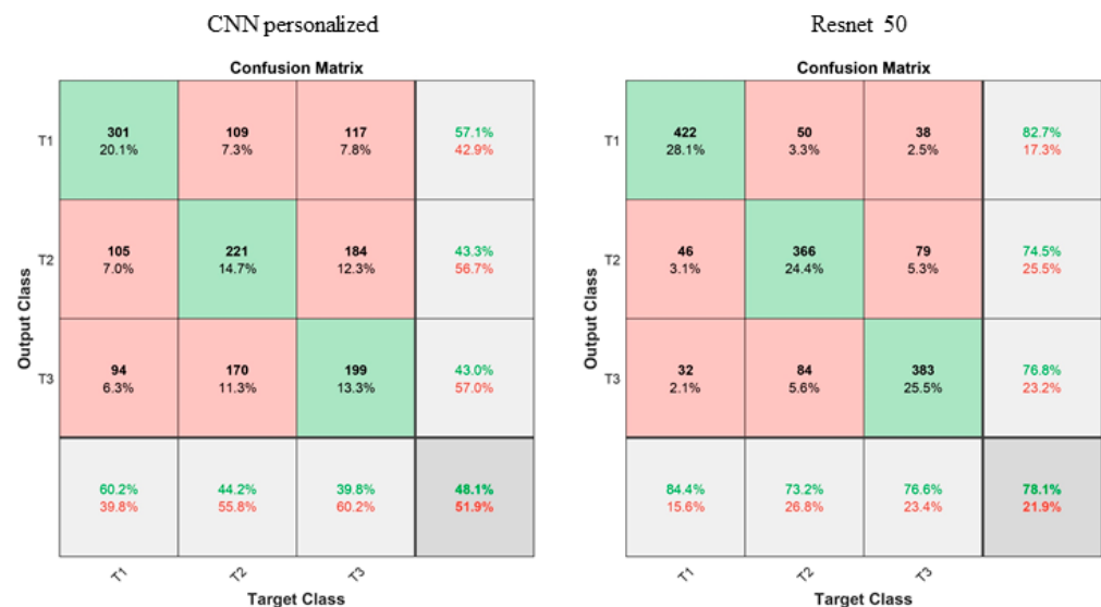
Figure 3. Confusion matrix between neural network-based models for classification of nitrogen doses in strawberry floral induction. In green (main diagonal) are the true positives of each class. In salmon, horizontally there are false negatives, and vertically the false positives. In light and dark gray are accuracies and errors by classes and total respectively.
