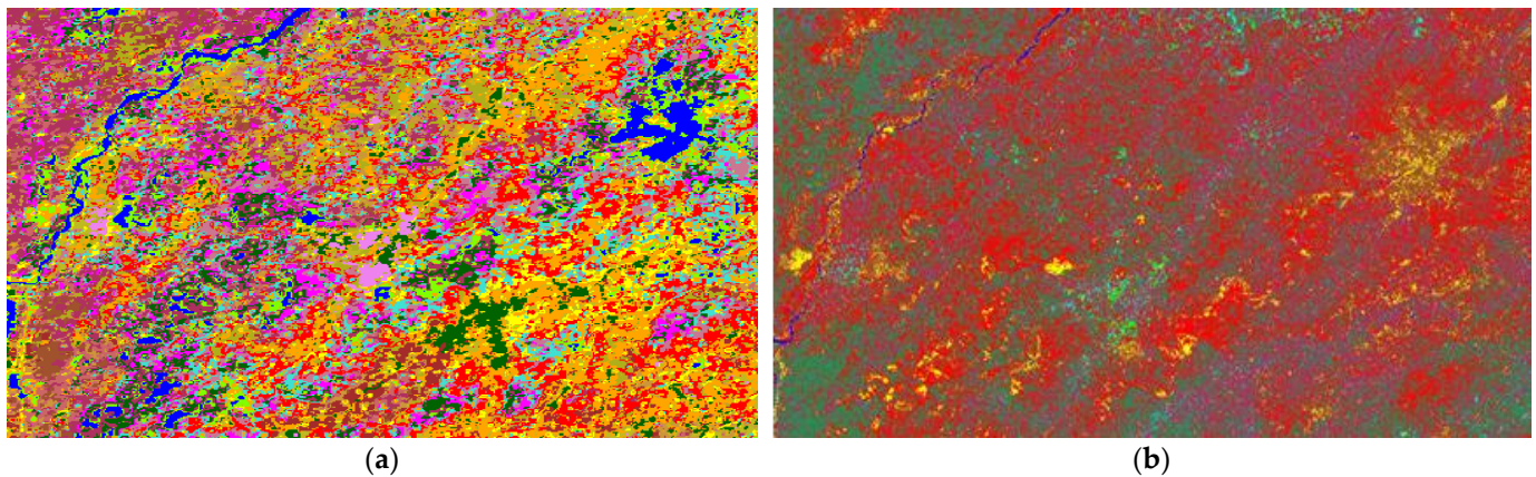
Figure 4. Comparison of the currently developed LULC map (a) from MODIS with the (b) fine resolution Landsat5 TM map.
