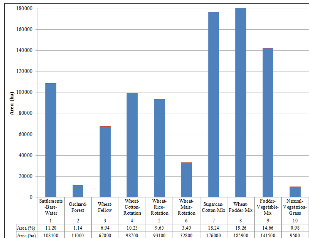
Figure 7. LULC classes and their areal extent in Faisalabad and Toba Tek Singh Districts.
