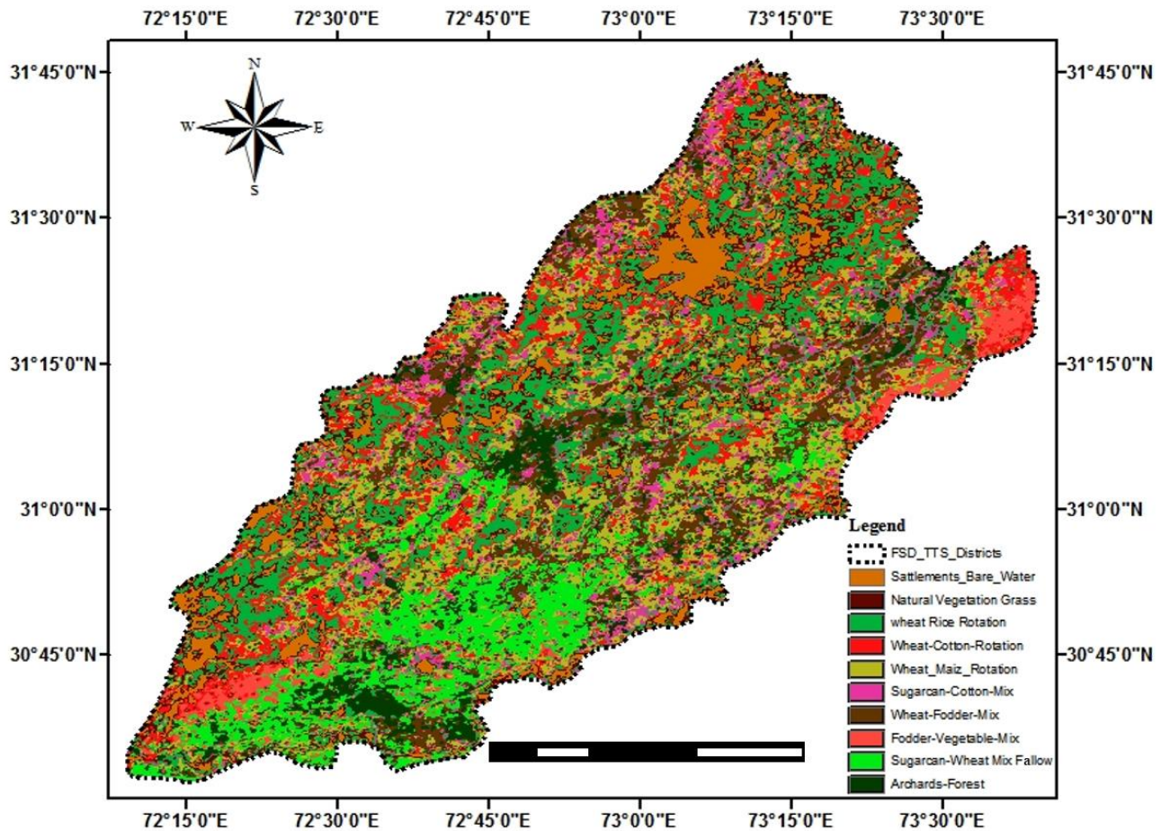
Figure 6. Land cover and land use map developed from 46 MODIS NDVI layers for 2008–2009.
