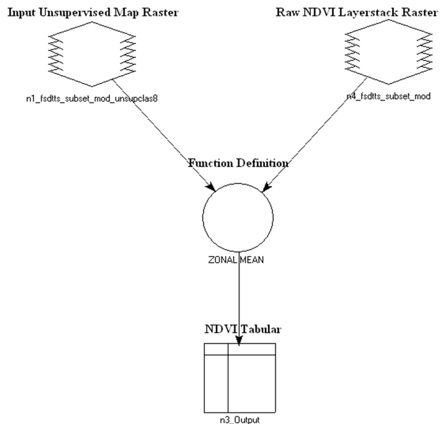
Figure 3. Model for digital values of the NDVI derivation.
