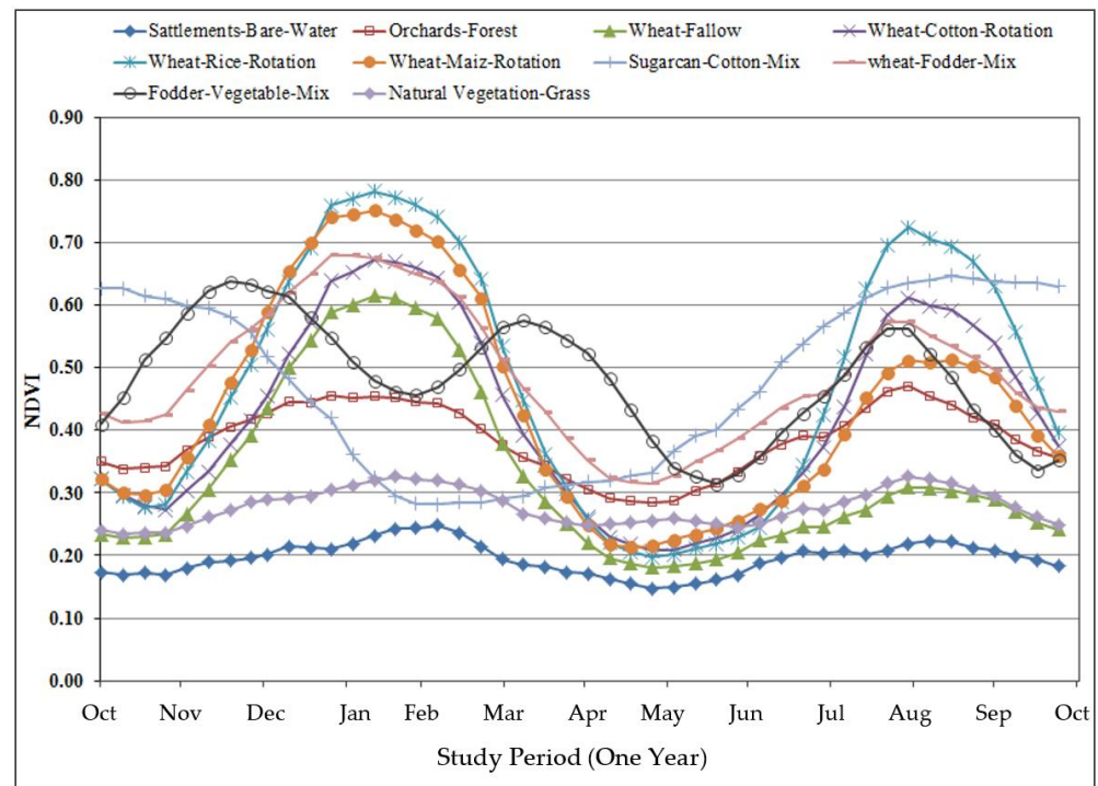
Figure 5. Crop phenology and NDVI profiles of final agriculture/crop classes.
