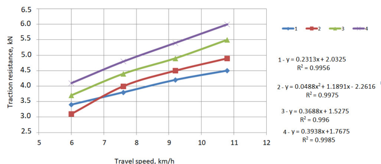
Figure 16. Influence of travel speed on the traction resistance of design–technological schemes; 1—scheme №1; 2—scheme №2; 3—scheme №4; 4—scheme №3.
