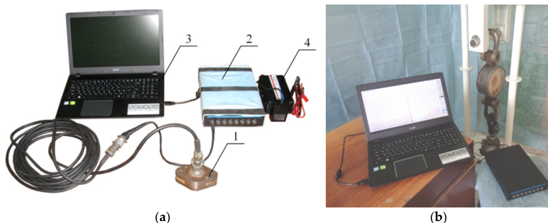
Figure 5. General view of strain-gauge equipment: (a)—strain-gauge equipment; (b)—calibration stand for strain-gauge links; 1—strain-gauge link; 2—strain-gauge station; 3—portable PC; 4—12–220 V voltage converter.
