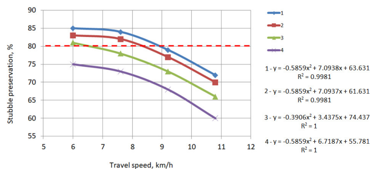
Figure 14. Influence of travel speed on stubble preservation; 1 is scheme №1; 2 is scheme №2; 3 is scheme №4; 4 is scheme №3.
