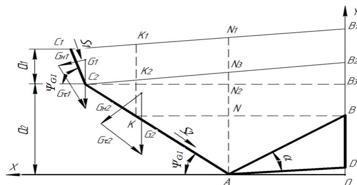
Figure 6. The scheme of the decomposition of forces acting on the wedge due to the weight of the soil layer.
