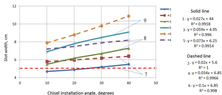
Figure 11. Effect of shank thickness, chisel angle, and chisel width on slit width; shank thickness (solid line)—20 mm; shank thickness (dashed line)—30 mm; chisel width: 7—40 mm; 8—50 mm; 9—60 mm.
