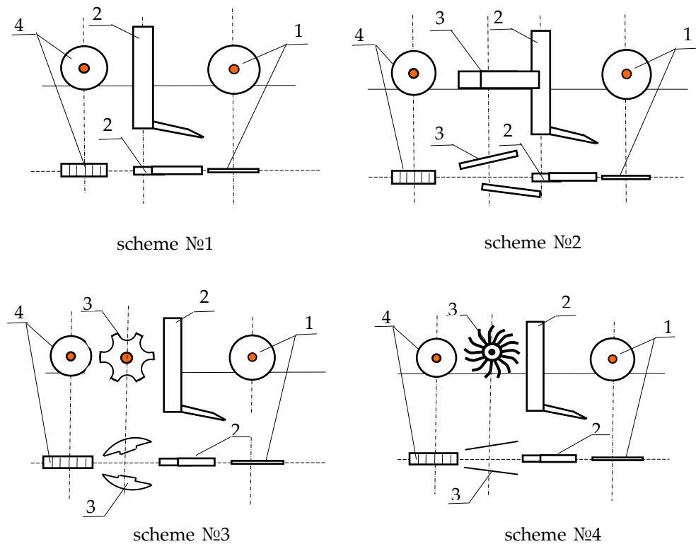
Figure 1. Structural-technological schemes: 1—cutting disk; 2—chisel; 3—soil turners; 4—packing roller.
