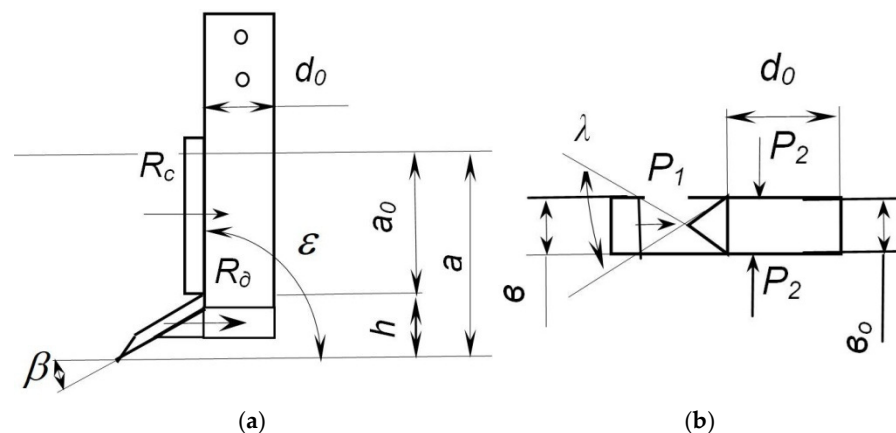
Figure 8. Chisel calculation scheme; (a) side view; (b) top view.
