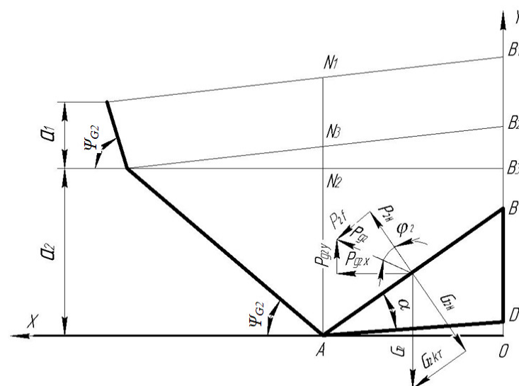
Figure 7. Force diagram acting on a two-edged wedge due to the weight of the soil layer.
