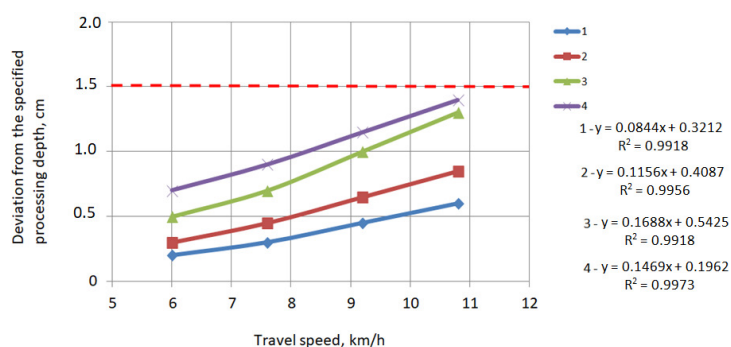
Figure 13. Influence of travel speed on working-depth deviation; 1 is scheme №1; 2 is scheme №2; 3 is scheme №3; 4 is scheme №4.
