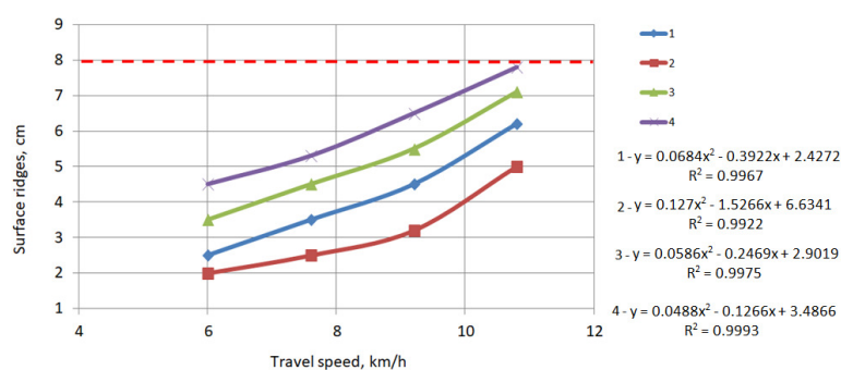
Figure 15. Influence of travel speed on ridge height; 1 is scheme №1; 2 is scheme №2; 3 is scheme №3; 4 is scheme №4.
