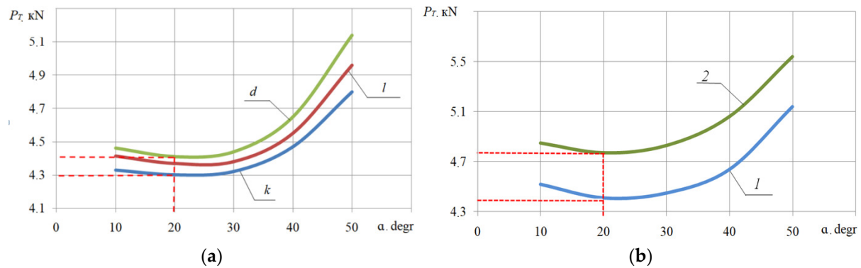
Figure 9. The influence of shank thickness, chisel width and chisel angle relative to the furrow bottom on the traction resistance of the chisel: (a) the influence of chisel angle on traction resistance at 20 mm shank thickness; (b) the influence of shank thickness with a chisel width of 50 mm. 1—a shank thickness of 20 mm; 2—a shank thickness of 30 mm; chisel width: k —40 mm; l —50 mm; d —60 mm.
