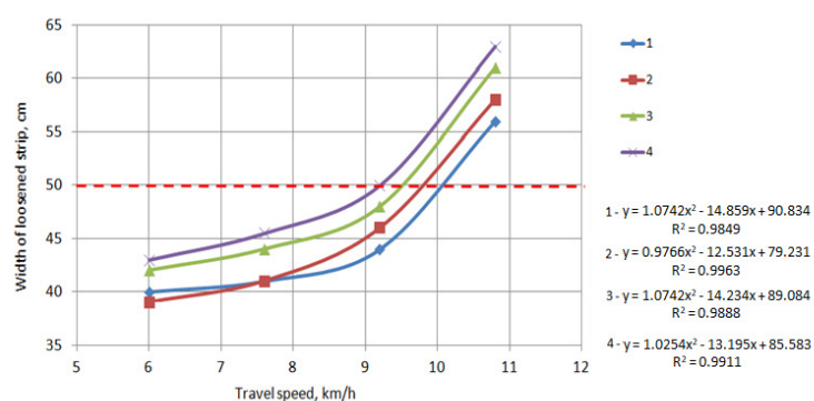
Figure 12. Effect of travel speed and design–technological schemes on the width of the loosened strip; 1 is scheme №1; 2 is scheme №2; 3 is scheme №3; 4 is scheme №4.
