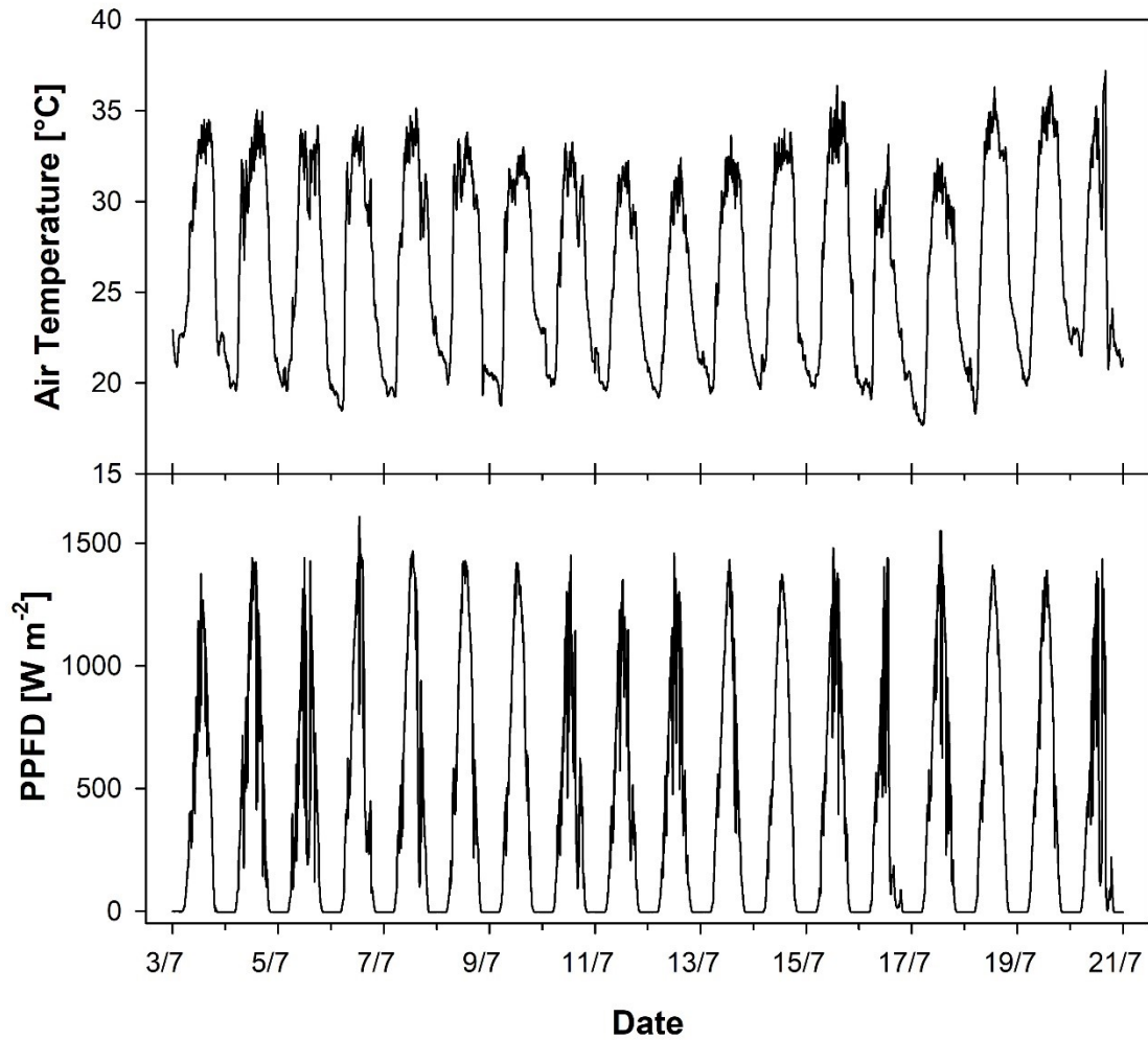
Figure S1. Air temperature (A) and Photosynthetic Photon Flux Density (PPFD) (B) measured at the weather station within the experimental tunnel at the University of Padova, Legnaro, Italy, during the water stress trial period.
