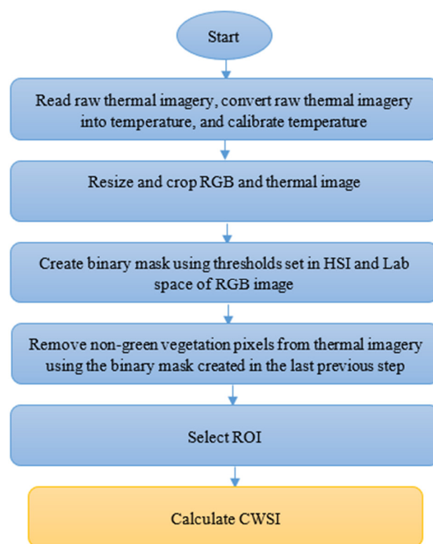
Figure 2. Steps used in analyzing color and thermal imagery for CWSI calculation.
