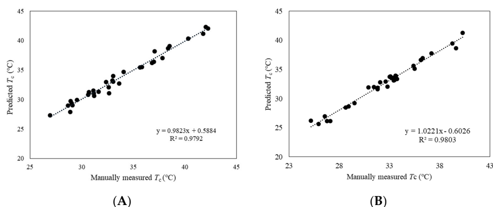
Figure 4. Performance of the proposed imaging processing algorithm for average T_c calculation relative to the manually measured T_c in the (A) shaded side and (B) sunlit side of vine canopies.
