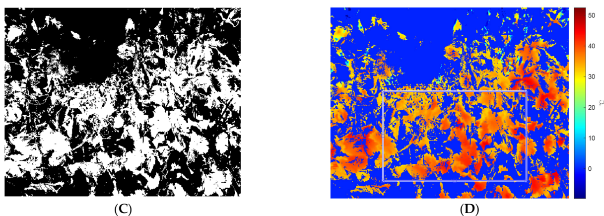
Figure 3. Thermal imagery and processed image of a sample grapevine canopy: (A) false color thermal image, (B) original RGB image, (C) canopy binary mask, (D) overlapped thermal image with selected rectangle ROI.
