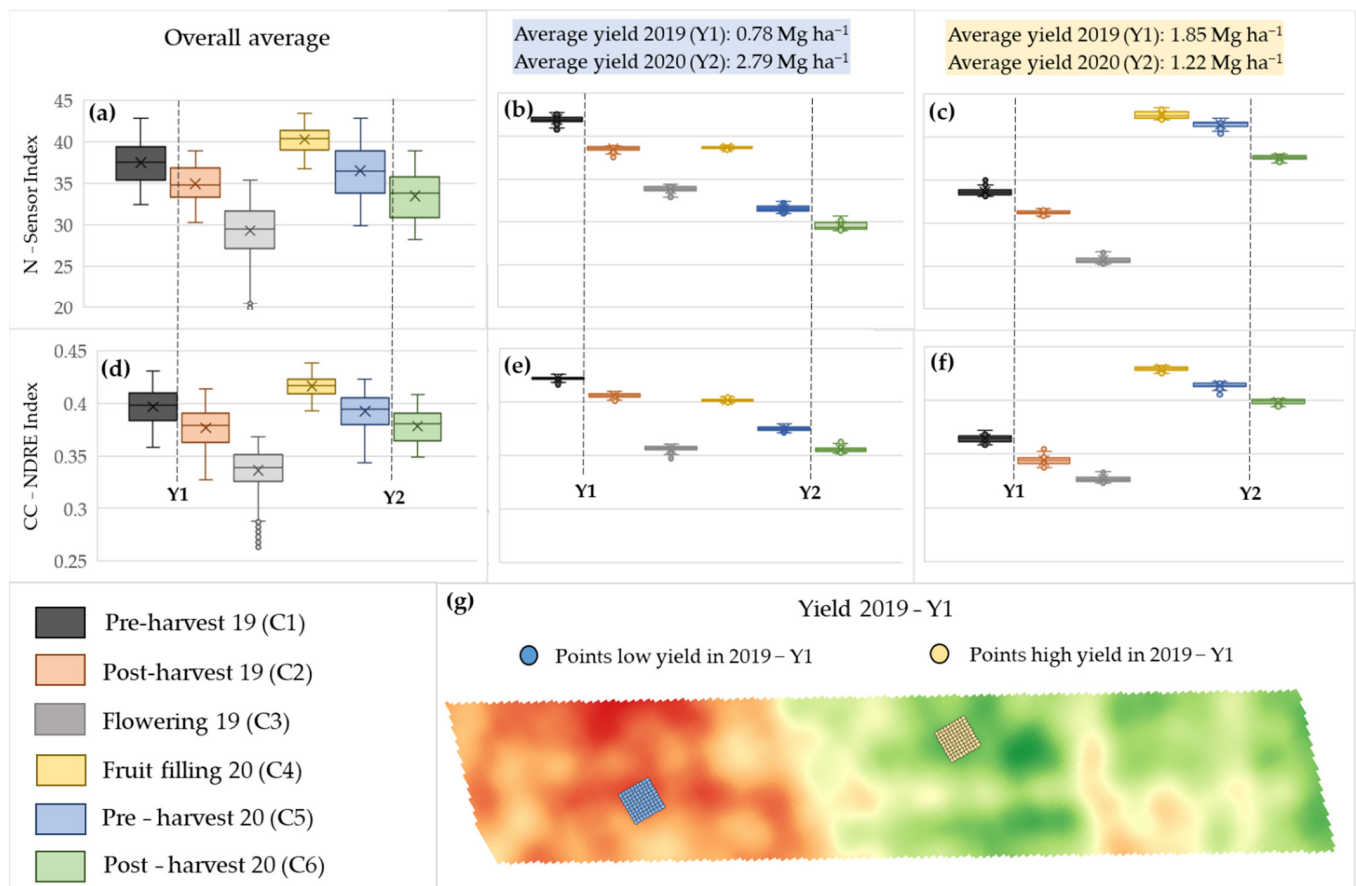
Figure 5. Temporal behavior of the N-Sensor vegetation index (from C1 to C6) showing the boxplots of all field data (a), the boxplots of an area with low yield in 2019 and high yield in 2020 (b), and the boxplots of an area with high yield in 2019 and low yield in 2020 (c). Temporal behavior of the CC-NDRE vegetation index (from C1 to C6) showing the boxplots of all field data (d), the boxplots of an area with low yield in 2019 and high yield in 2020 (e), and the boxplots of an area with high yield in 2019 and low yield in 2020 (f). For the graphs generated in (b,c,e,f), 100 sampling points were used for the regions of low and high yield (g).
