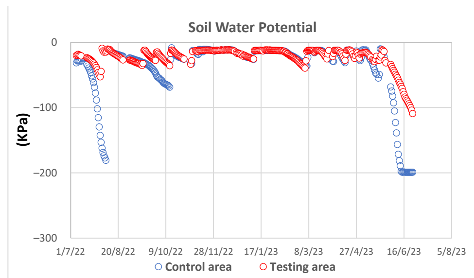
Figure 7. Soil water potential during the monitoring period (7 July 2022–6 July 2023).
