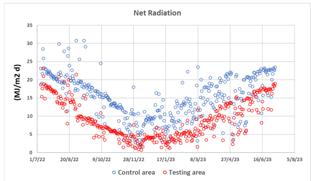
Figure 4. Net radiation in control and testing area (7 July 2022–6 July 2023).
