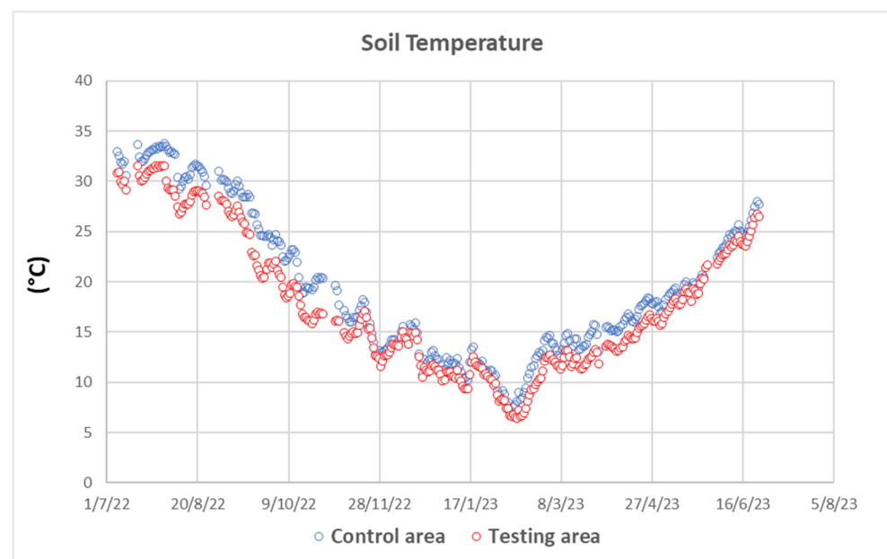
Figure 6. Soil temperature during the monitoring period (7 July 2022–6 July 2023).
