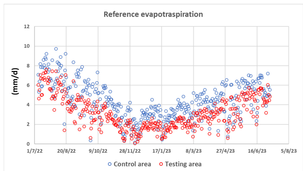
Figure 5. Reference evapotranspiration in control and testing area (7 July 2022–6 July 2023).
