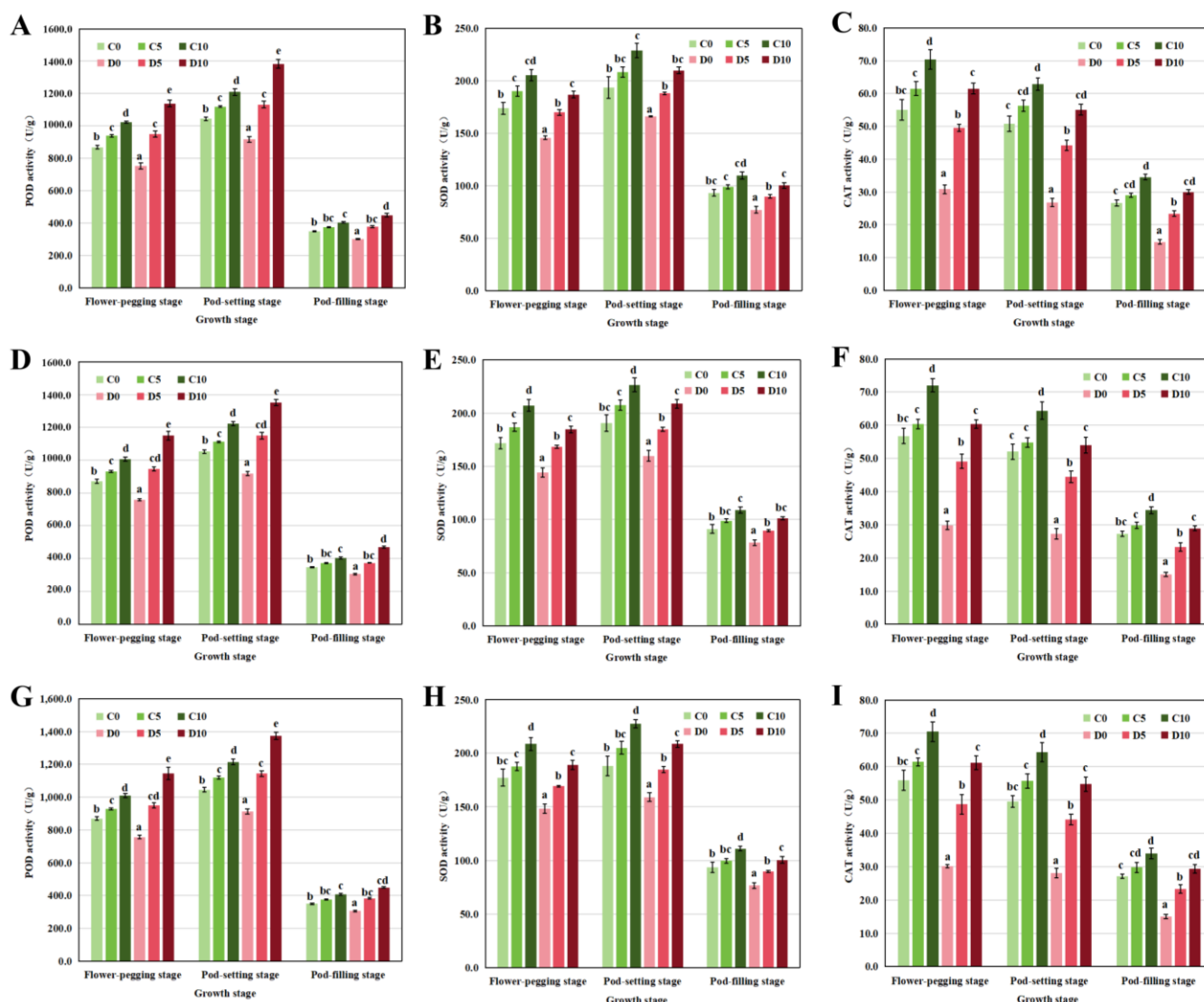
Figure 2. Defense-related enzymes induced by T6P in adzuki bean during post-drought recovery during growing seasons. POD: 2023 (A), 2022 (D), 2021 (G); SOD: 2023 (B), 2022 (E), 2021 (H); CAT: 2023 (C), 2022 (F), 2021 (I). Vertical bars represent the standard error of the mean of three replicates ( n = 30 ). Different letters on bars at the same growth stage indicate significant differences among treatments by Duncan's multiple range test ( p < 0.05 ). C0, C5 and C10 represent the combinations of control with the application of 0, 5 and 10 \mu\text{M} T6P, respectively; D0, D5 and D10 represent the combinations of drought stress with the application of 0, 5 and 10 \mu\text{M} T6P, respectively. C: control; D: drought. POD: peroxidase; SOD: superoxide dismutase; CAT: catalase.
