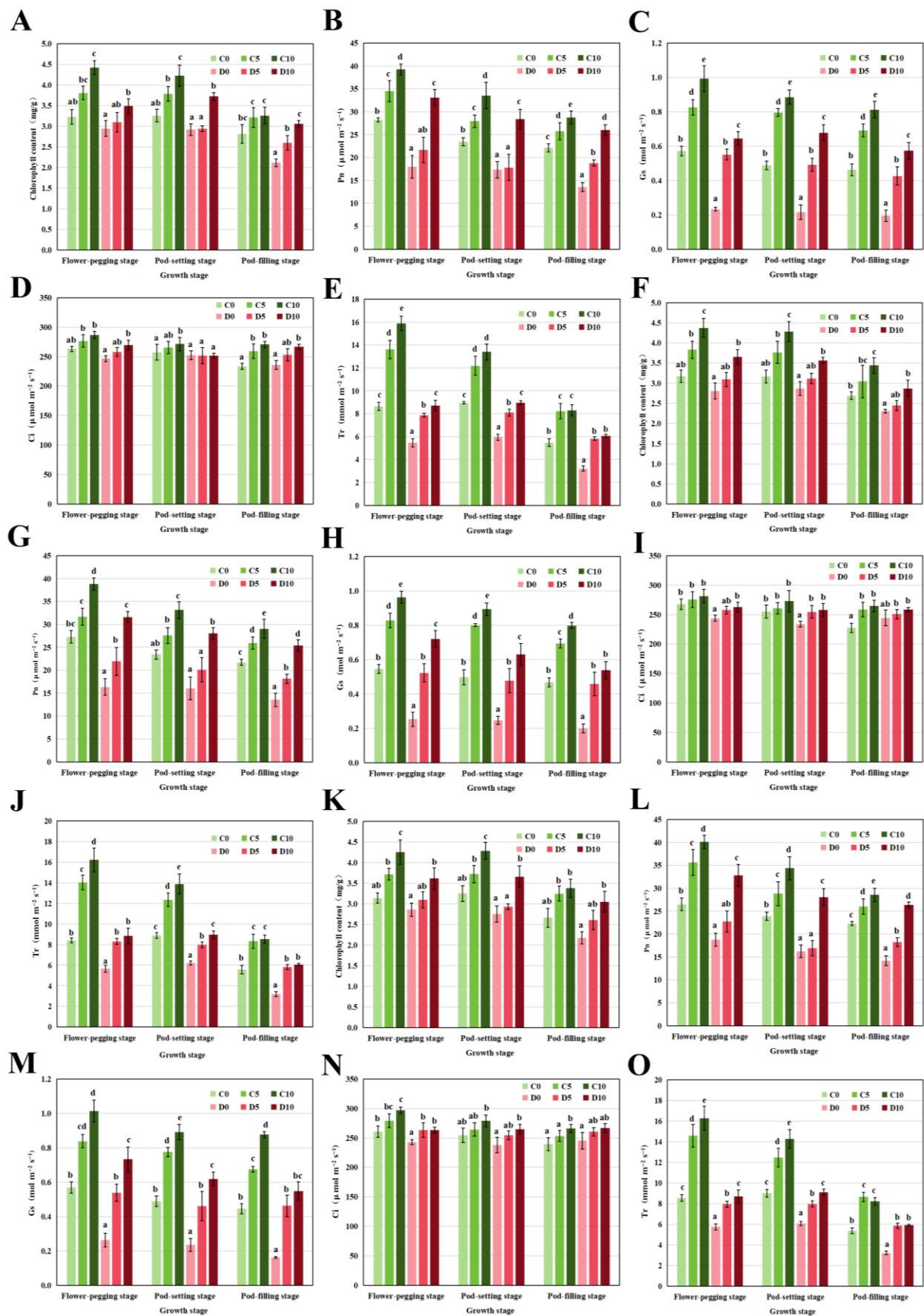
Figure 1. Photosynthetic characteristics in adzuki bean during post-drought recovery caused by T6P during growing seasons. Chlorophyll measurement: 2023 (A), 2022 (F), 2021 (K); net photosynthetic rate: 2023 (B), 2022 (G), 2021 (L); stomatal conductance: 2023 (C), 2022 (H), 2021 (M); intercellular
