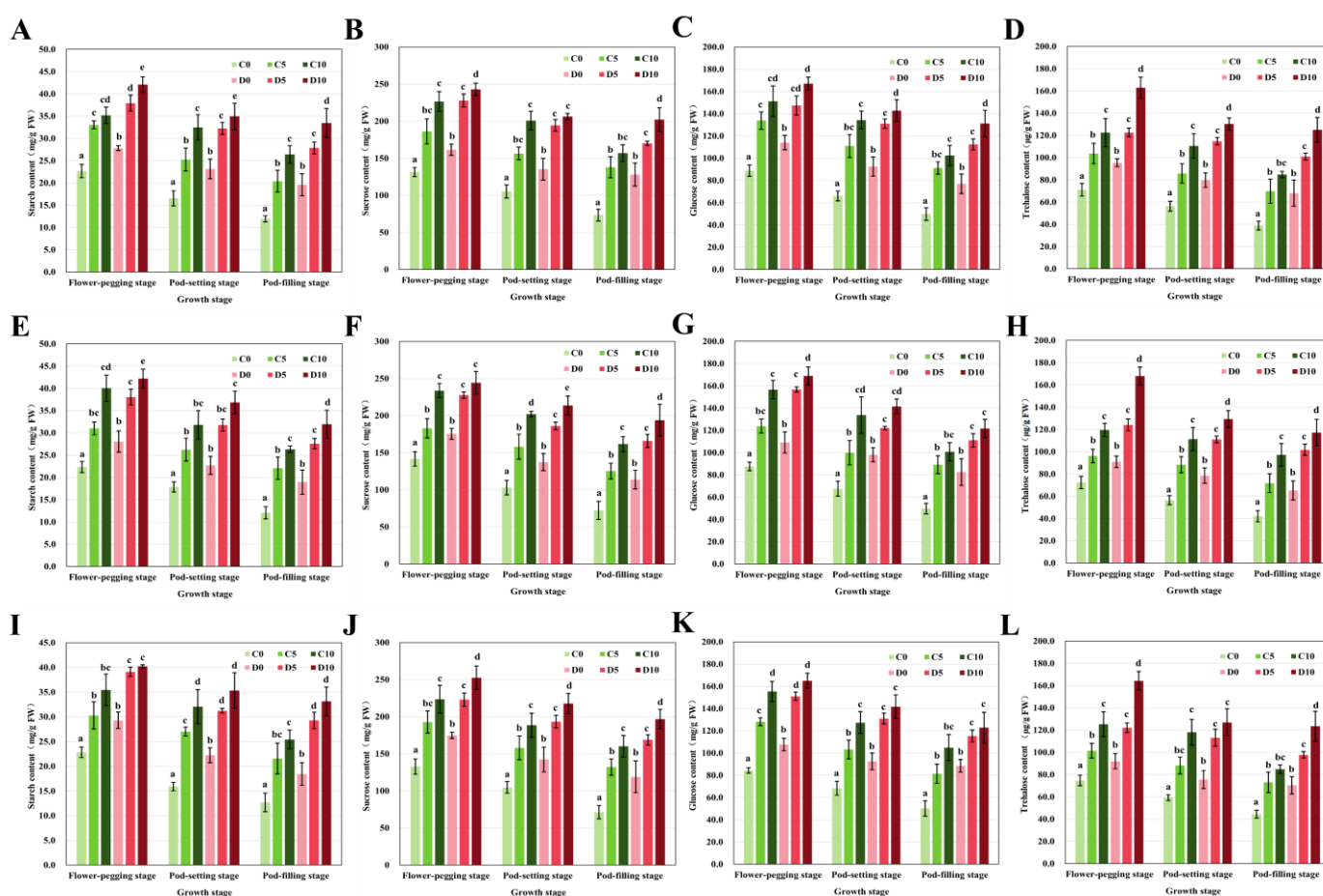
Figure 4. T6P-mediated sugar molecules in adzuki bean during post-drought recovery during growing seasons. Starch: 2023 (A), 2022 (E), 2021 (I); sucrose: 2023 (B), 2022 (F), 2021 (J); glucose: 2023 (C), 2022 (G), 2021 (K); trehalose: 2023 (D), 2022 (H), 2021 (L). Vertical bars represent the standard error of the mean of three replicates ( n = 30 ). Different letters on bars at the same growth stage indicate significant differences among treatments by Duncan's multiple range test ( p < 0.05 ). C0, C5 and C10 represent the combinations of control with the application of 0, 5 and 10 \mu\text{M} T6P, respectively; D0, D5 and D10 represent the combinations of drought stress with the application of 0, 5 and 10 \mu\text{M} T6P, respectively. C: control; D: drought.
