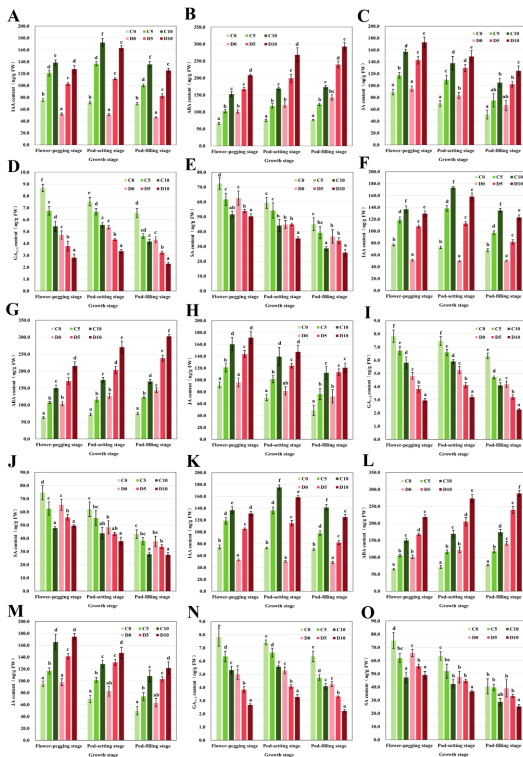
Figure 5. Effects of foliar T6P application on endogenous hormone accumulation profiles in adzuki bean leaves during post-drought recovery across the growing seasons. IAA: 2023 (A), 2022 (F), 2021 (K); ABA: 2023 (B), 2022 (G), 2021 (L); JA: 2023 (C), 2022 (H), 2021 (M); GA: 2023 (D), 2022 (I), 2021 (N); SA: 2023 (E), 2022 (J), 2021 (O). Vertical bars represent the standard error of the mean of three replicates ( n = 30 ). Different letters on bars at the same growth stage indicate significant differences among treatments by Duncan's multiple range test ( p < 0.05 ). C0, C5 and C10 represent the combinations of controls with the application of 0, 5 and 10 \mu\text{M} T6P, respectively; D0, D5 and D10 represent the combinations of drought stress with the application of 0, 5 and 10 \mu\text{M} T6P, respectively. C: control; D: drought. IAA: indoleacetic acid; ABA: abscisic acid; JA: jasmonic acid; GA: gibberellin; SA: salicylic acid.
