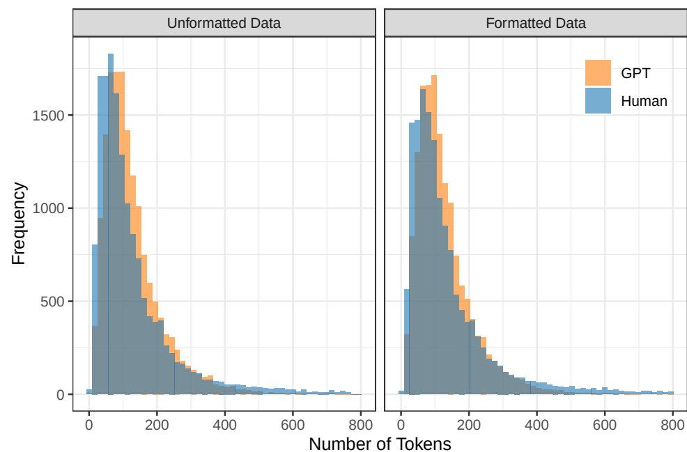
Figure 4. Distribution of the code length (number of tokens according to cl100k_base encoding) across the unformatted and formatted dataset. Values larger than the 99% quantile were removed to avoid a distorted picture.
