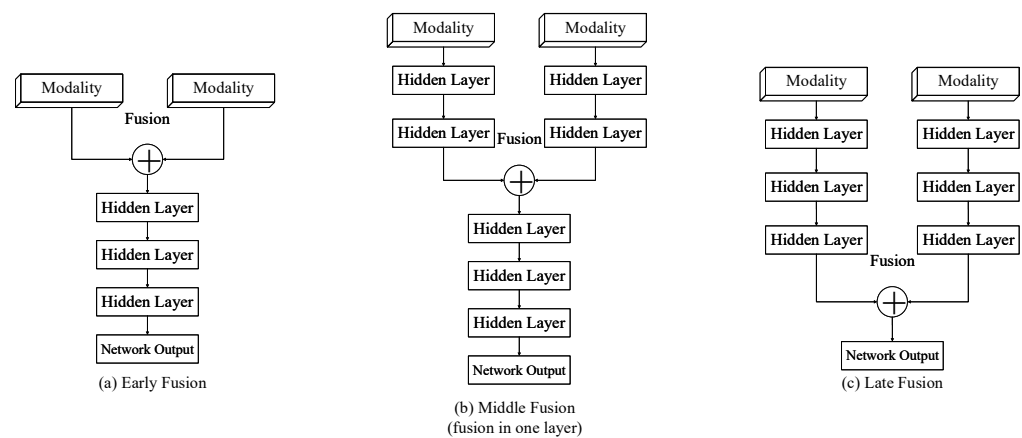
Figure 5. Comparison of representative multimodal fusion strategies for emotional stress recognition, including early (feature-level), mid-level (hidden-layer), and late (decision-level) fusion.
