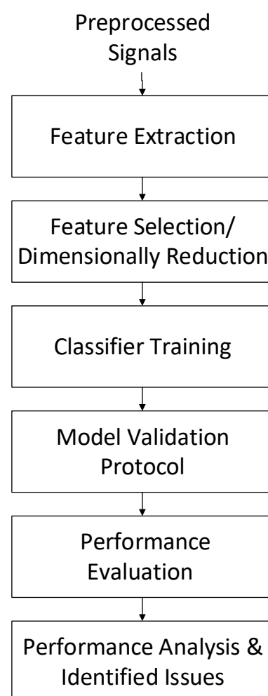
Figure 6. Traditional machine learning-based multimodal stress recognition framework.
