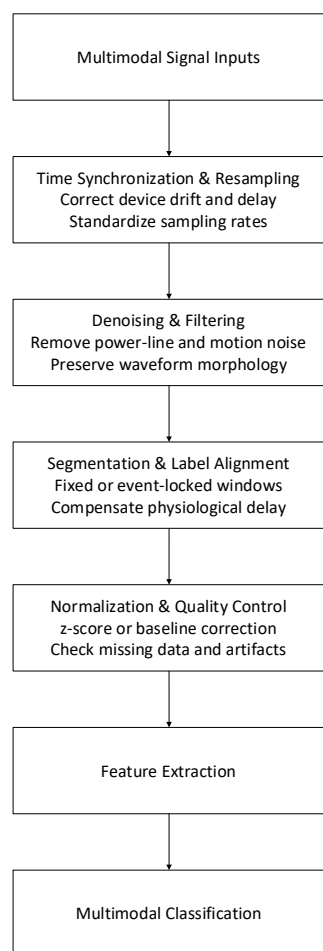
Figure 4. Overview of preprocessing and feature extraction workflow for multimodal emotional stress analysis.
