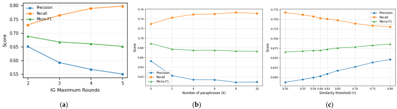
Figure 4. Sensitivity analysis of the proposed model on Arabic datasets. (a) Effect of iterative generation rounds. (b) Effect of number of paraphrases. (c) Effect of semantic similarity threshold.
