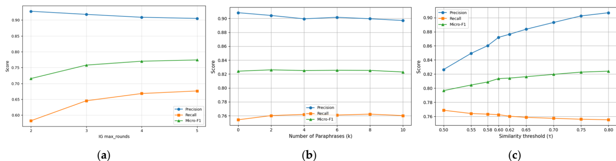
Figure 3. Sensitivity analysis: (a) iterative generation rounds; (b) number of paraphrases; (c) semantic similarity threshold \tau .
