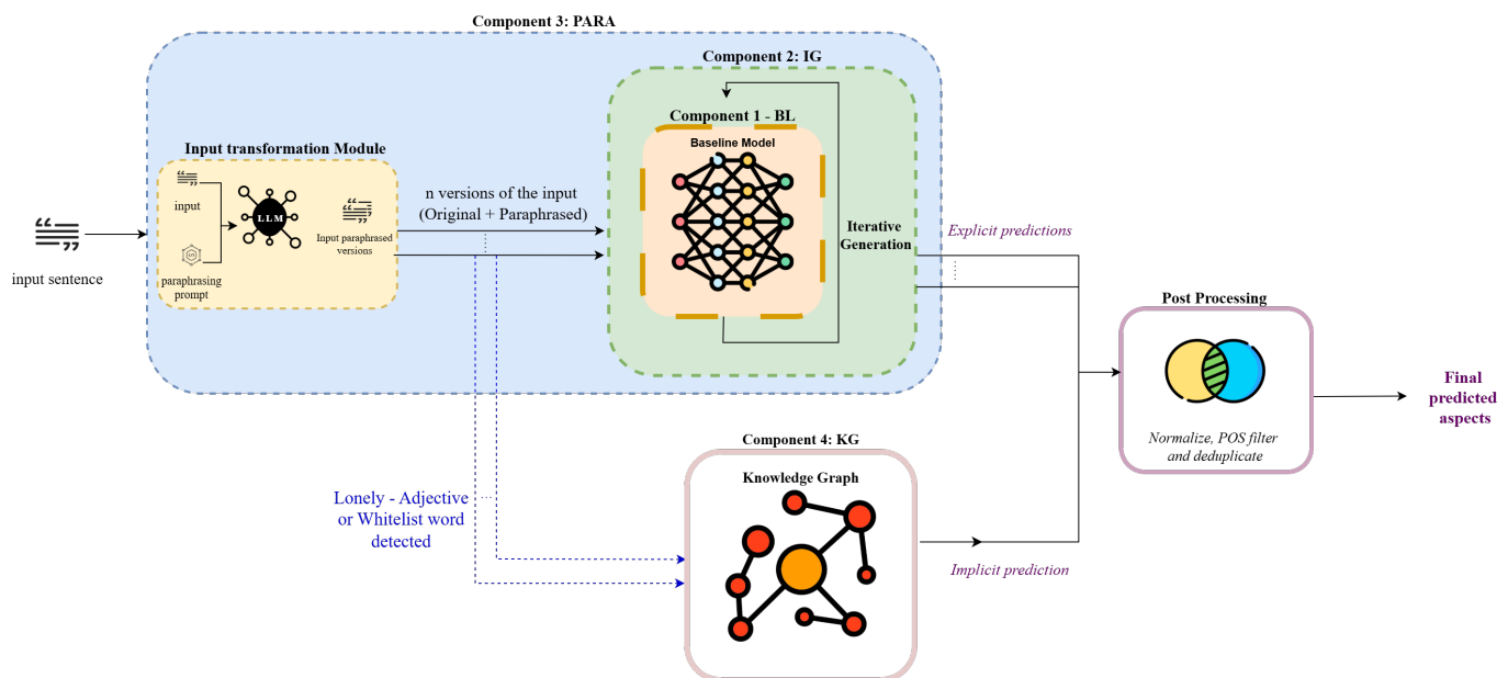
Figure 1. Overview of the proposed four-component pipeline for explicit and implicit aspect extraction. Arrows indicate the flow of sentence representations. Parallel double lines indicate multiple original and paraphrased inputs passed in parallel to the baseline model.
