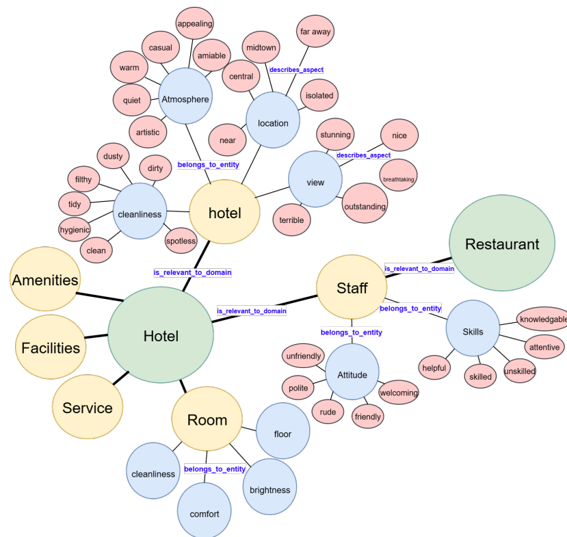
Figure 2. An illustrative subgraph of the English knowledge graph, showing the four vertex types and their relationships. Domain vertices: green; entity vertices: yellow; aspect vertices: blue; clue vertices: pink. Edges represent the relations is_relevant_to , belongs_to , and describes_aspect , enabling multi-hop inference from surface clues to domain-specific aspects.
