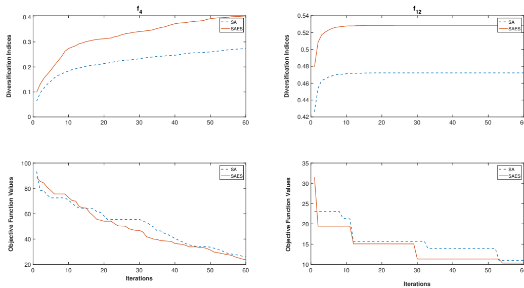
Figure 7. Examples of the SA and SAES diversification performance using classical test functions.
