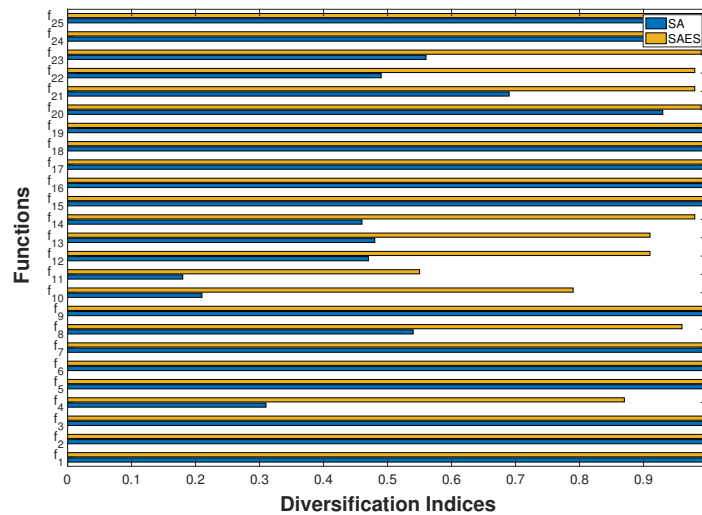
Figure 5. Diversification indices of classical test functions.
