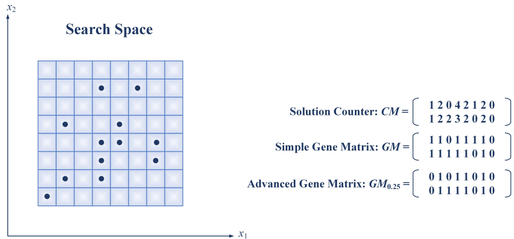
Figure 1. An example of the Gene Matrix in R^2 .
