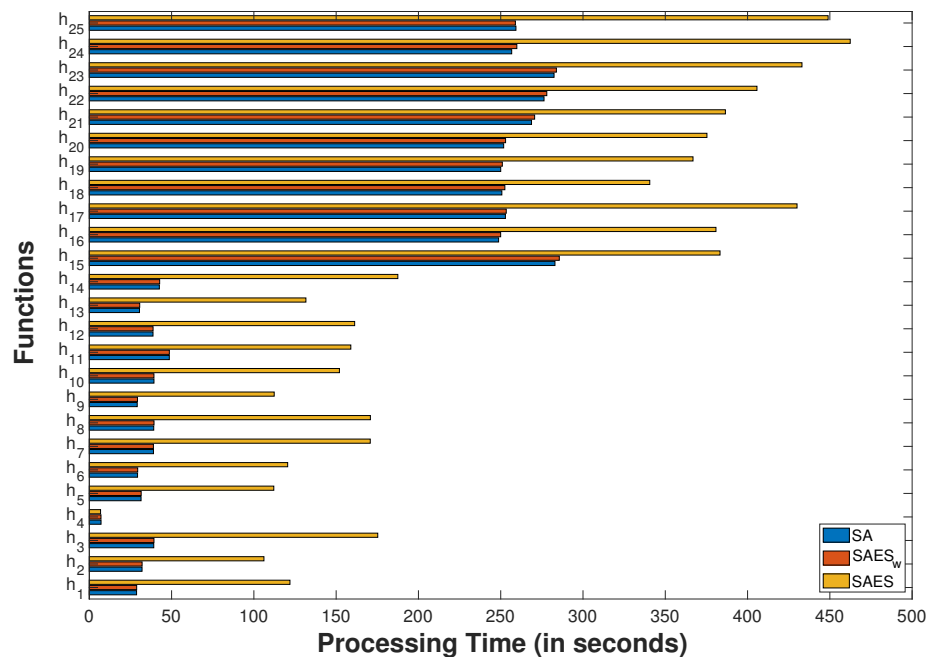
Figure 4. Averages of processing time in seconds using the hard test functions.
