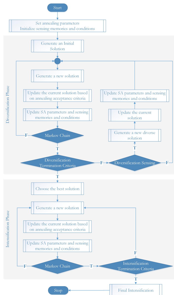
Figure 2. Flowchart of the proposed methodology.
