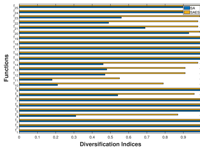
Figure 6. Diversification indices of classical hard functions.
