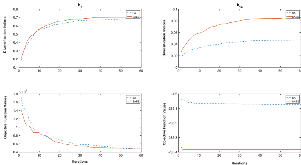
Figure 8. Examples of the SA and SAES diversification performance using hard test functions.
