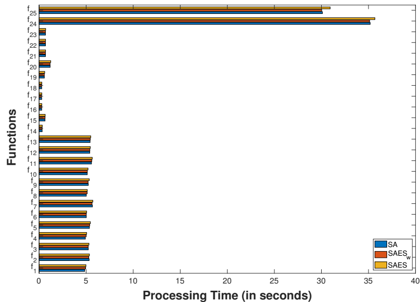
Figure 3. Averages of processing time in seconds using the classical test functions.
