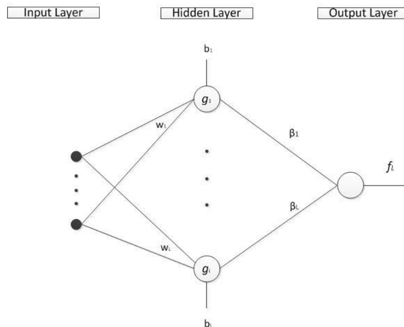
Figure 1. SLFN with additive nodes.
