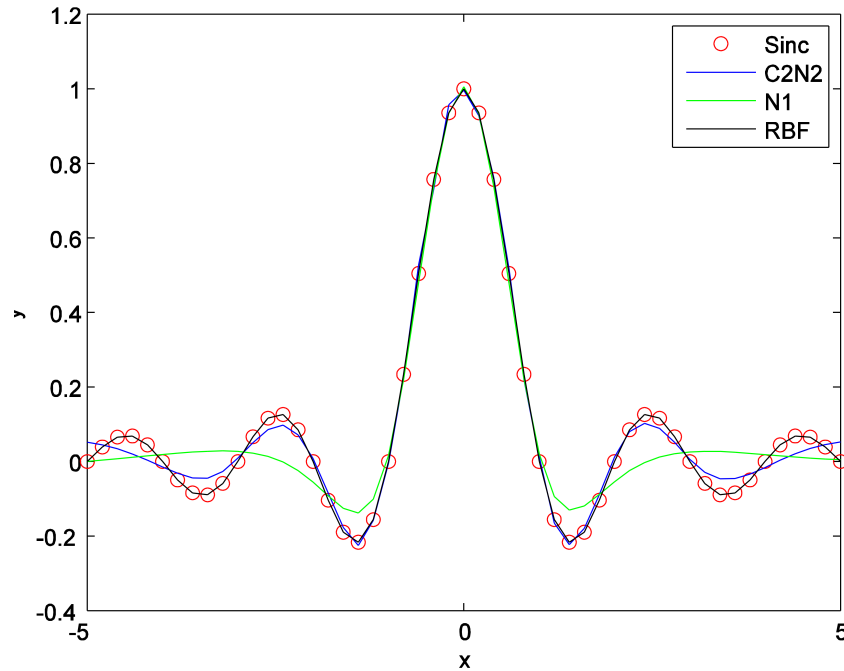
Figure 8. Comparison of C2N2 with RBF and the network N_1 . The experiment is performed on the approximation of the Sinc function.
