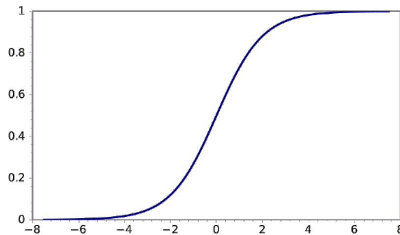
Figure 4. Sigmoid function.
