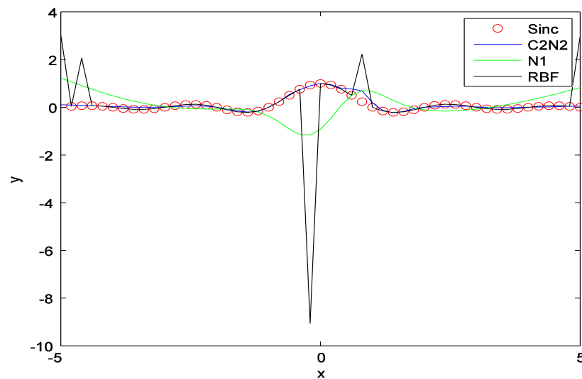
Figure 9. Comparison of C2N2 with RBF and the network N_1 . The experiment is performed on the approximation of the Sinc function and in the presence of impulsive noise.
