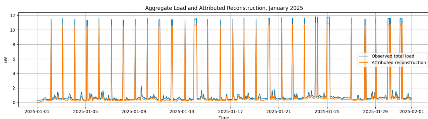
Figure 5. Aggregate load and attributed reconstruction for January 2025.
