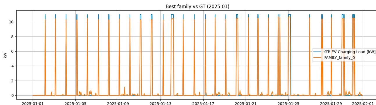
Figure 7. Hourly comparison between the EV-aligned family contribution and the reference EV charging load for January 2025.
