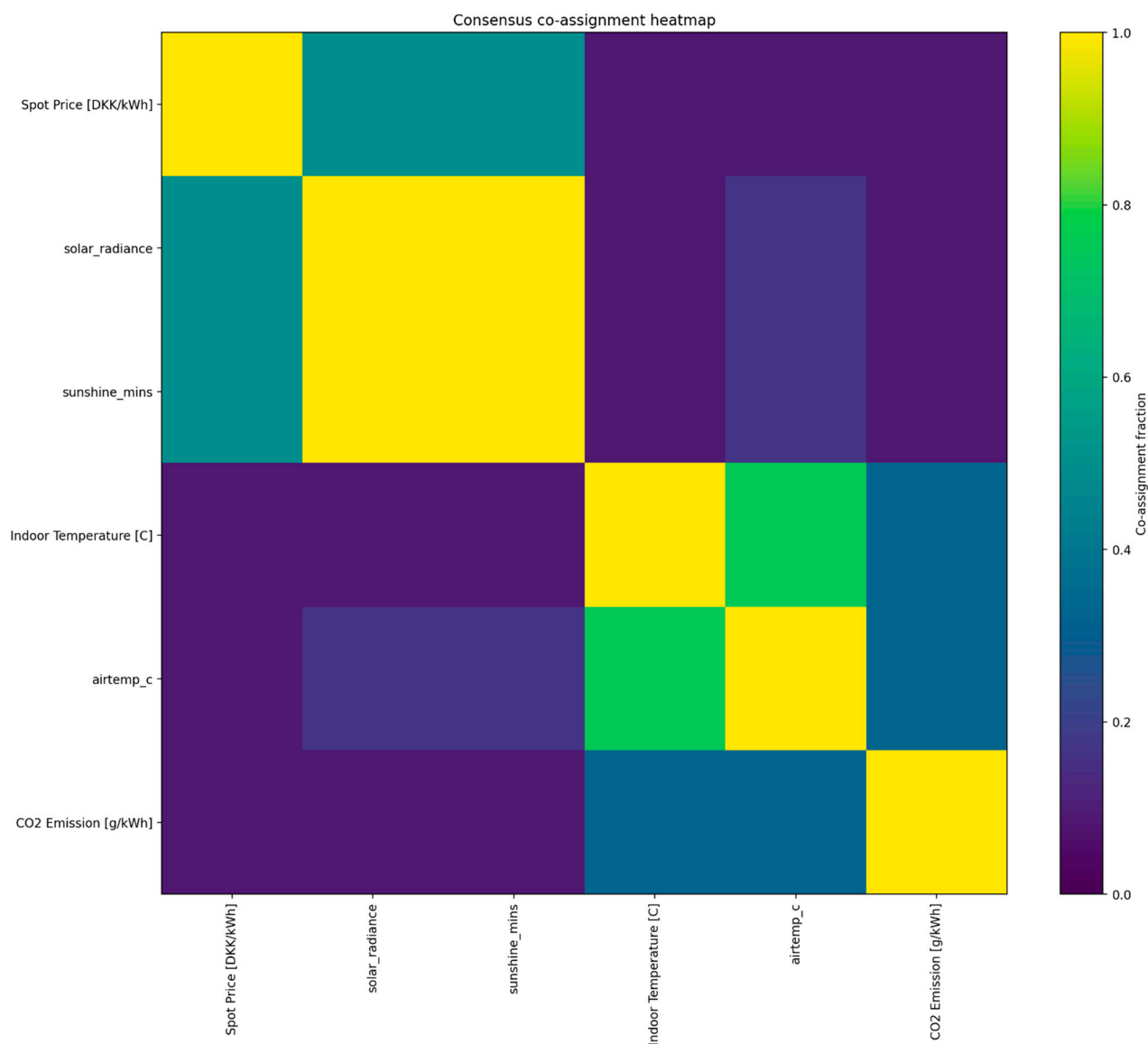
Figure 3. Consensus co-assignment matrix showing the fraction of relation layers in which each pair of features is assigned to the same family.
