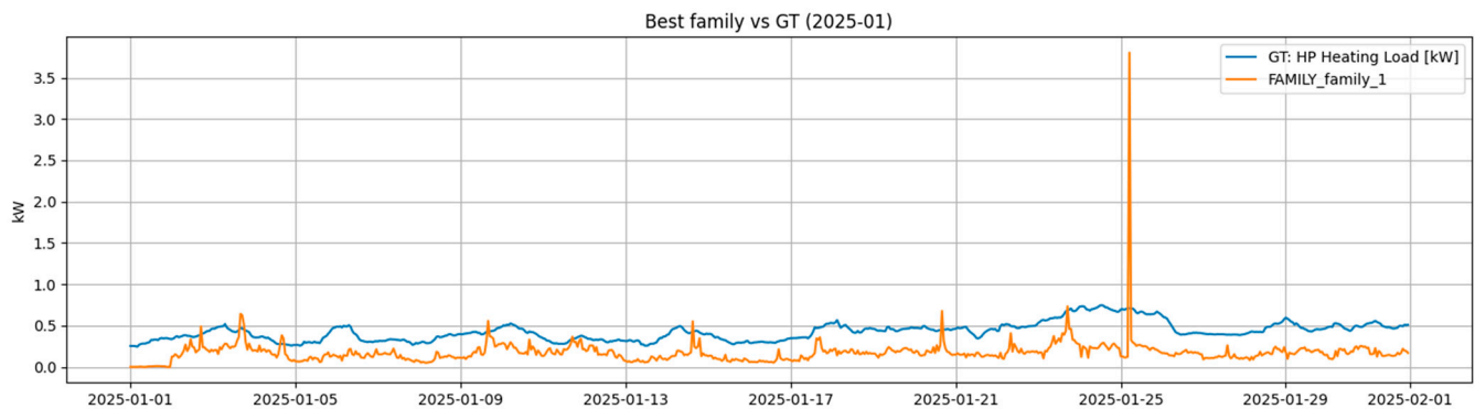
Figure 8. Hourly comparison between the heat-pump-aligned family contribution and the reference heat-pump load.
